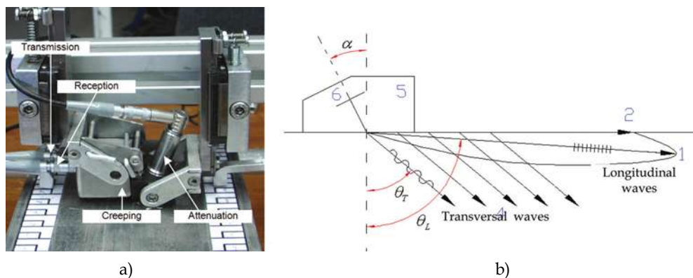
Fig. 17. Inspection of FSW with conventional creeping ultra-sound.
