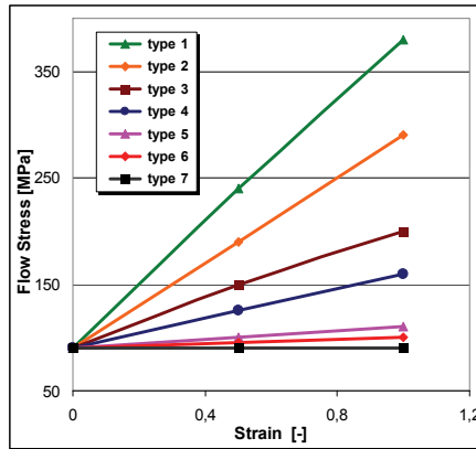
Fig. 9. The \sigma - \varepsilon curves with linear strengthening
