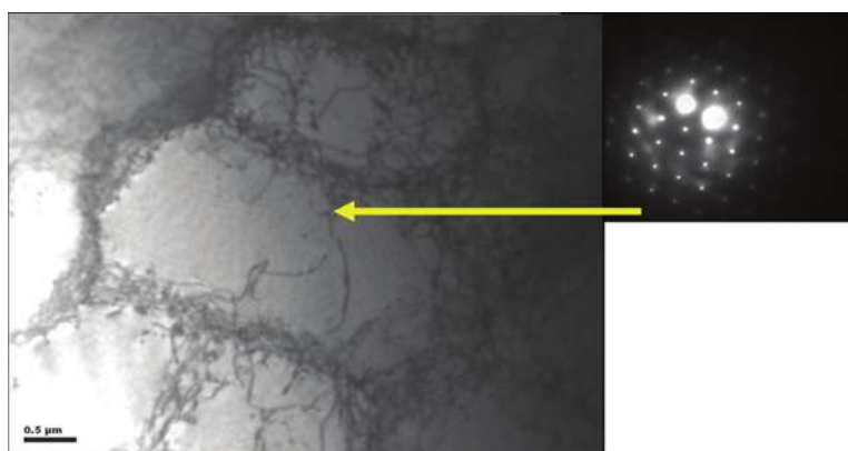
Fig. 18. TEM micrograph after 6 th ECAP pass ( d_{sg} \sim 2,6 \mu m )
