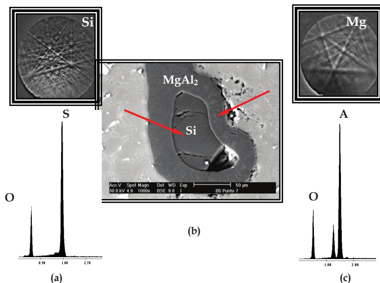
Fig. 11. (a), EDS and EBSD patterns of the nucleus of a SiO 2 particle reacted for 5 minutes at 750 °C in molten aluminium; (b), SEM micrograph of the particle; and (c), EDS and EBSD patterns of MgAl 2 O 4 in the layers of reaction products.
