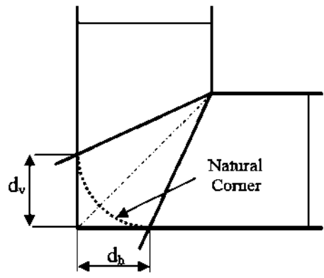
Fig. 6. Geometrical definition of channels
