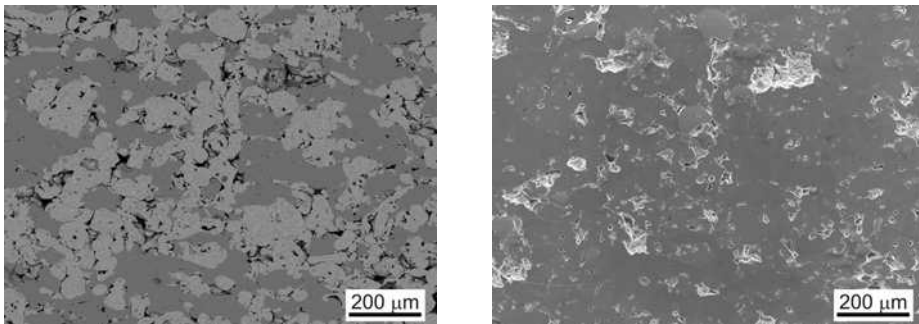
Fig. 12. The typical microstructure for 600 MPa pressed specimens, Al-Zn-Mg-Cu specimens, left SEI and right COMPO
