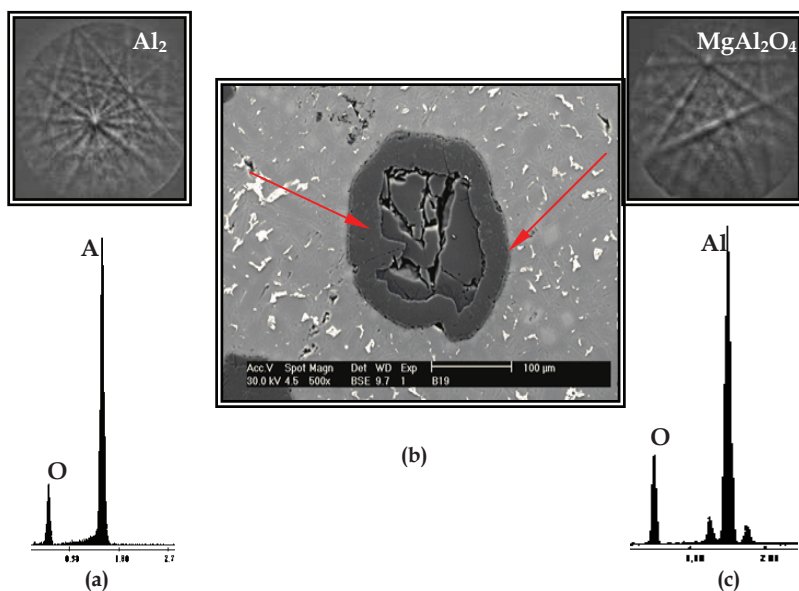
Fig. 12. (a), EDS and EBSD patterns of Al 2 O 3 around the nucleus of a SiO 2 particle reacted for 10 minutes at 750 °C in molten aluminium; (b), SEM micrograph of the particle; and (c), EDS and EBSD patterns of MgAl 2 O 4 in the outer layers of reaction products.
