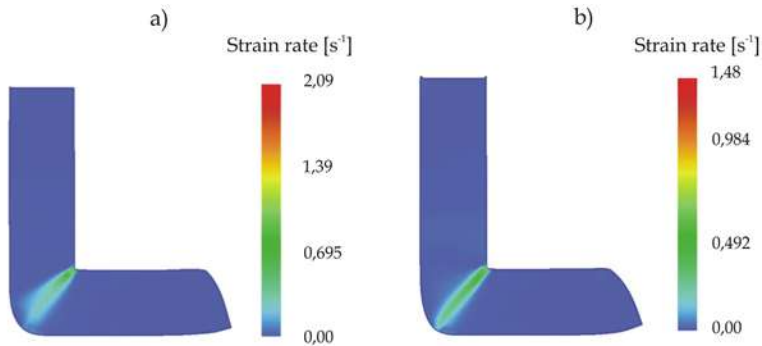
Fig. 31. Distribution of strain rate intensity along to cross-section in 550 th computational step: a) database material, and b) experimental material
