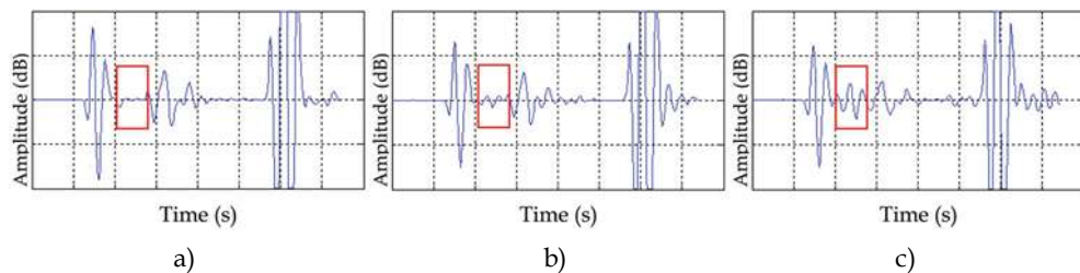
Fig. 20. Results of the NDT ToFD ultra-sound on AA5083-H111.
