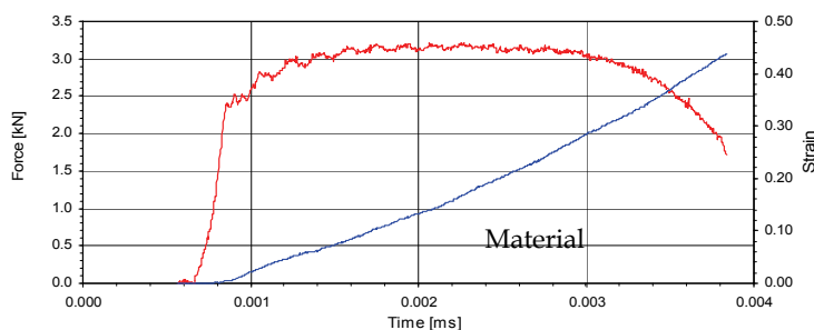
Fig. 9. Load and displacement curve
