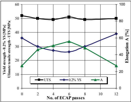
Fig. 14. Development of mechanical properties on ECAP passes
