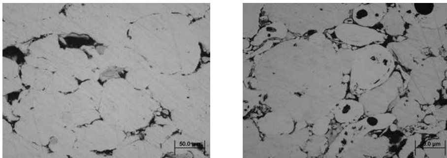
Fig. 5. Microstructure of aluminium alloys at 200 MPa, left - Al-Mg-Si-Cu-Fe, right - Al-Zn-Mg-Cu
