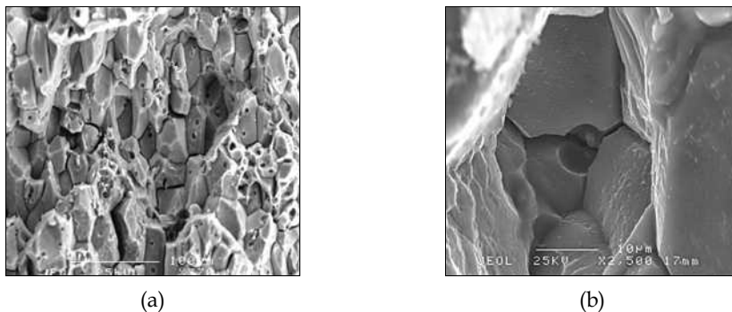
Fig. 12. CFCG fracture surfaces in air (a) intergranular decohesions ( K_{max} = 23 MPa \times m^{1/2} , da/dN = 2 \times 10^{-5} m/cycle , 10s-1500s-10s, 175°C); (b) cavitation at triple grain boundary ( K_{max} = 30 MPa \times m^{1/2} , da/dN = 2 \times 10^{-6} m/cycle , 10s-300s-10s, 175°C).
