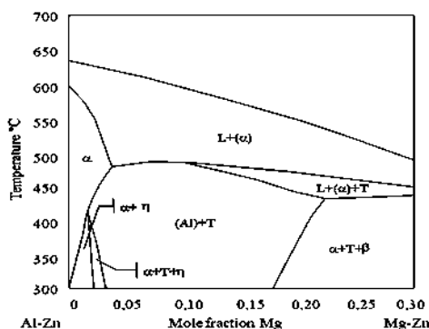
Fig. 2. Isoleth of the Al-5%Zn-Mg alloy
