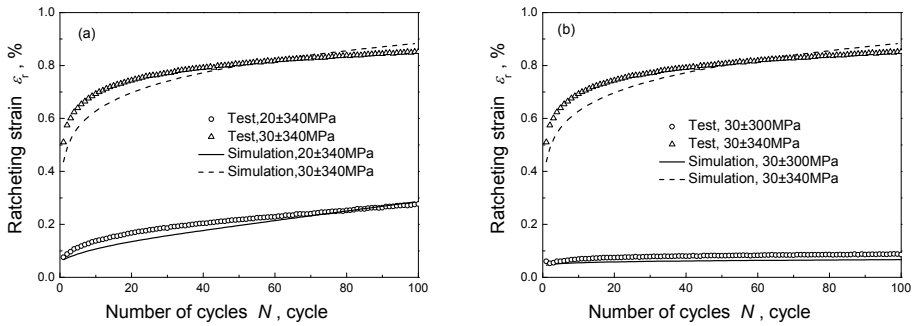
Fig. 14. Experimental and simulated results of uniaxial ratchetting for 6061-T6 aluminium alloy at room temperature (stress rate 100 \text{ MPa} \cdot \text{s}^{-1} ): (a) with different mean stresses; (b) with different stress amplitudes. (Originally from Ding et al. (2010))
