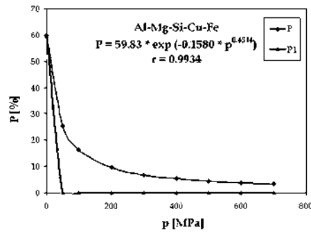
Fig. 2. Compressibility curves of Al-Mg-Si-Cu-Fe aluminium alloy
