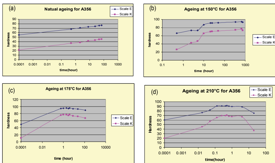
Fig. 4. Hardness changes with time for A356 at (a) Natural ageing; (b) 150^\circ\text{C} ; (c) 175^\circ\text{C} ; (d) 210^\circ\text{C}
