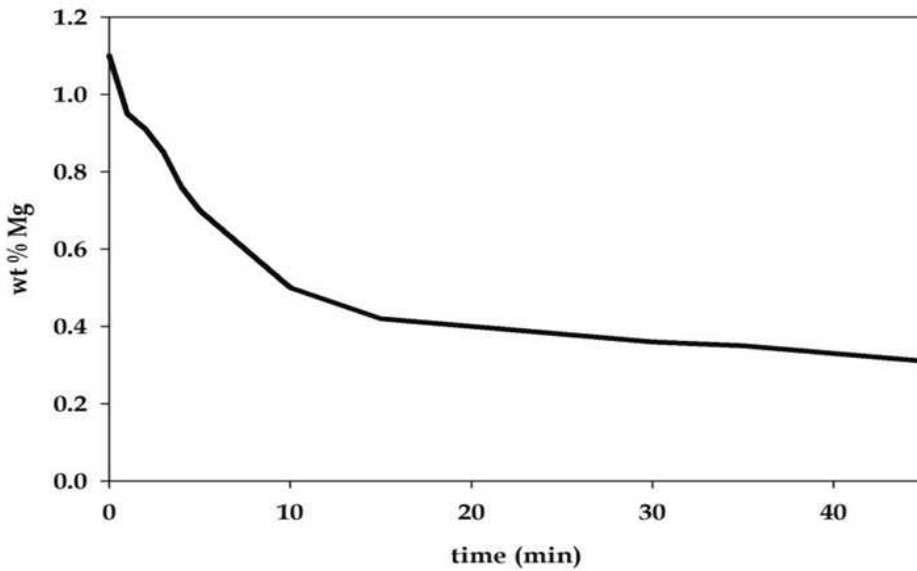
Fig. 10. Variation of Mg concentration as a function of time during \text{SiO}_2 particle addition with mechanical agitation at 750^\circ\text{C} .
