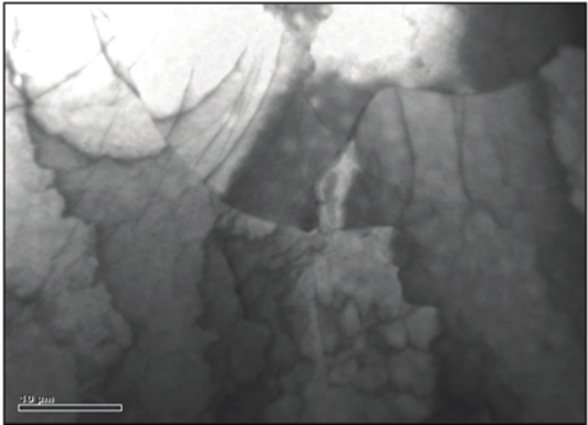
Fig. 16. TEM micrograph before ECAP ( d_g \sim 650 \mu\text{m} )
