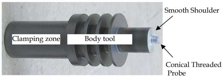
Fig. 2. Conventional FSW mono-bloc tool
