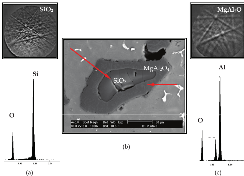
Fig. 8. (a), EDS and EBSD patterns of \text{SiO}_2 particles; (b), SEM micrograph of the particles, and (c), EDS and EBSD patterns of the \text{MgAl}_2\text{O}_4 layer of reaction products. The micrographs correspond to a particle that has been reacting in the molten bath for 1 minute at 750 °C.
