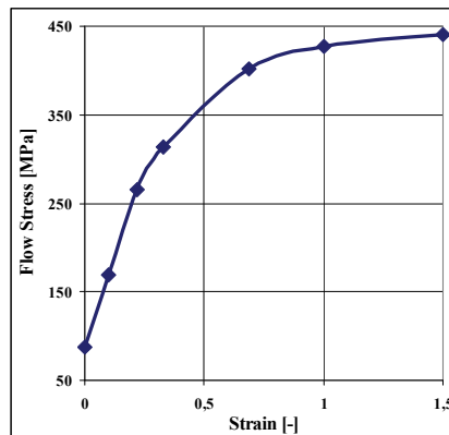
Fig. 3. Stress-strain curve of Al material
