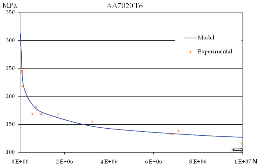
Fig. 10. Fatigue curve of the AA7020 T6
