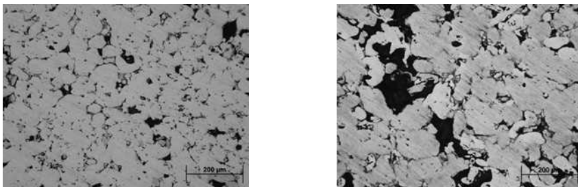
Fig. 4. Microstructure of aluminium alloys at 50 MPa, left - Al-Mg-Si-Cu-Fe, right - Al-Zn-Mg-Cu
