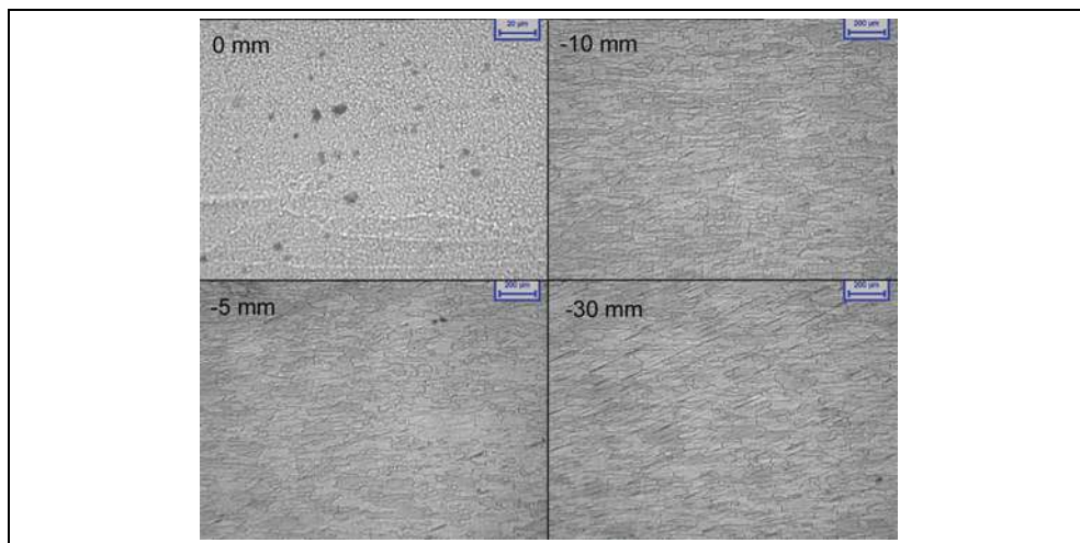
Fig. 10. Microstructure of different parts of a 6013-6013 weld.
