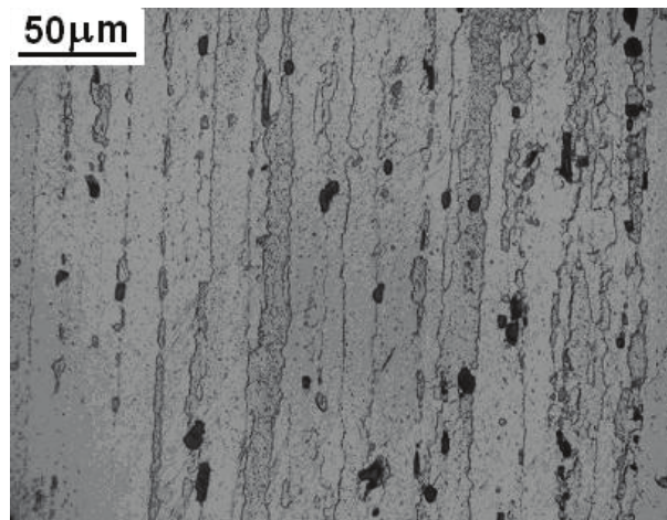
Fig. 1. Microstructure of AlCu4Mg1 aluminium alloy, magnification 500x
