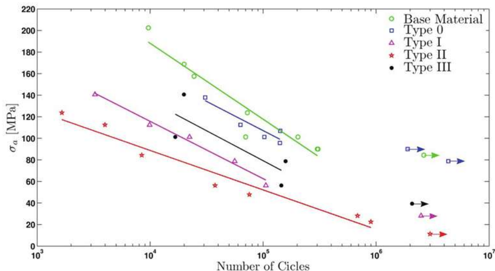
Fig. 13. Fatigue curves for base material and 4 different defect type conditions
