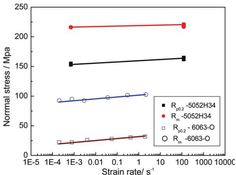
Fig. 13. Relationship between strength and strain rate
