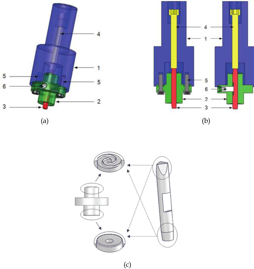
Fig. 3. Modular dual FSW tool. a) 3D view of assembly, b) Cutaway view in two perpendicular planes, c) Detail of geometric duality of the dual basis and probe dual. Nomenclature: main body (1), dual shoulder (2), dual-probe (3), vertical adjustment screw (4), bolts of the dual basis (5), dual screw probe (6).
