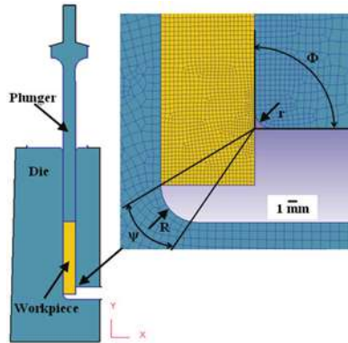
Fig. 2. FEM simulation scheme of ECAP
