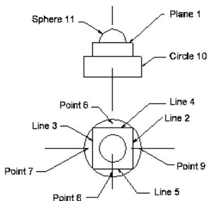
Fig. 4. Geometrical elements measured on workpieces and electrodes
