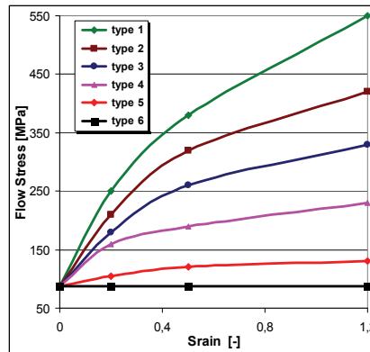
Fig. 10. The \sigma - \varepsilon curves with nonlinear strengthening
