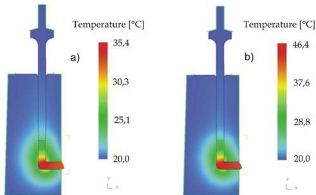
Fig. 32. Temperature development during ECAP process and heating of forming tools: a) database material, and b) experimental material
