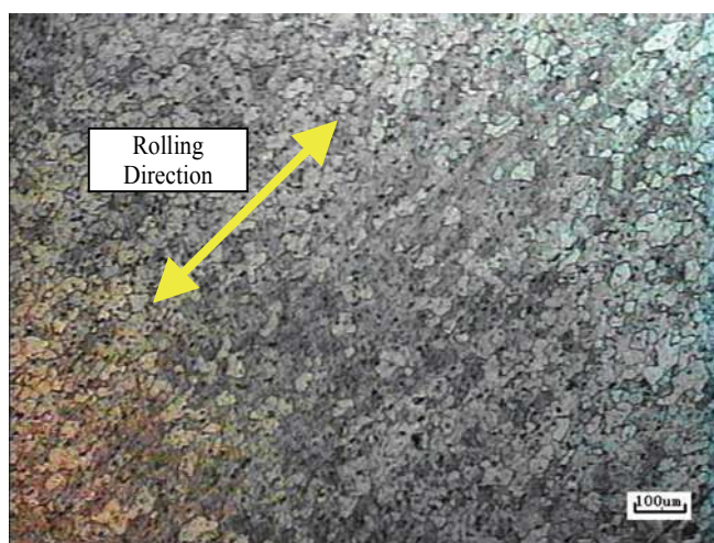
Fig. 6. Microstructure of rolling plate 5052H34
