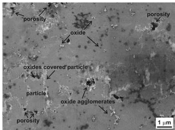
Fig. 10. Oxide layer covering aluminium particles
