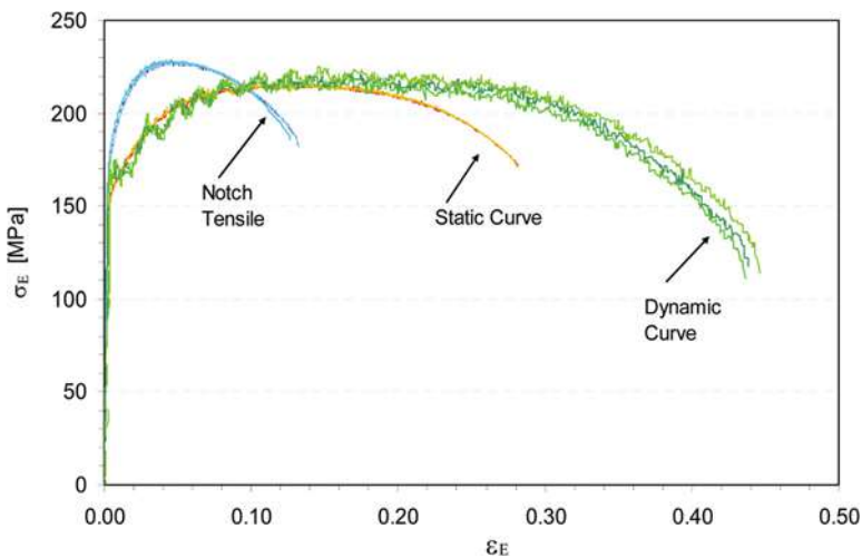
Fig. 12. Effects of stress state and strain rate on material flow property
