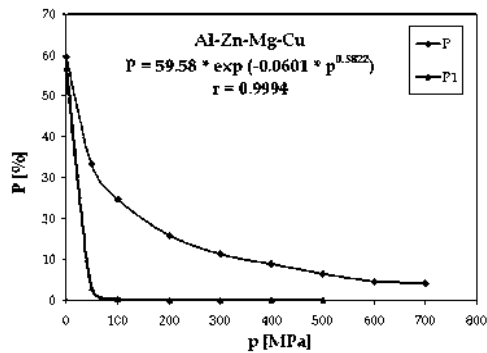
Fig. 3. Compressibility curves of Al-Zn-Mg-Cu alloy
