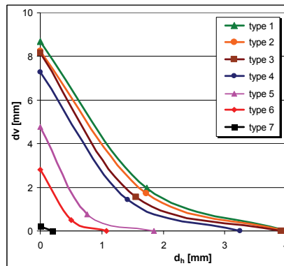
Fig. 11. Effect of \sigma - \varepsilon curves with linear strengthening on the channel outer filling
