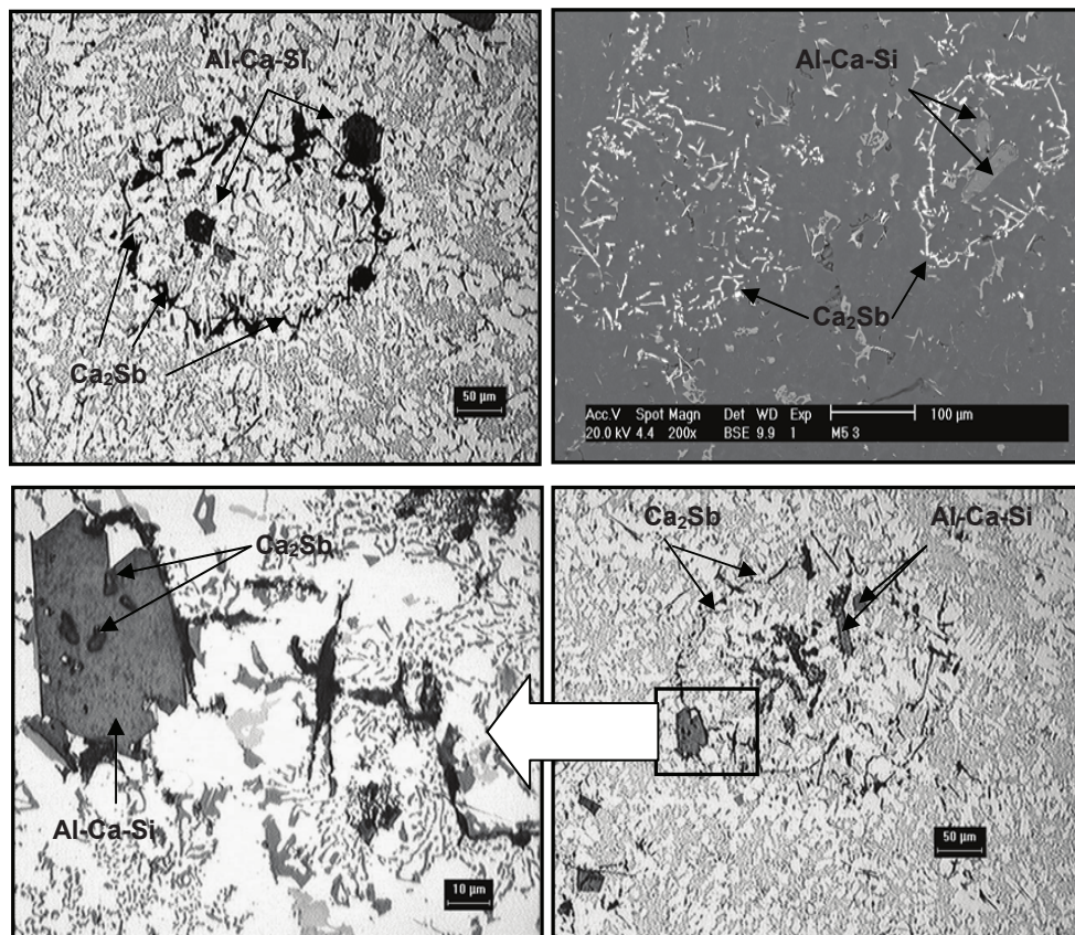
Fig. 7. Microstructural features of AlCaSi and CaSb particles after calcium addition to AlSi alloys.
