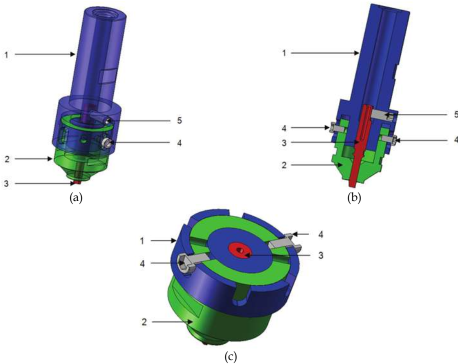
Fig. 4. Modular dual FSW tool with forced cooling.
