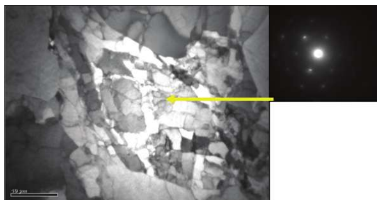
Fig. 19. TEM micrograph after 8 th ECAP pass ( d_{sg} \sim 2,6 \mu m )
