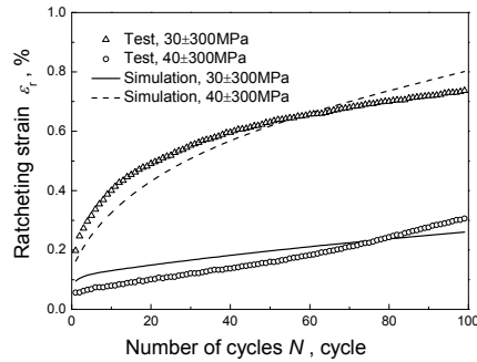
Fig. 15. Experimental and simulated results of uniaxial ratchetting for 6061-T6 aluminium alloy at 150^\circ\text{C} and with different mean stresses (stress rate 100 \text{ MPa} \cdot \text{s}^{-1} ). (Originally from Ding et al. (2010))
