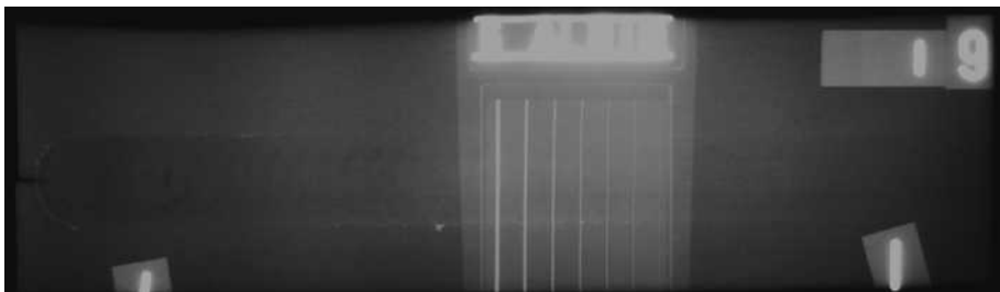
Fig. 15. X-ray image of specimens produced on AA2024-T4 with roots defects Type II
