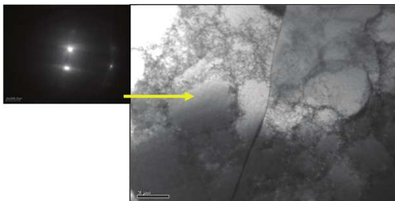
Fig. 17. TEM micrograph after 4 th ECAP pass ( d_{sg} \sim 2,6 \mu m )
