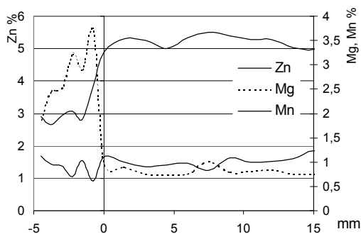
Fig. 12. EDX analysis of welded joint.
