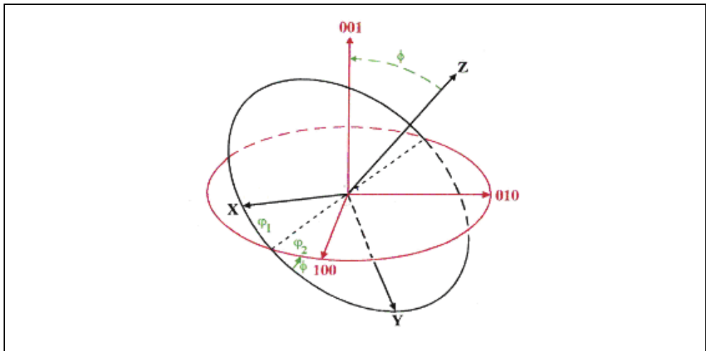
Fig. 3. Definition of the Euler angles.
