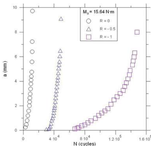
Fig. 8. Fatigue crack length versus number of cycles under bending
