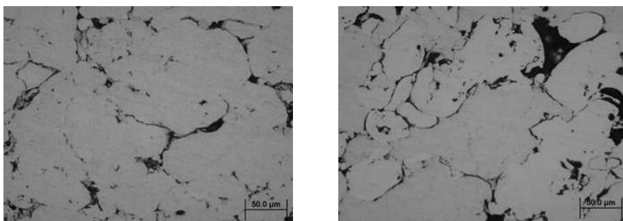
Fig. 6. Microstructure of aluminium alloys at 400 MPa, left - Al-Mg-Si-Cu-Fe, right - Al-Zn-Mg-Cu
