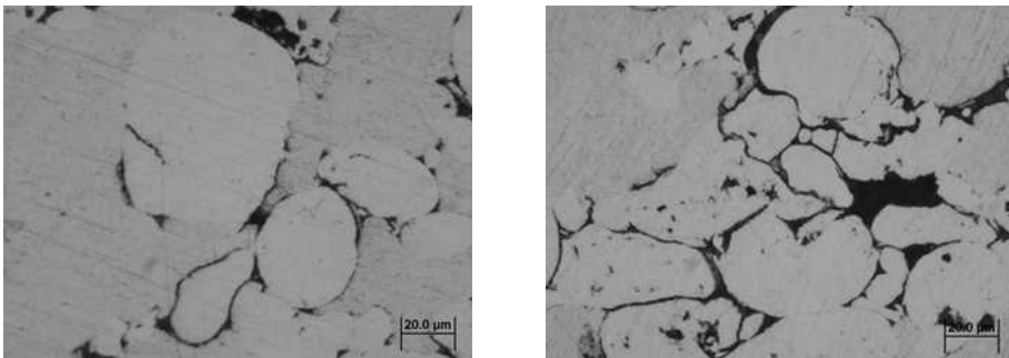
Fig. 9. Microstructure of aluminium alloys at 600 MPa, left, and 700 MPa, right - Al-Zn-Mg-Cu aluminium alloy
