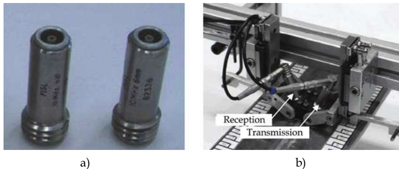
Fig. 19. ToFD ultra-sound NDT testing of AA5083-H111.
