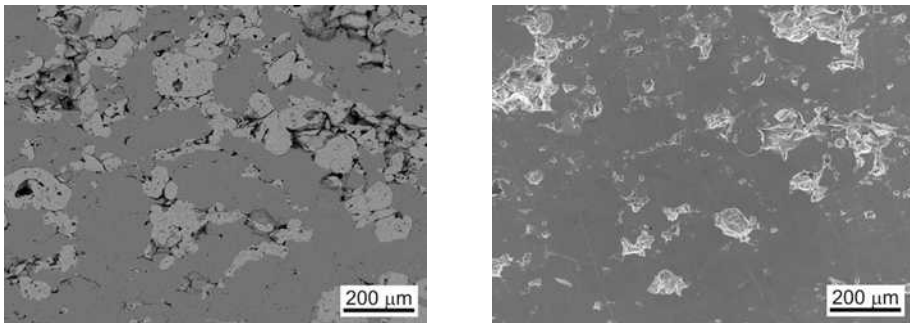
Fig. 11. The typical microstructure for 400 MPa pressed specimens, Al-Zn-Mg-Cu specimens, left SEI and right COMPO
