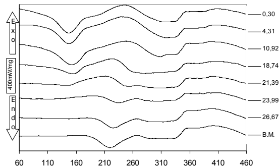
Fig. 14. DSC through a welded joint HAZ.
