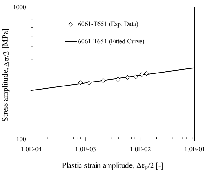
Fig. 5. Cyclic curve of the 6061-T651 aluminium alloy
