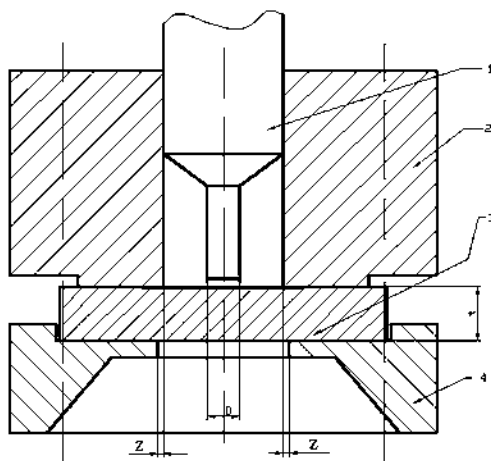
Fig. 19. Experimental setup of the STP
