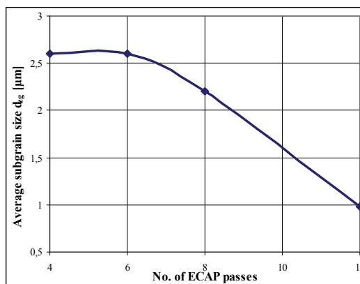
Fig. 21. Grain size change on ECAP passes
