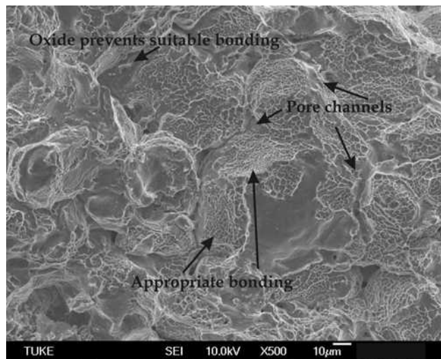
Fig. 13. Consolidation of aluminium alloys by sintering
