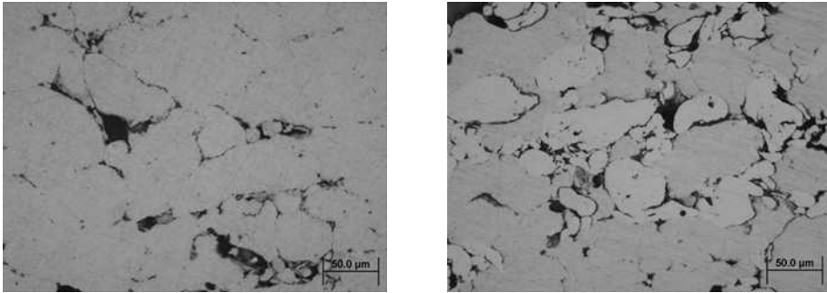
Fig. 7. Microstructure of aluminium alloys at 600 MPa, left - Al-Mg-Si-Cu-Fe, right - Al-Zn-Mg-Cu
