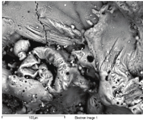
Fig. 18. Detail of Al7075 after roughing
