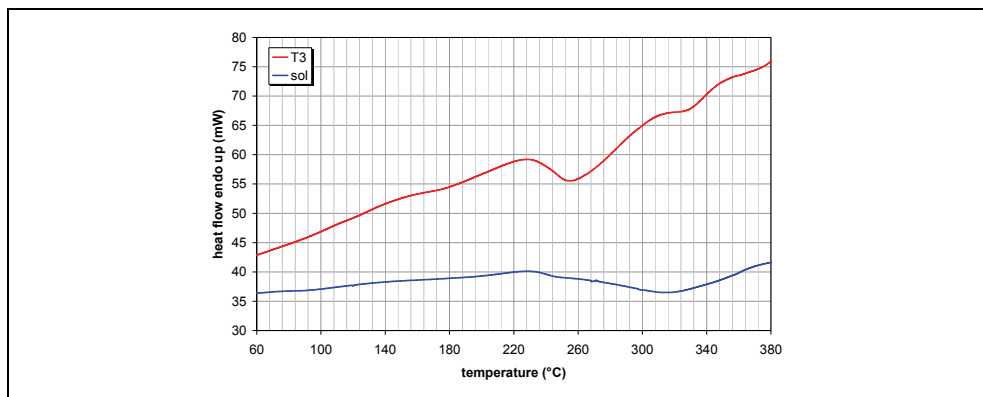
Fig. 14. DSC curves for 2198 alloy.
