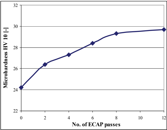
Fig. 15. Microhardness change on ECAP passes
