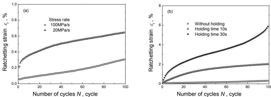
Fig. 8. Time-dependent ratchetting of the alloy at 150°C ( 30\pm300\text{MPa} ): (a) at two stress rates; (b) with or without peak stress hold. (Originally from Ding et al. (2007))
