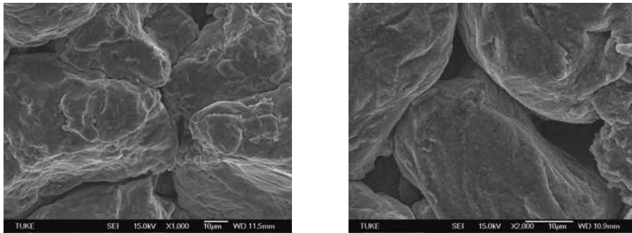
Fig. 8. Microstructure of aluminium alloys at 600 MPa, left - Al-Mg-Si-Cu-Fe, right - Al-Zn-Mg-Cu
