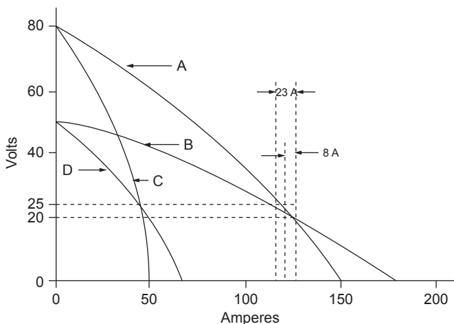
FIGURE 2-3-6 Volt-ampere characteristics of a drooping slope power source with adjustable open circuit voltage.
