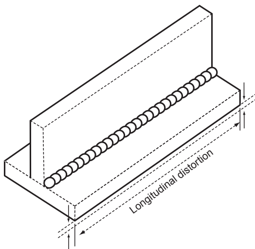
FIGURE 2-5-3 Longitudinal stress and distortions in weld.
