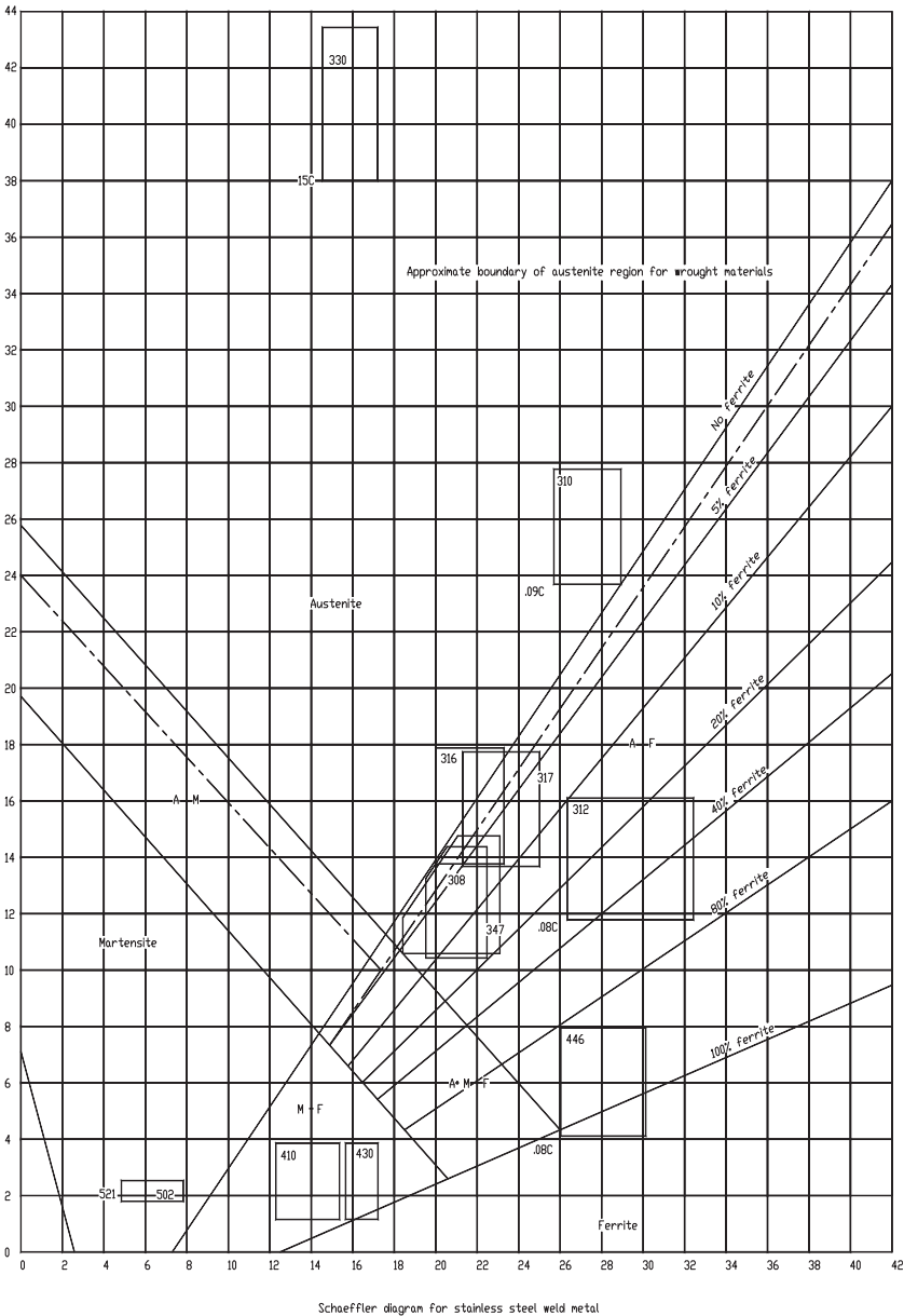
FIGURE 2-6-1 Schaeffler diagram.
