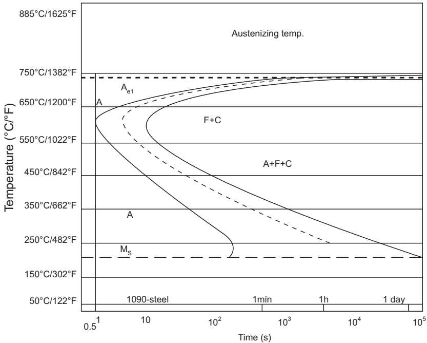
FIGURE 1-12-2 Time temperature transformation diagram of 1090 steel.
