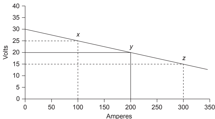
FIGURE 2-3-5 Volt-ampere output relationship for constant voltage power source.
