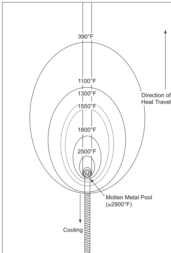
FIGURE 2-4-1 Temperature distributions in a plate.
