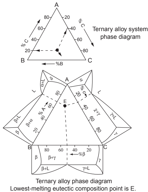
FIGURE 1-4-3 Ternary diagrams.
