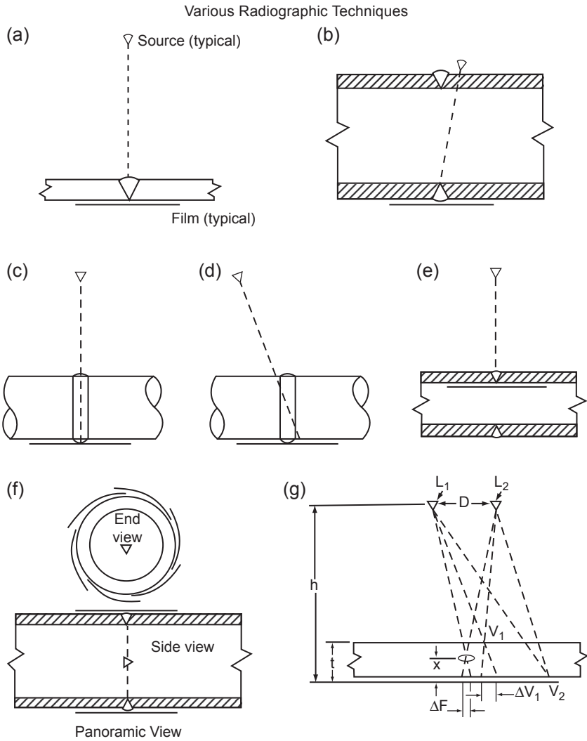
FIGURE 3-3-5 Radiographic techniques.
