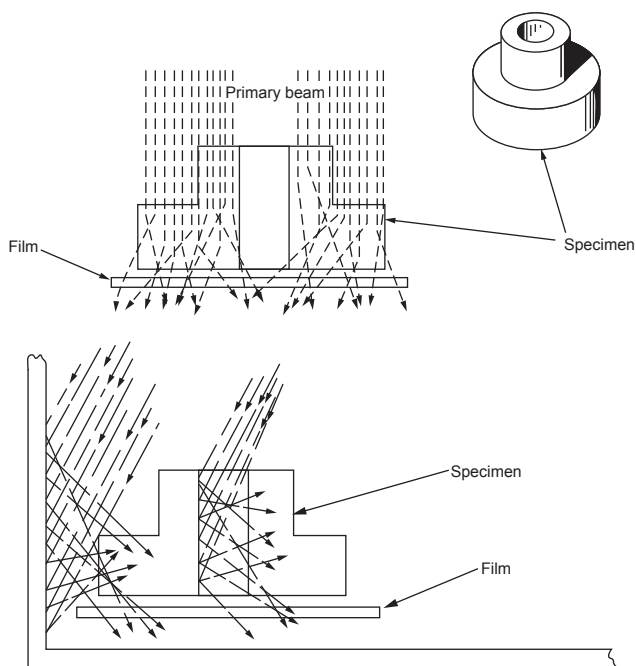
FIGURE 3-3-2 Radiation scatter.
