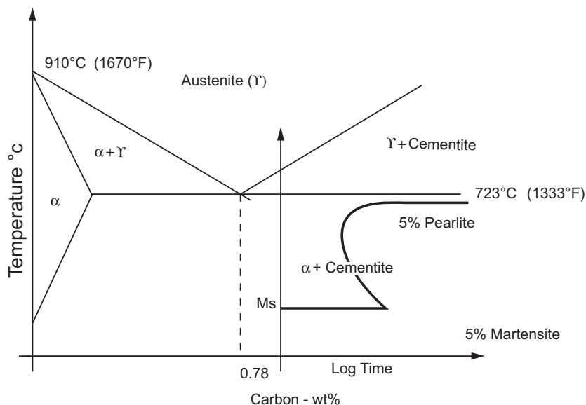
FIGURE 1-12-1 Time temperature transformation curve of eutectoid steel superimposed on an iron carbon phase diagram.
