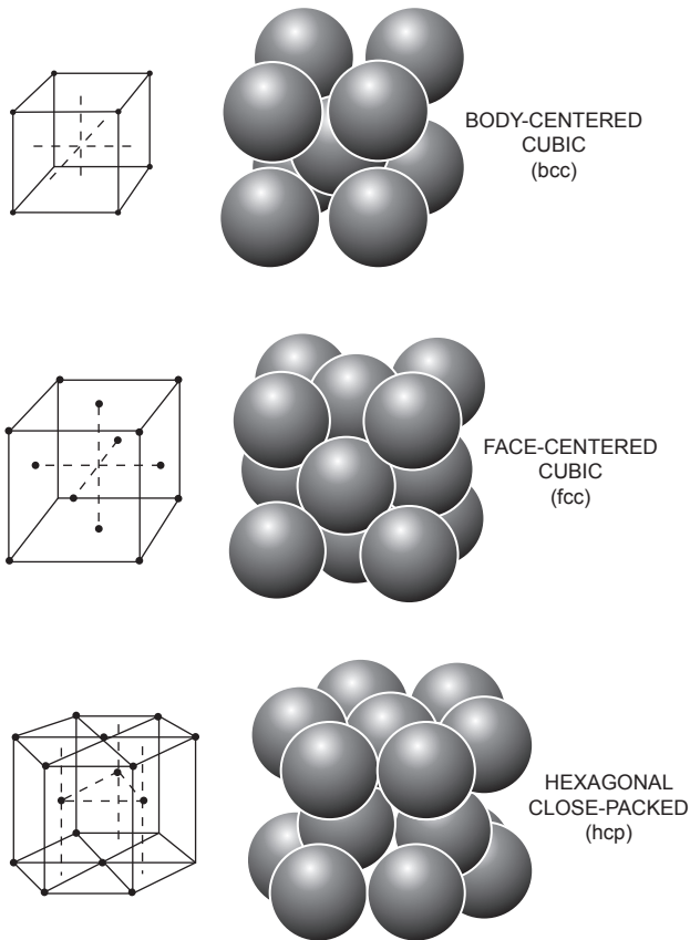
FIGURE 1-3-1 Crystal Lattices.
