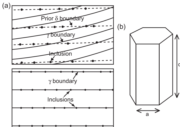
FIGURE 1-3-3 (a) Location of large inclusions for solidification as \delta ferrite and as austenite. (b) A hexagonal prism model for the columnar austenite grains typical of the microstructure of steel weld metals.
