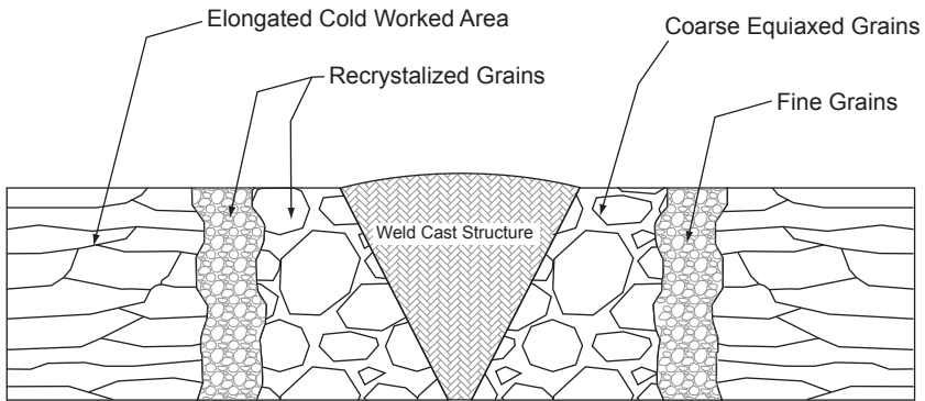
FIGURE 2-5-1 Stresses in weld.
