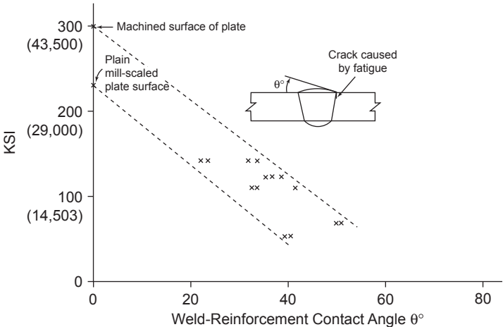
FIGURE 2-5-5 Effect of weld reinforcement contact angle on fatigue strength of weldments.
