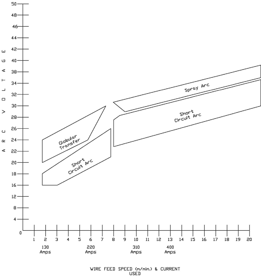
FIGURE 2-3-3 Metal transfer in the short circuit gas metal arc welding process.
