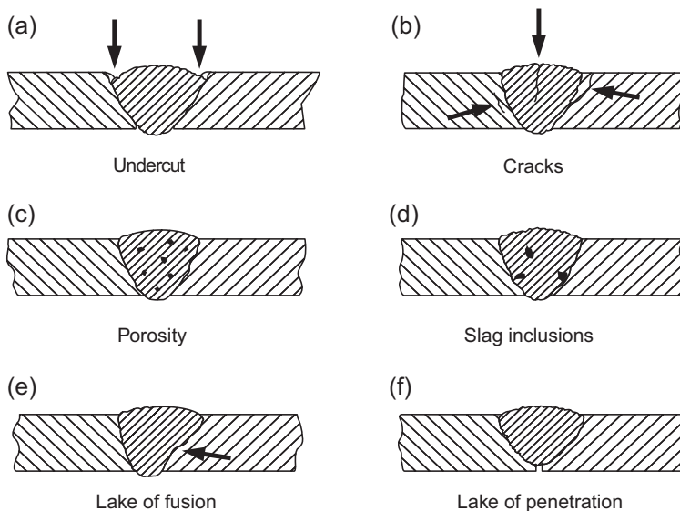
FIGURE 2-8-1 Typical weld defects.
