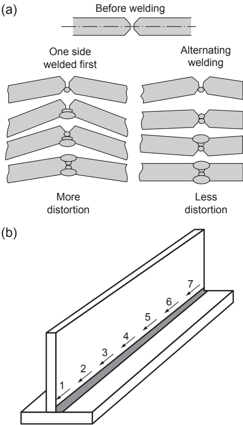
FIGURE 2-5-4 Controlling distortion by welding.
