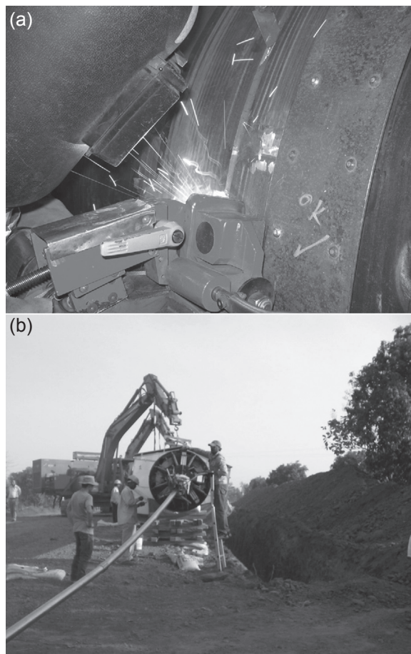
FIGURE 2-3-4 (a) Mechanized welding being performed, (b) Mechanized welding of 48 inch diameter pipe.
