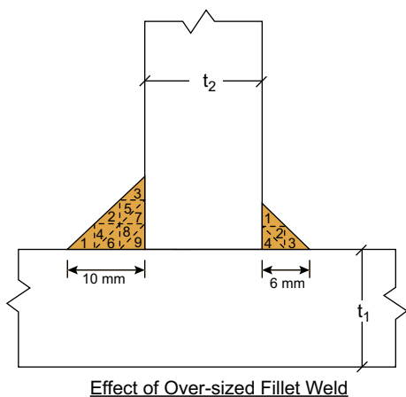
FIGURE 2-5-6 Effect of over-sized weld. Note the number of equal area triangles in each comparisons above.
