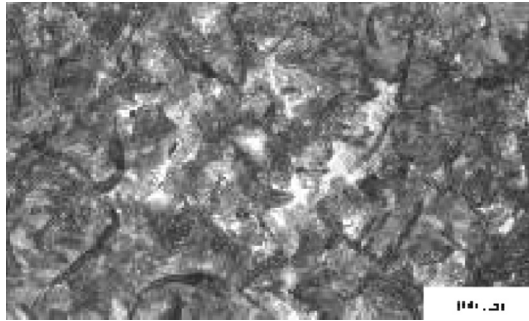
FIGURE 1-7-1 Grey cast iron, Fe 3.2%C and Si 2.5% by weight, containing graphite flakes in a matrix, which is pearlitic. The speckled white regions represent a phosphide eutectic. (Courtesy of Bombay Malleable, Andheri-Kurla Road, Bombay, 1983.)
