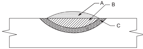
FIGURE 2-2-1 Dilution of material and heat in the weld nugget.
