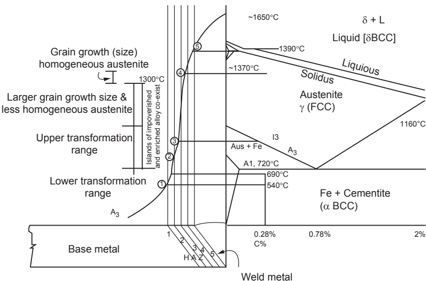
FIGURE 2-4-2 Temperature distributions in weldments superimposed on a phase diagram.
