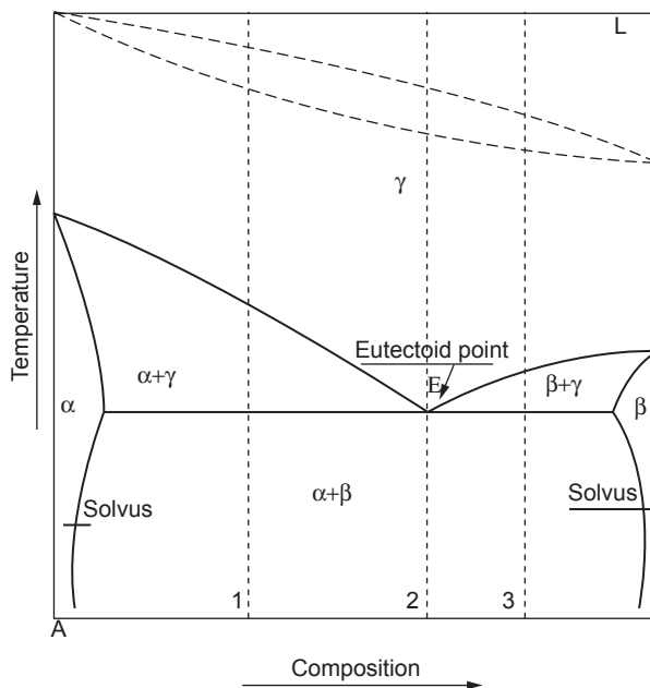
FIGURE 1-4-2 Binary diagram of a eutectoid system.
