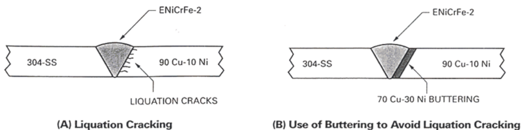
Figure 2.4 Liquation cracking may be avoided by buttering with an intermediate melting temperature weld metal [Ref. 3]
