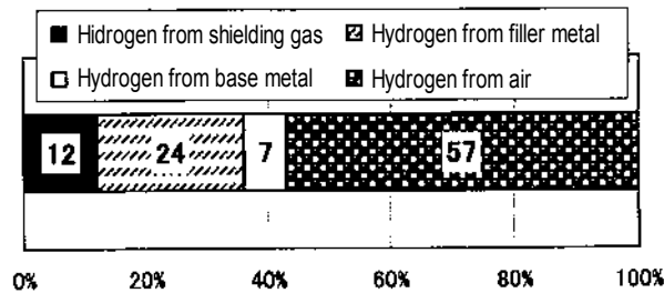
Figure 3.11 Ratios of sources of the hydrogen invaded into the arc atmosphere [Ref. 8]
