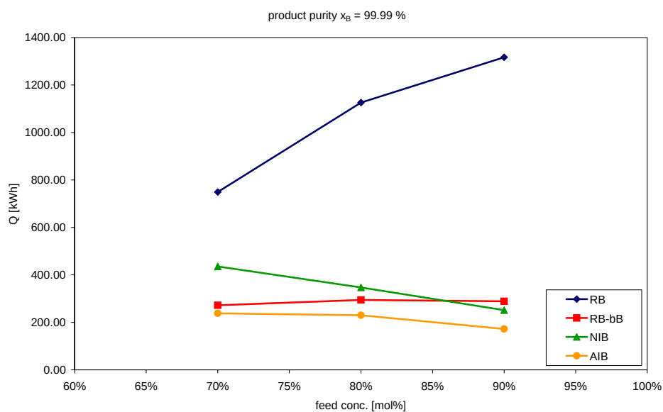
Fig. 6.35 Comparison concerning the energy consumption for different structures (RB-bB4x, NIB4x, AIB4x): high pressure, product purity 99,99 mol% water, feed conc. 70 mol%, 80 mol%, 90 mol% ACN.
