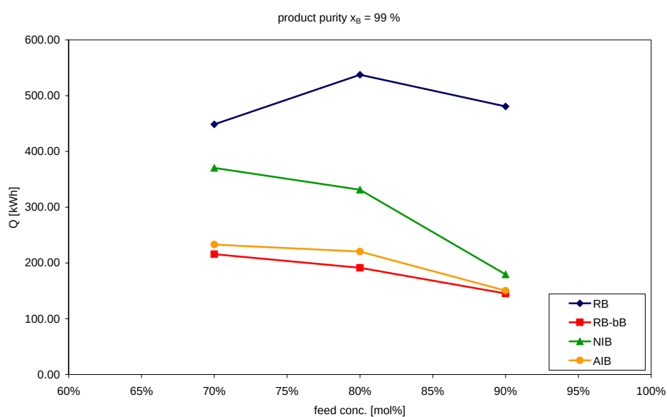
Fig. A.14 Comparison concerning the energy consumption for different structures (RB, RB-bB, NIB, AIB): high pressure, product purity 99 mol% water, feed conc. 70 mol%, 80 mol%, 90 mol% ACN.
