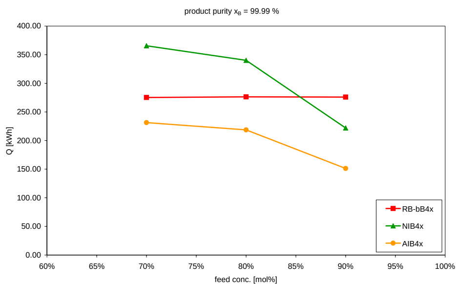
Fig. A.32 Comparison concerning the energy consumption for different structures (RB-bB4x, NIB4x, AIB4x): high pressure, product purity 99,99 mol% water, feed conc. 70 mol%, 80 mol%, 90 mol% ACN.
