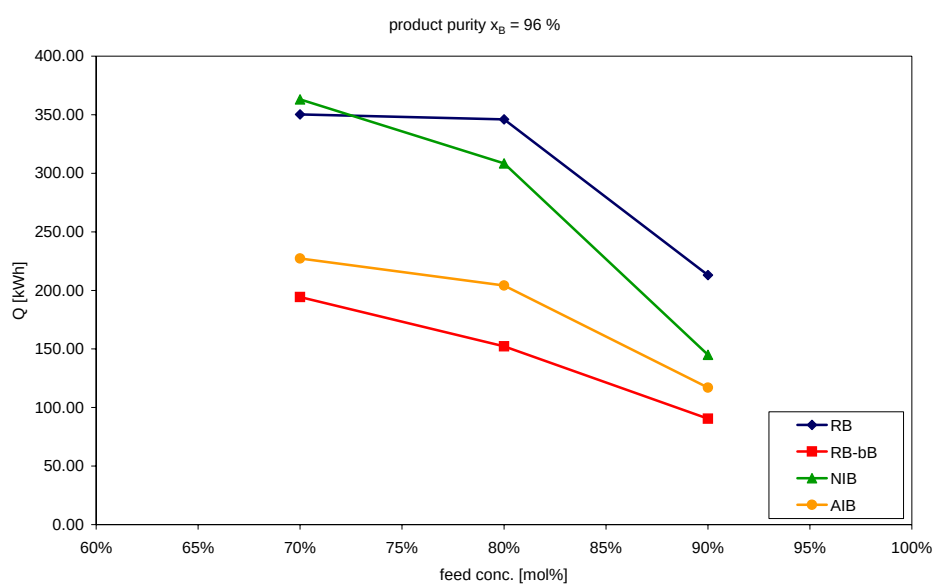
Fig. A.13 Comparison concerning the energy consumption for different structures (RB, RB-bB, NIB, AIB): high pressure, product purity 96 mol% water, feed conc. 70 mol%, 80 mol%, 90 mol% ACN.
