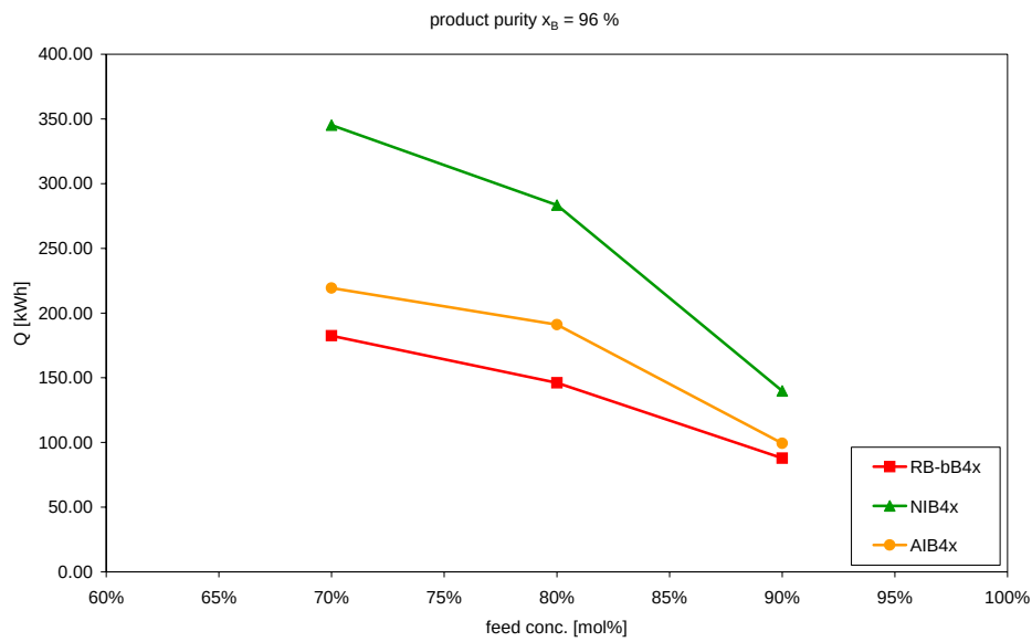
Fig. A.29 Comparison concerning the energy consumption for different structures (RB-bB4x, NIB4x, AIB4x): high pressure, product purity 96 mol% water, feed conc. 70 mol%, 80 mol%, 90 mol% ACN.
