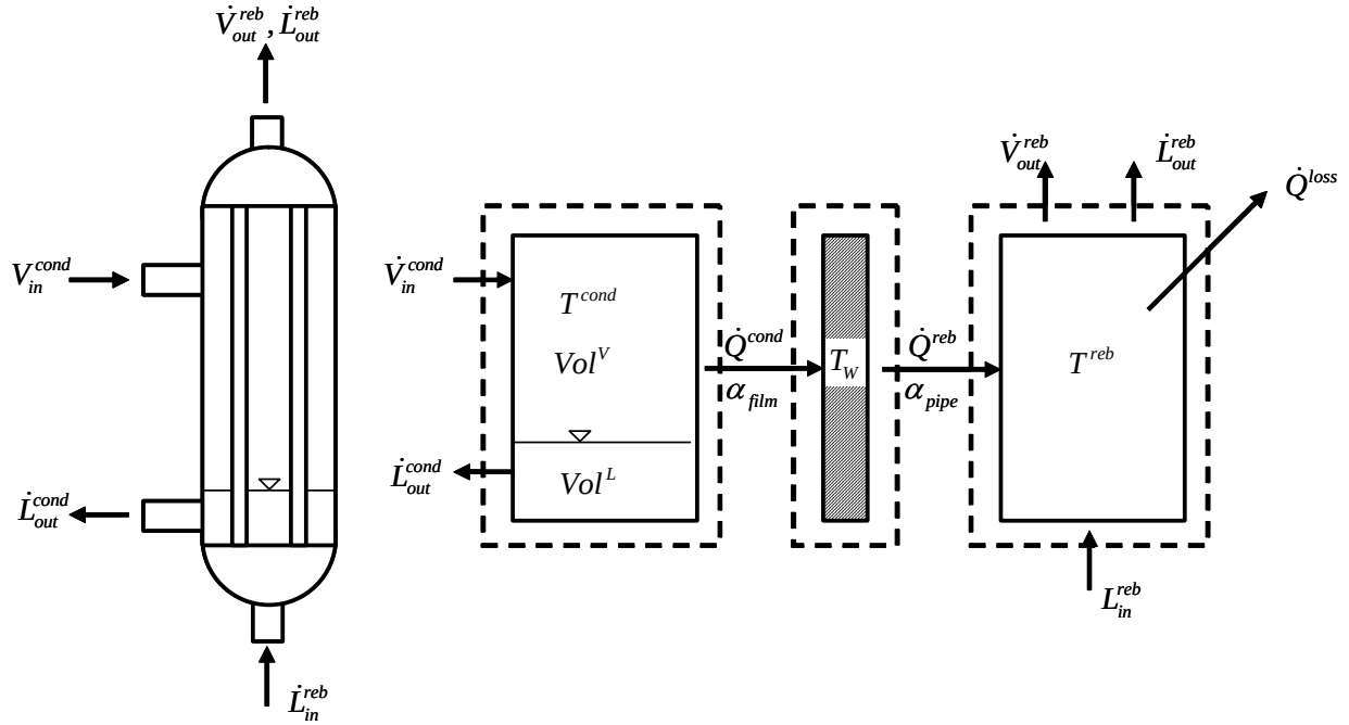
Fig. 3.14 Balance regions for the coupled heat exchanger.
