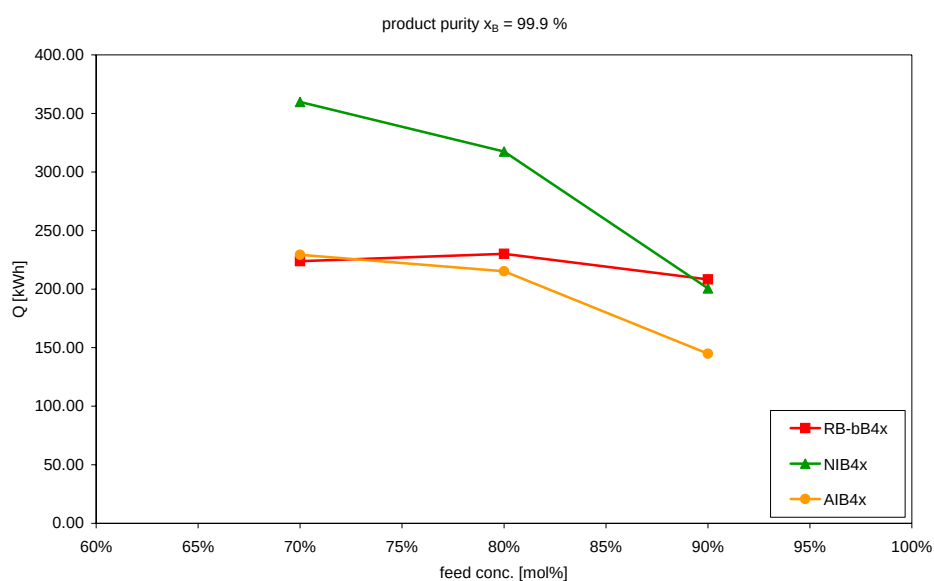
Fig. A.31 Comparison concerning the energy consumption for different structures (RB-bB4x, NIB4x, AIB4x): high pressure, product purity 99,9 mol% water, feed conc. 70 mol%, 80 mol%, 90 mol% ACN.
