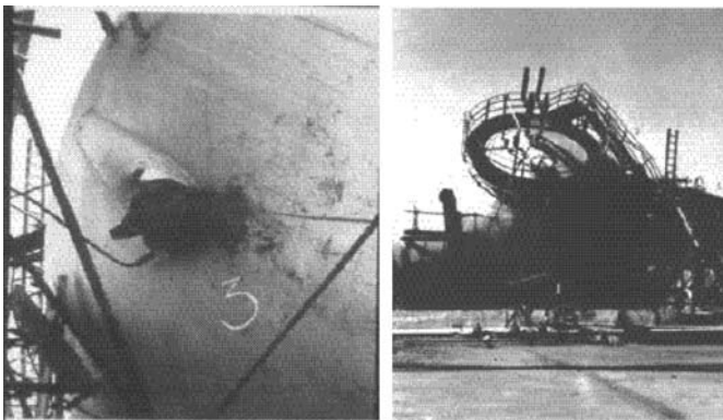
Collapsed LPG sphere supports in 1972
