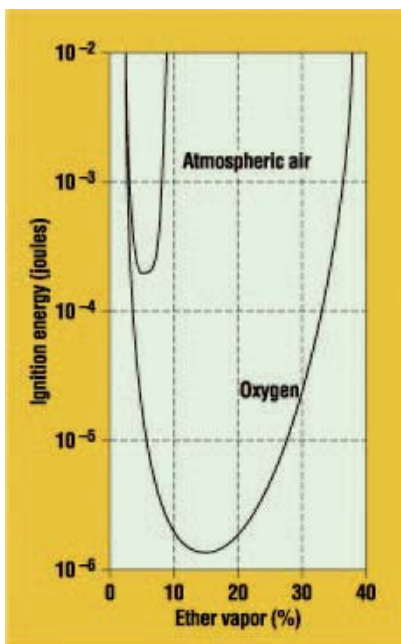
Figure 46 Ignition energies for diethyl vapour in air and oxygen.
