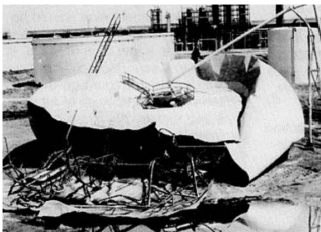
Figure 40 Spheroid ruptured by low-grade explosion. Although this tank appears to have been damaged by vacuum, it was established by examination that the vacuum damage occurred due to the outrush of water after the explosion had ruptured the tank. Note the unbuckled condition of the supporting truss in the centre of the area which was pushed out.
