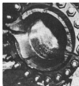
Figures 30 and 31 A mixture of lube-oil mist and air in the suction piping of a centrifugal compressor operating in a test loop detonated. The detonation progressed upstream to the normal flow. Suction piping was ruptured in two locations, and internal damage occurred in the compressor and in a cooler. The building was wrecked (Figure 32), and other parts of the test facility were badly damaged (Figures 30 and 31). Ignition probably was induced by friction in the compressor.
