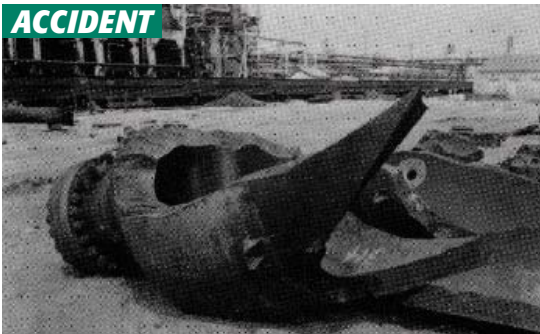
Figure 21 Three vertical drums—4'4" ID344' long with 5-1/2" wall thickness fragmented.
