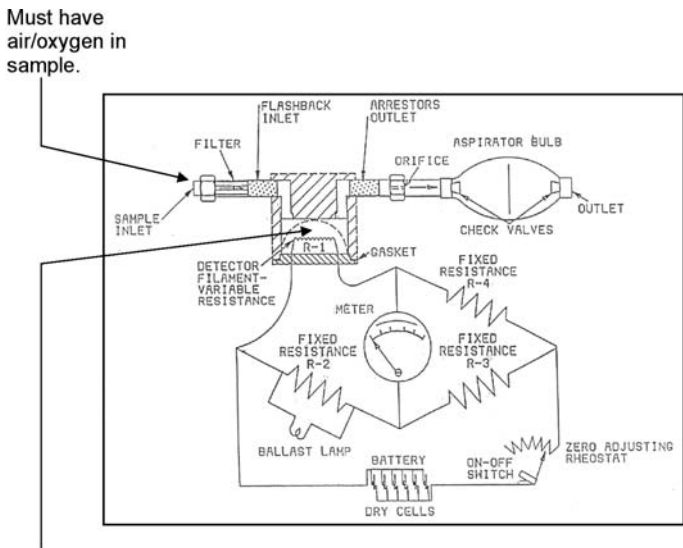
Figure 9 Working principle of an catalytic explosimeter.
