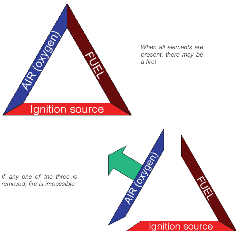
Figure 2 The fire triangle. A fire or explosion can occur only when all three sides of the triangle are present.
