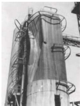
Figure 9a Too much vacuum damaged this catalyst storage drum.
