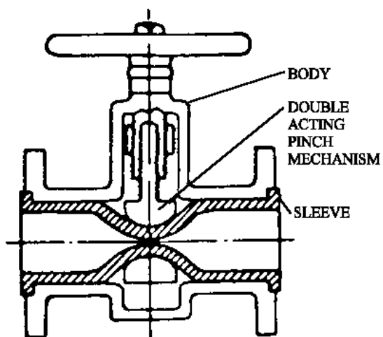
PINCH
