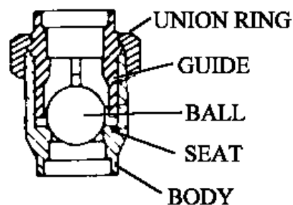
LIFT (BALL-VERTICAL)
