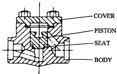
LIFT (PISTON)
