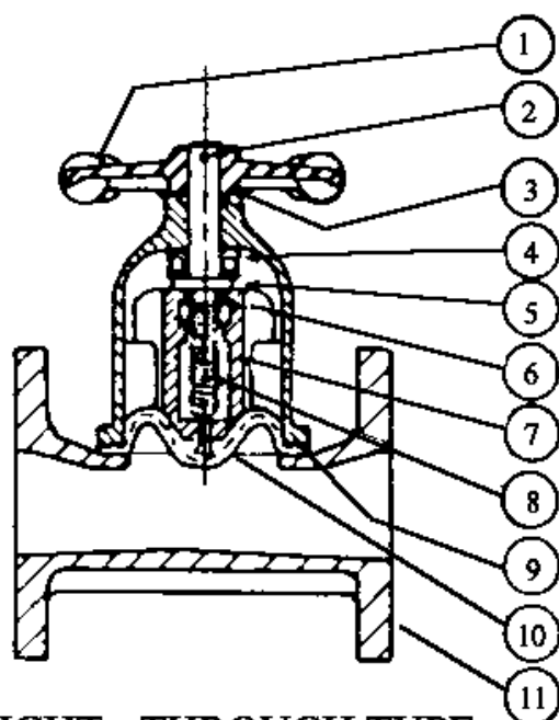
STRAIGHT - THROUGH TYPE
