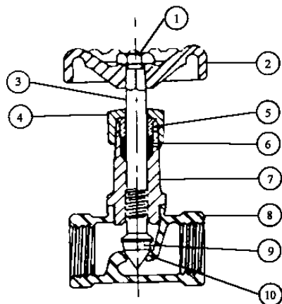
GLOBE ( NEEDLE TYPE DISK )
