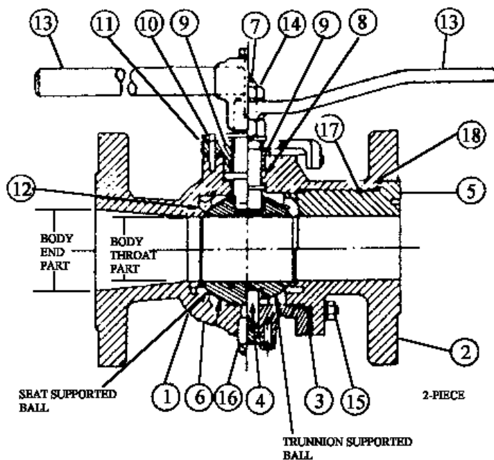
SPLIT BODY (END ENTRY)
