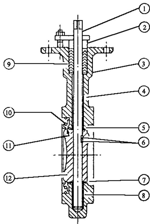
TYPICAL ASSEMBLY HIGH PERFORMANCE VALVE
