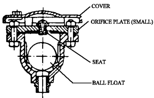
SINGLE VALVE
