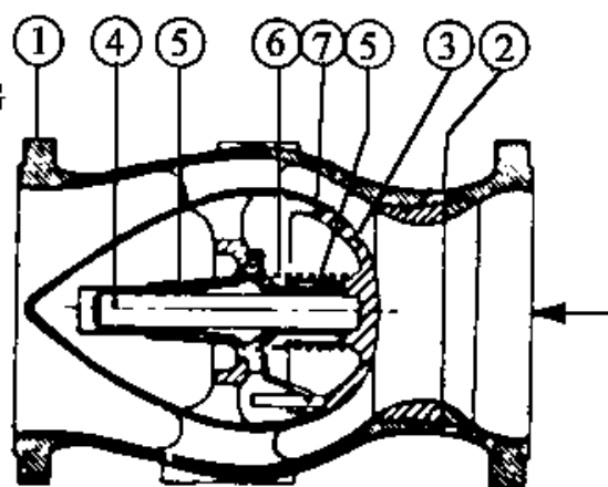
AXIAL FLOW
