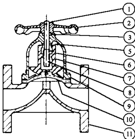
WEIR TYPE
