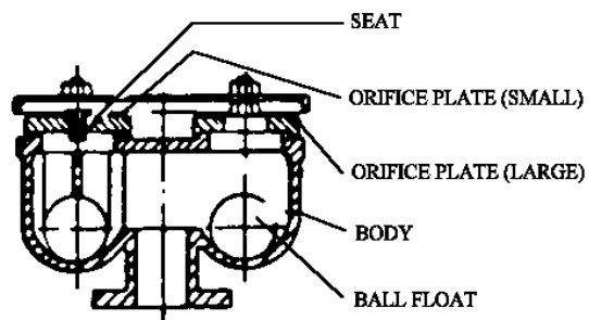
DOUBLE VALVE
