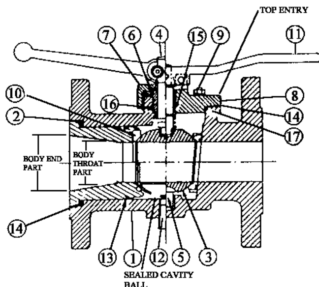
ONE PIECE BODY (END OR TOP ENTRY)
