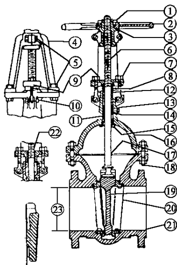
WEDGE GATE
