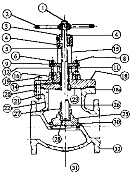
GLOBE ( PLUG TYPE DISK )
