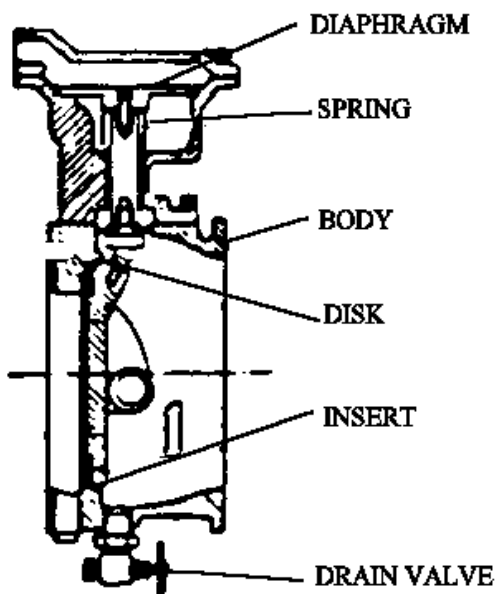
DELUGE VALVE
