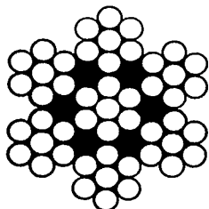
6 x 7 (6/1) WSC (sometimes referred to as 7 x 7)
