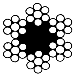
Round strand 6 x 7 (6/1) Fibre core
