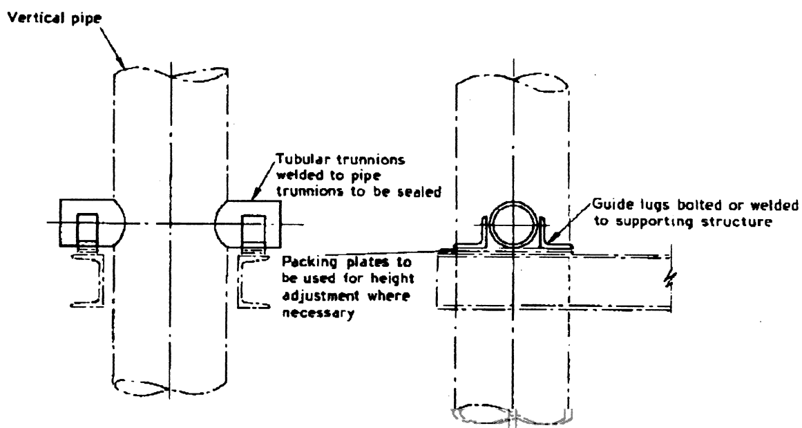
Figure 41 — Trunnion support for uninsulated vertical pipes
