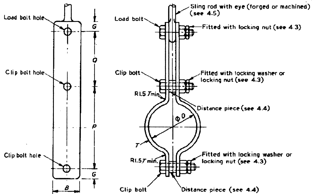
Figure 9 — Pipe clip for steel pipes, Range C: above 400 °C to 470 °C
