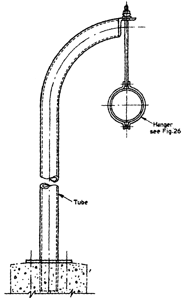
Figure 27 — Tubular support for a single pipe
