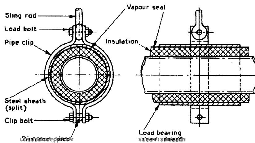
Figure 39 — Hanger for insulated cold pipes
