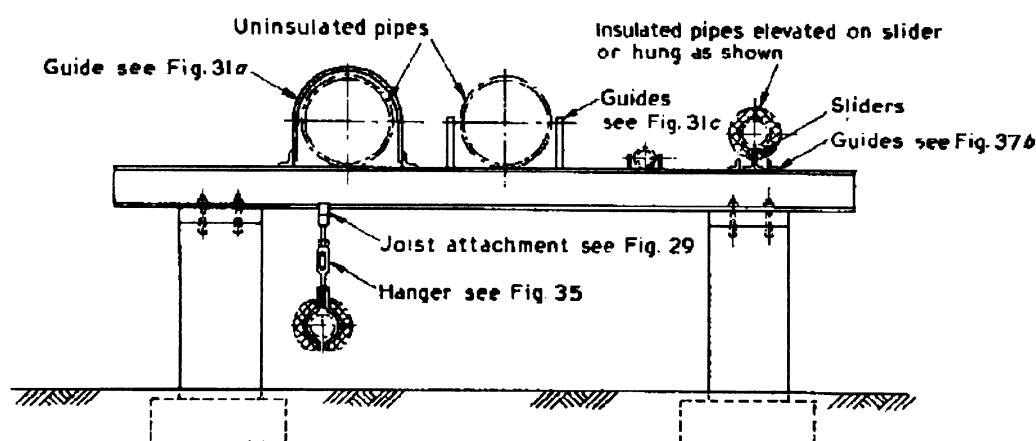
Figure 21 — Low-level trestle for multiple pipes
