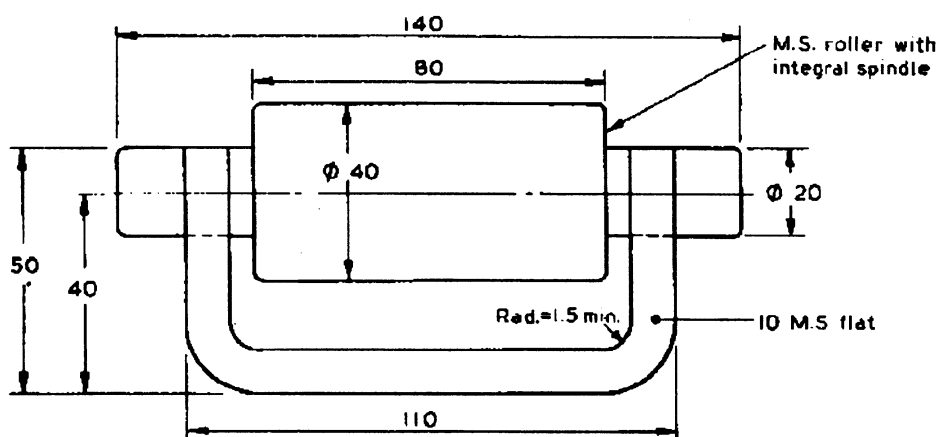
Figure 20 — Roller type support with mild steel roller and chair formed from rolled steel flat
