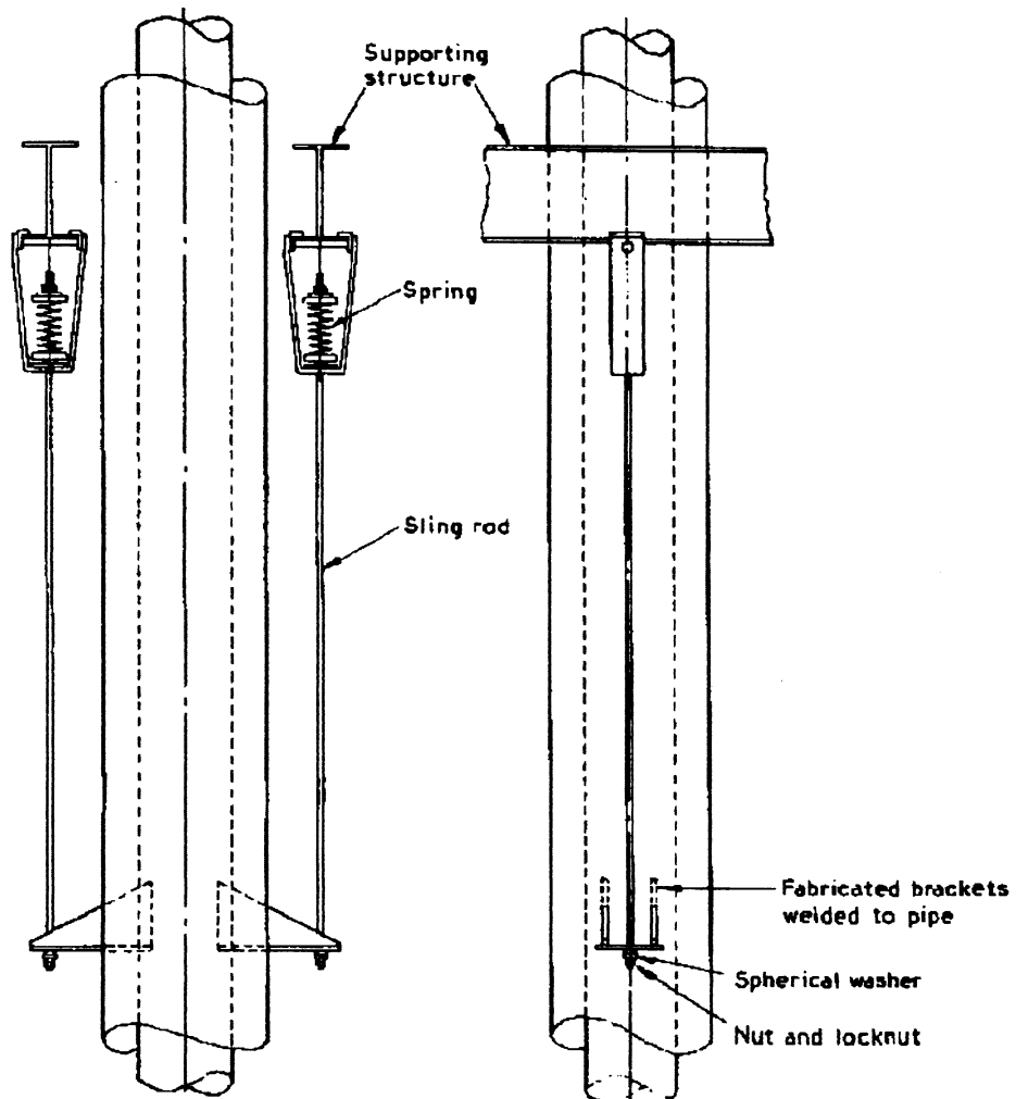
Figure 42 — Spring hanger for vertical pipes (variable load type)
