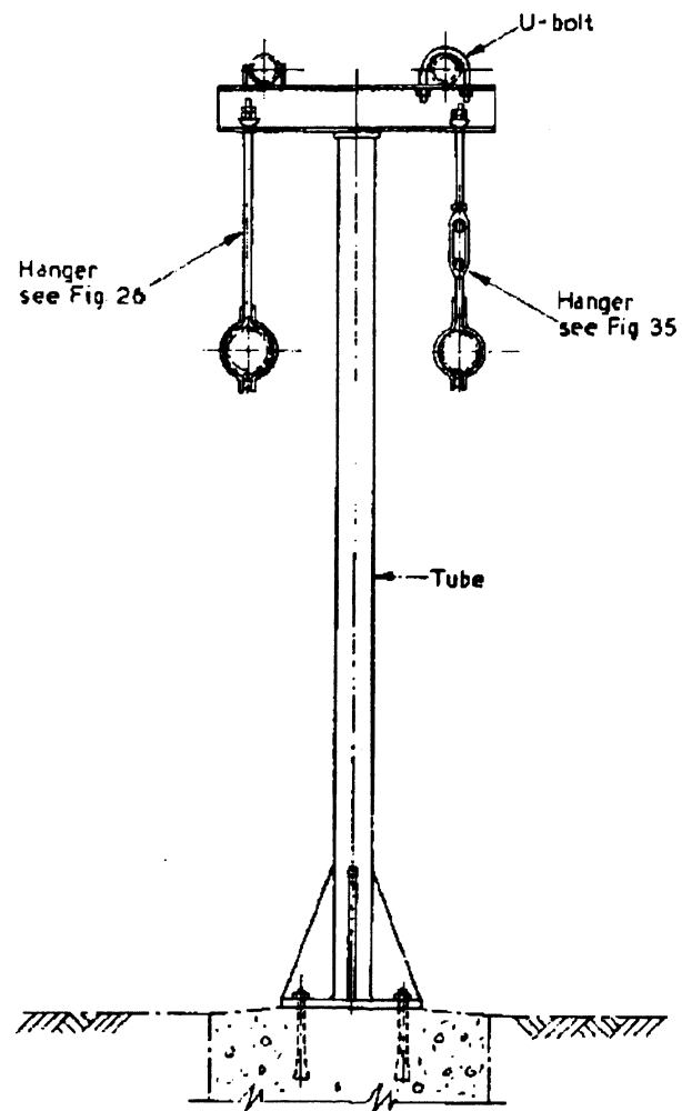
Figure 24 — Single tubular support
