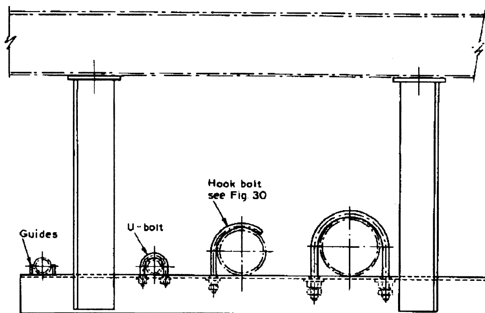
Figure 22 — Suspended support for multiple pipes
