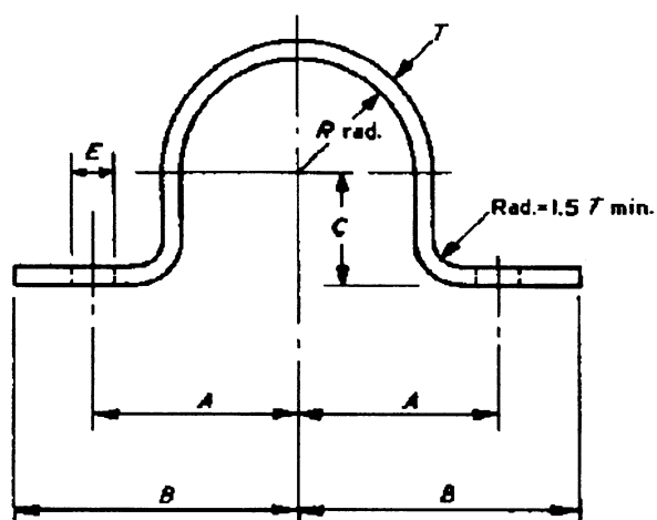
Figure 12 — Overstrap
