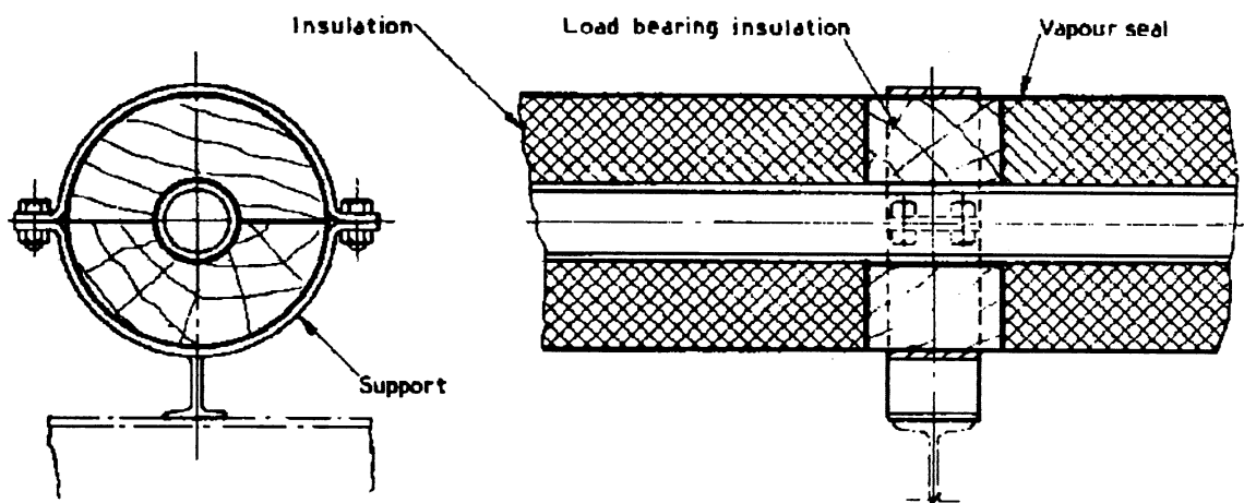
Figure 40 — Typical support for insulated cold pipe
