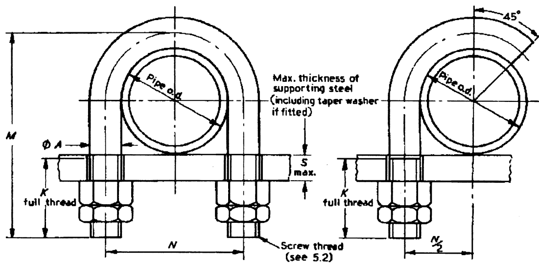
Figure 11a — U-bolt (to grip pipe)
