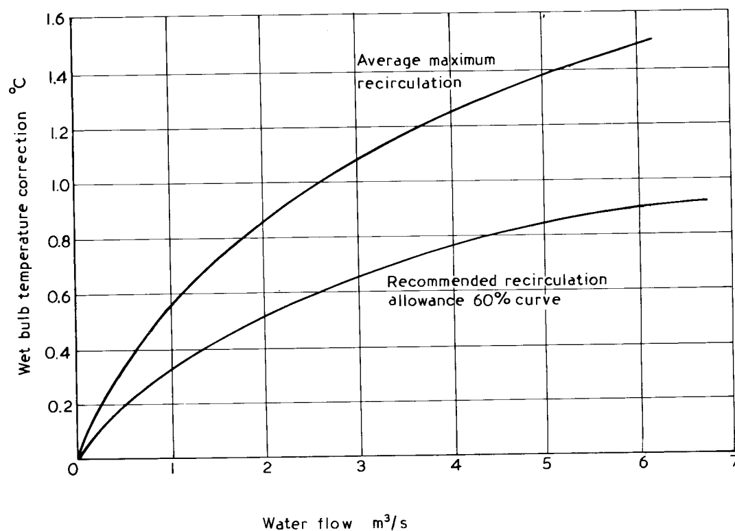
Figure 14. Basic recirculation allowance
