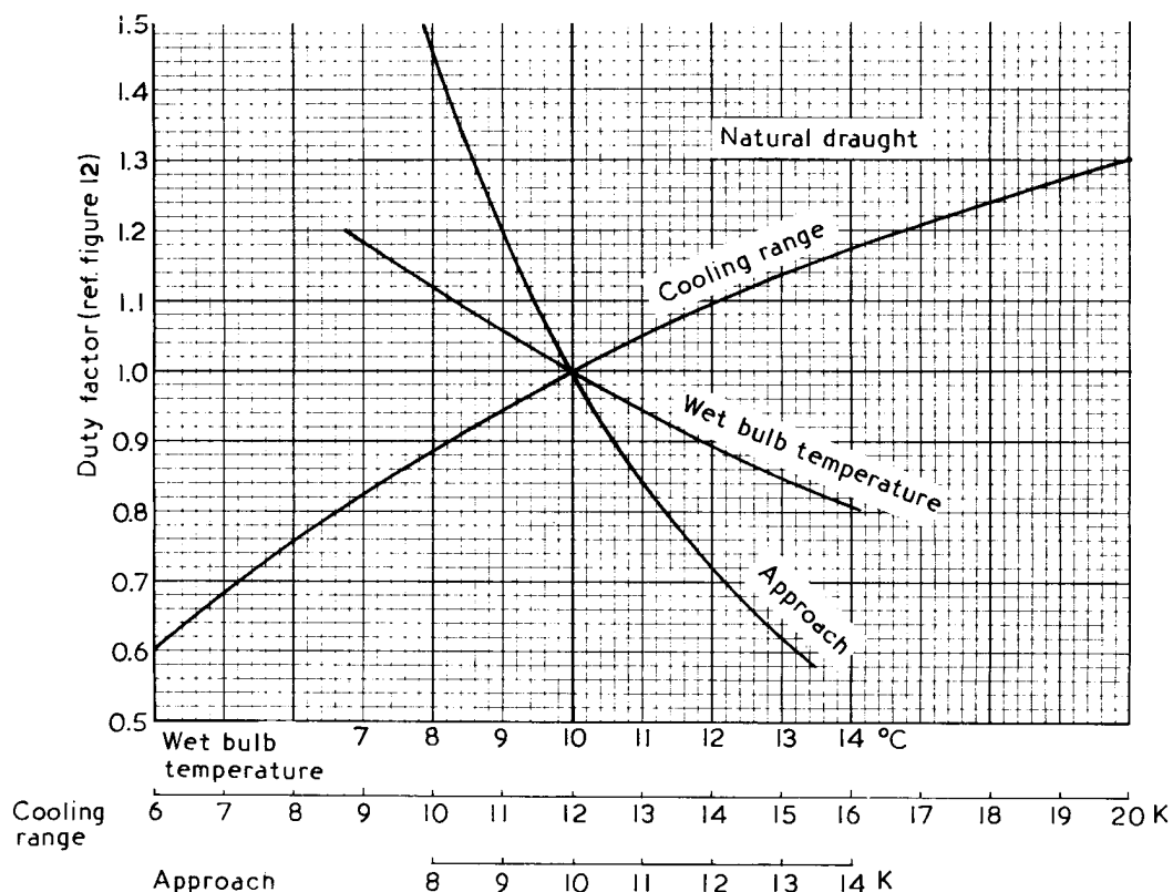
Figure 11. Natural draught tower: variation of duty factor with cooling range, approach and wet bulb temperature (at constant 70 % r.h.)
