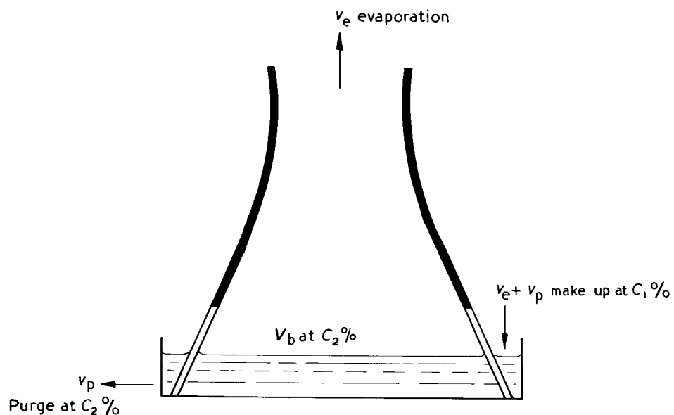
Figure 20. Purge, make-up and evaporation quantity balance
