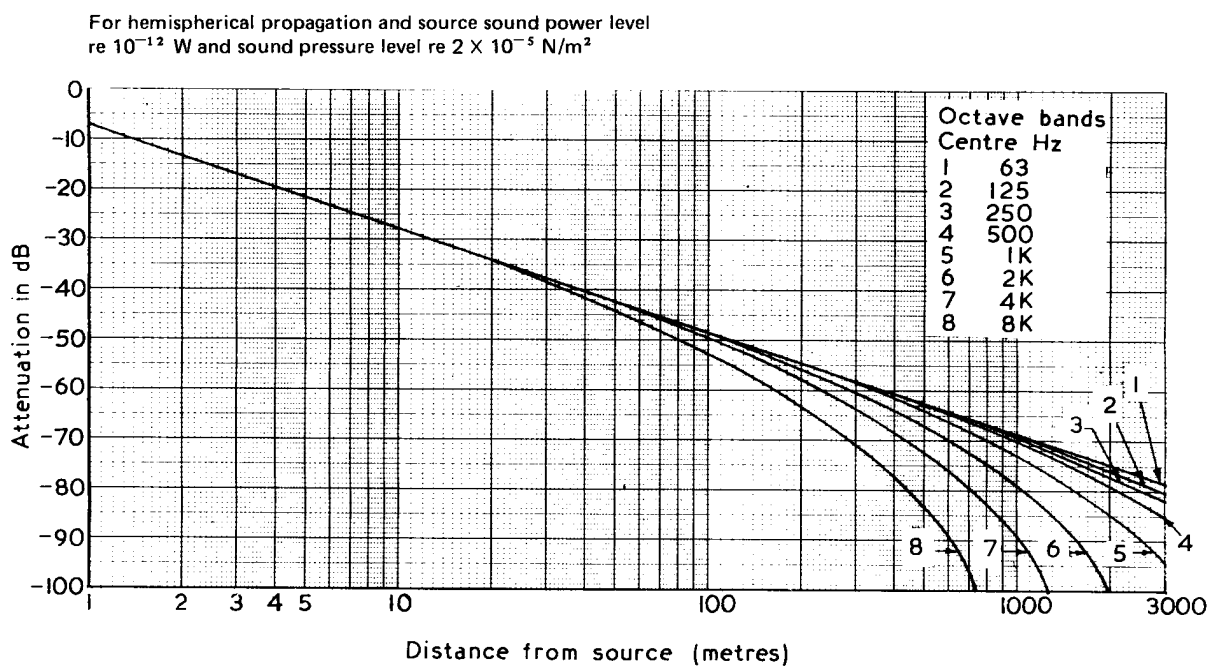
Figure 26. Attenuation for distance from source
