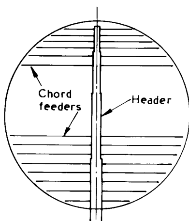
(b) Diametric header, chord feed
