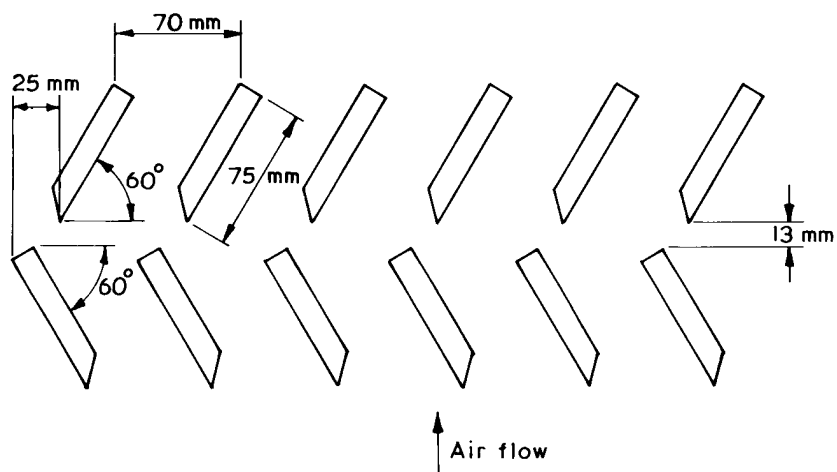
(a) Two layers of timber louvres
