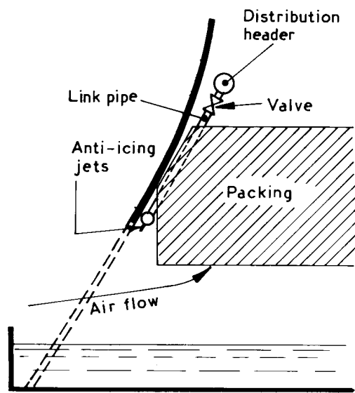
(a) Natural draught mixed flow
