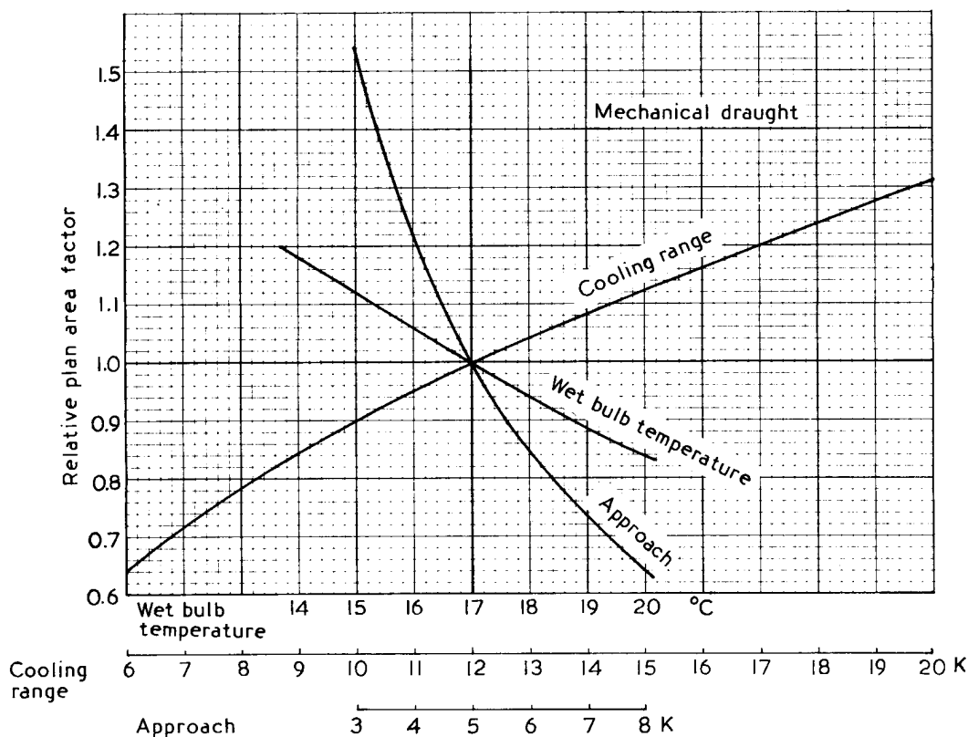
Figure 10. Mechanical draught counterflow tower: variation of tower size with cooling range, approach and wet bulb temperature
