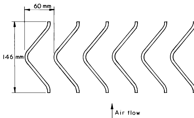
(b) Single layer of single corrugations
