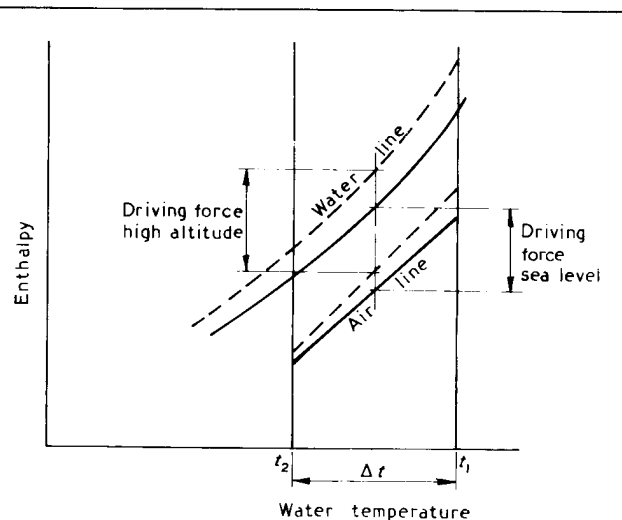
Figure 16. Effect of altitude on heat transfer diagram
