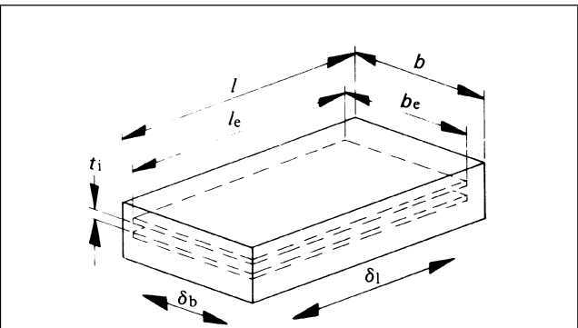
Figure 3 — Elastomeric laminated bearing
