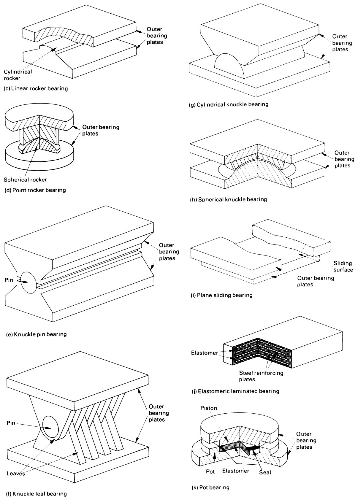
Figure 1 — Types of bearing (concluded)
