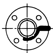
Figure 5 — Routing at flanges to avoid leaks and mechanical damage
