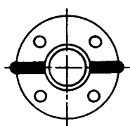
Figure 5 — Routing at flanges to avoid leaks and mechanical damage
