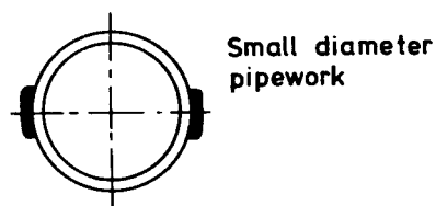
Figure 3 — Double run of heating tape straight traced on pipework without fittings
