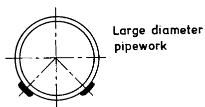
Figure 3 — Double run of heating tape straight traced on pipework without fittings
