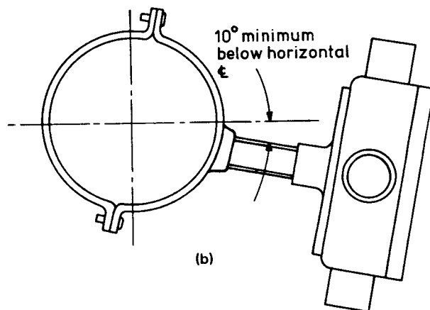
Figure 1 — Mounting of junction boxes on pipework
