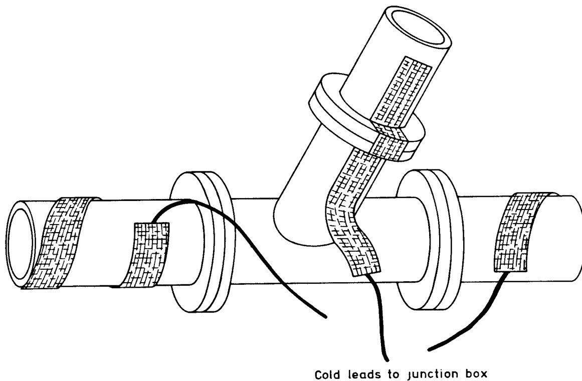
Figure 7 — Tracing on branch lines
