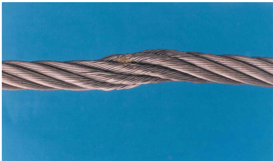
Figure 18 — Kink
