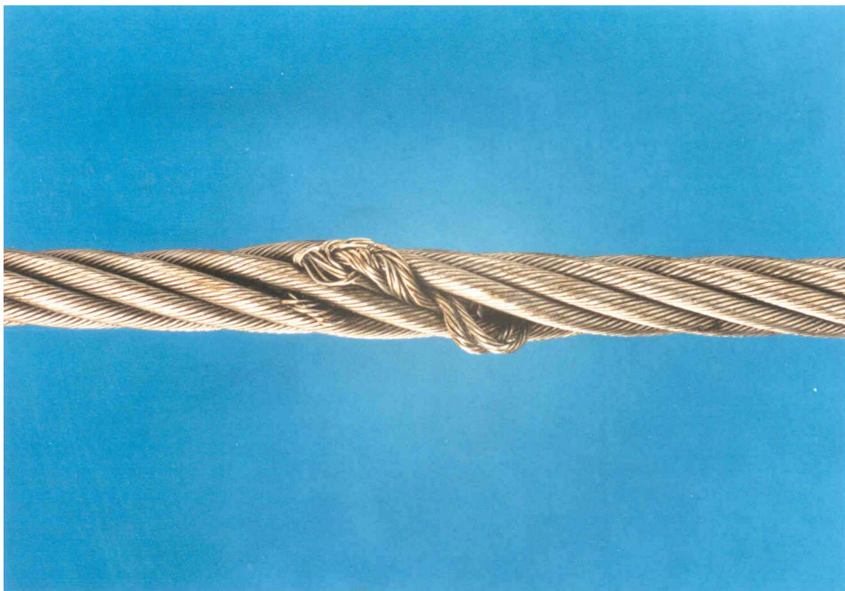
Figure 11 — Strand protrusion
