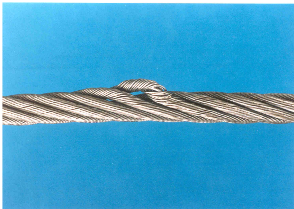
Figure 12 — Strand protrusion
