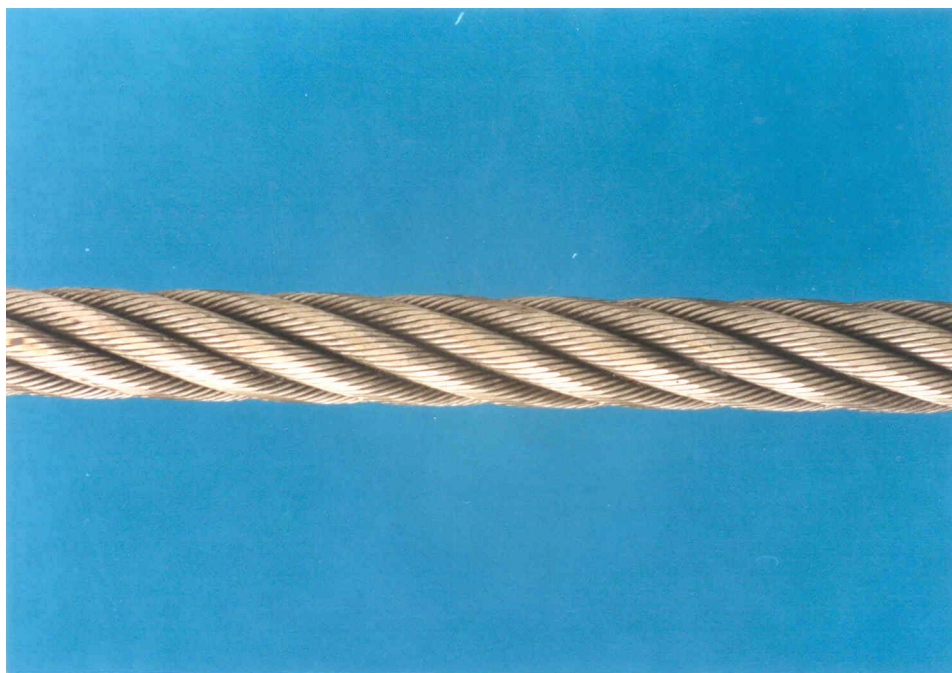
Figure 4 — External wear
