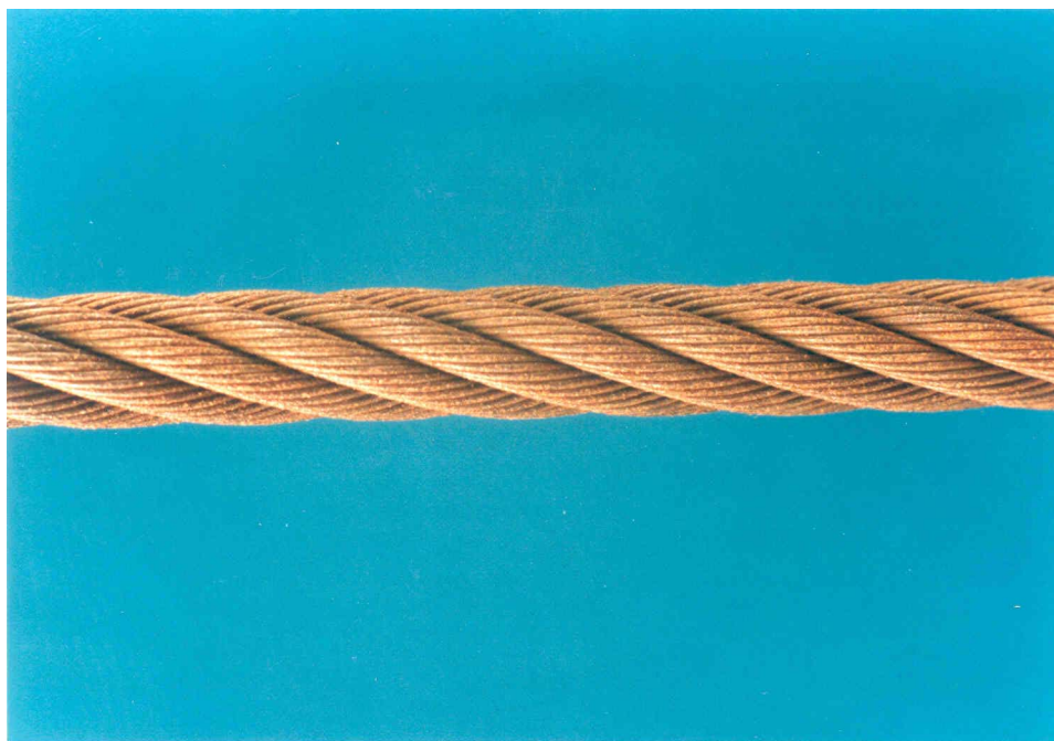
Figure 6 — External corrosion
