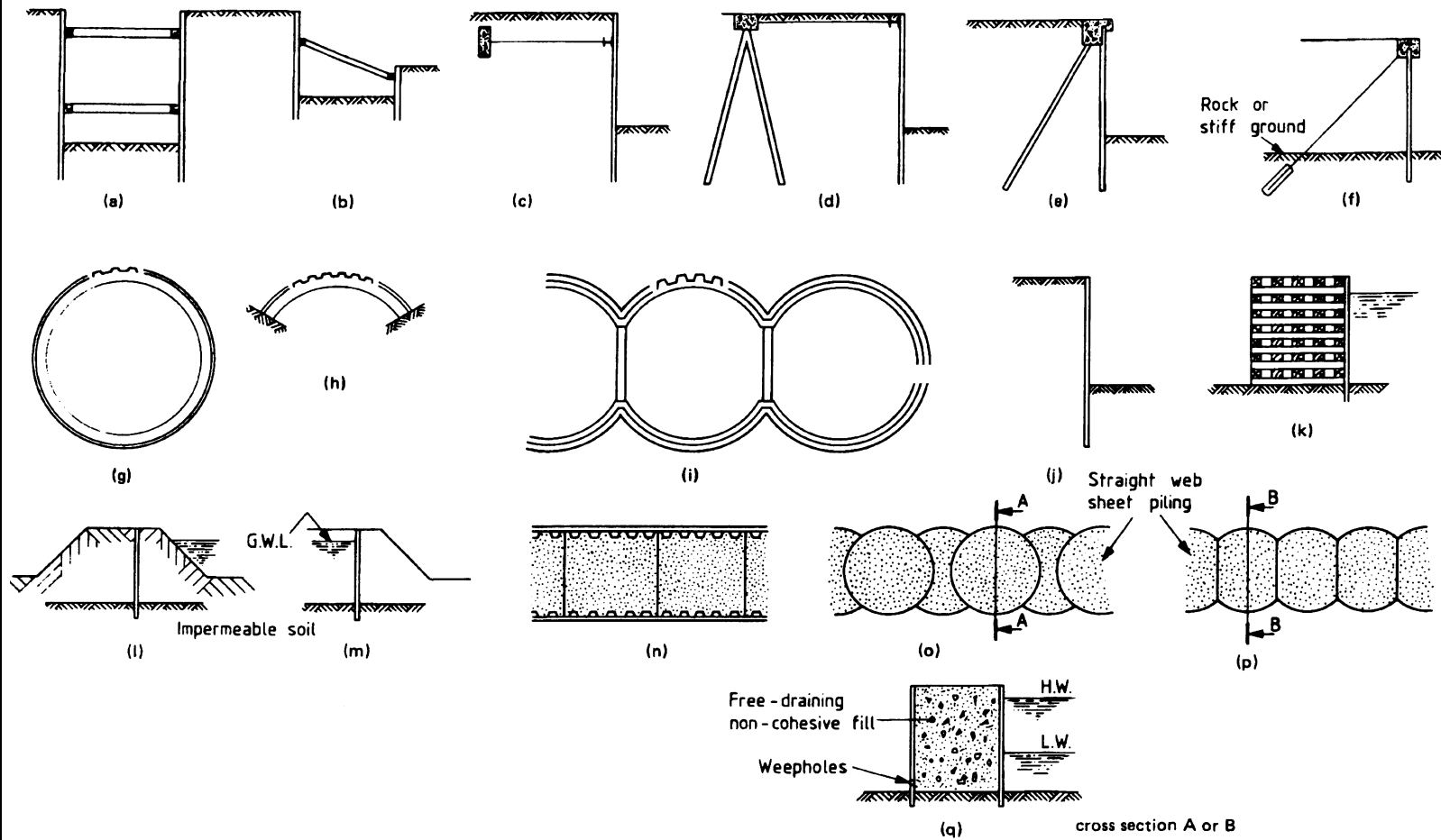
(b) Cofferdams using sheet piling
