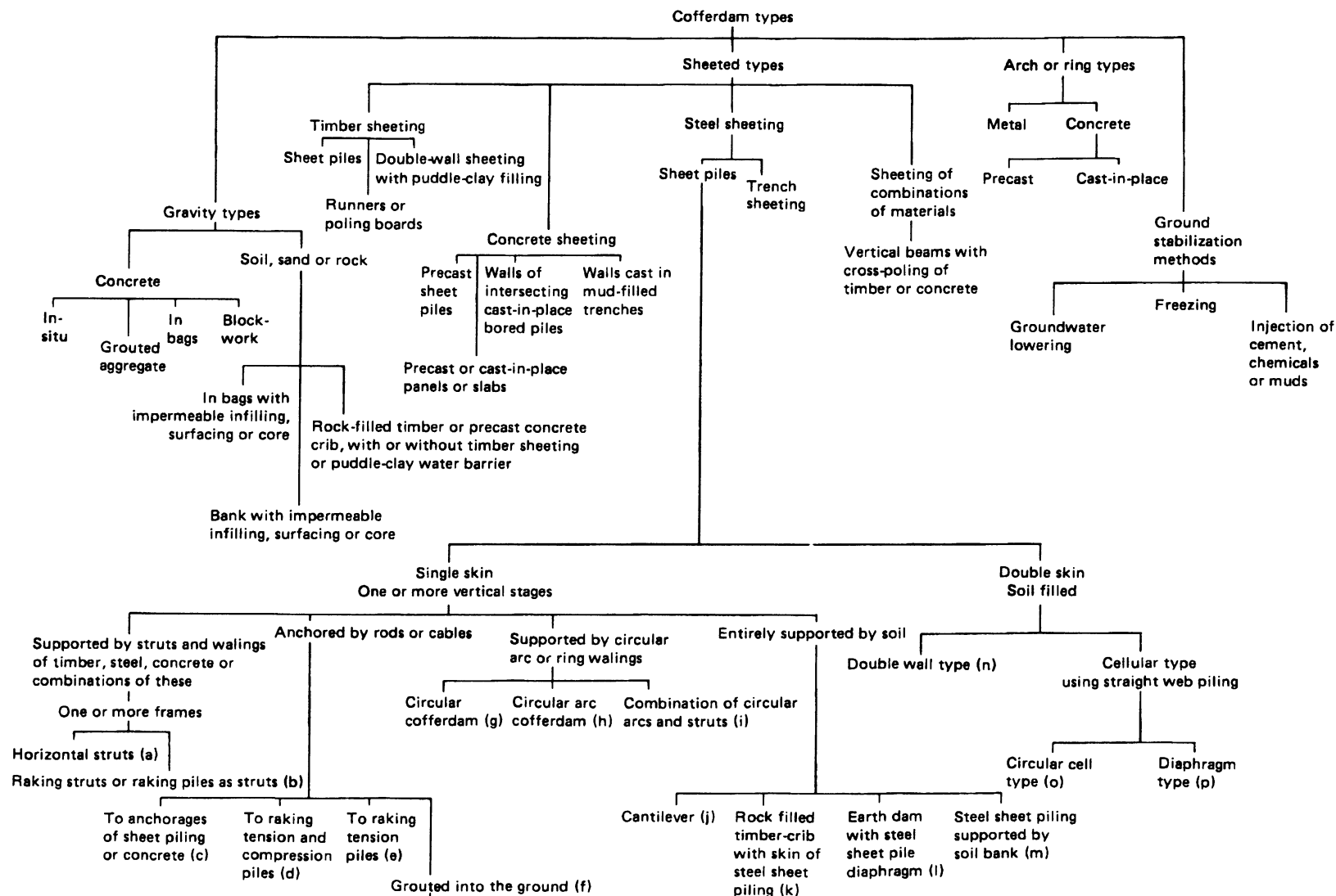
Figure 2 — Cofferdams
