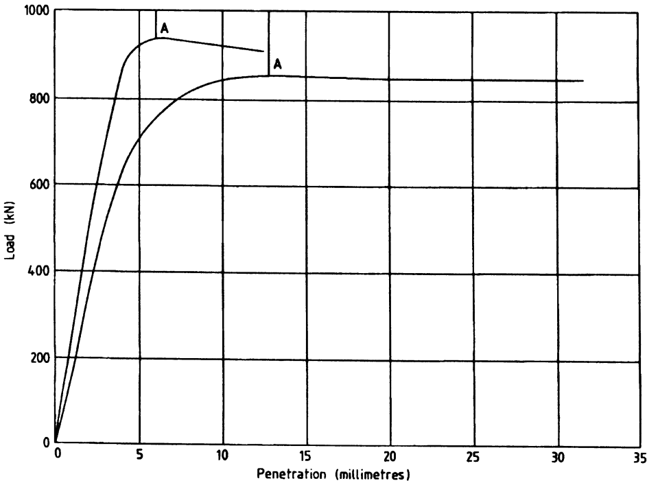
(a) Predominantly friction pile
