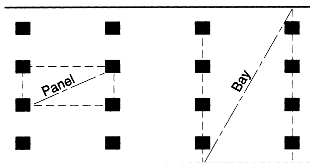
Figure 3.7 — Definition of panels and bays
