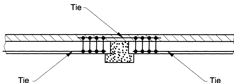
Figure 5.2 — Continuity of ties: anchorage by enclosing links
