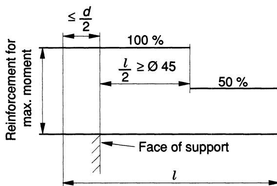
c) Cantilever
