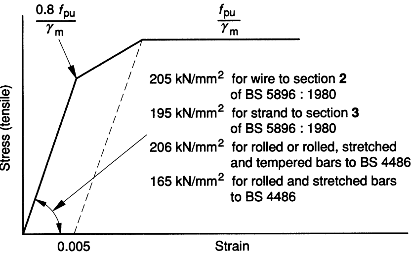
NOTE f_{pu} is in \text{N/mm}^2 . Figure 2.3 — Short term design stress-strain curve for prestressing tendons
