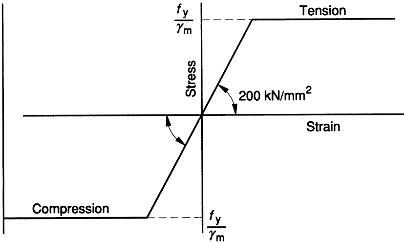
NOTE f_y is in \text{N/mm}^2 . Figure 2.2 — Short term design stress-strain curve for reinforcement
