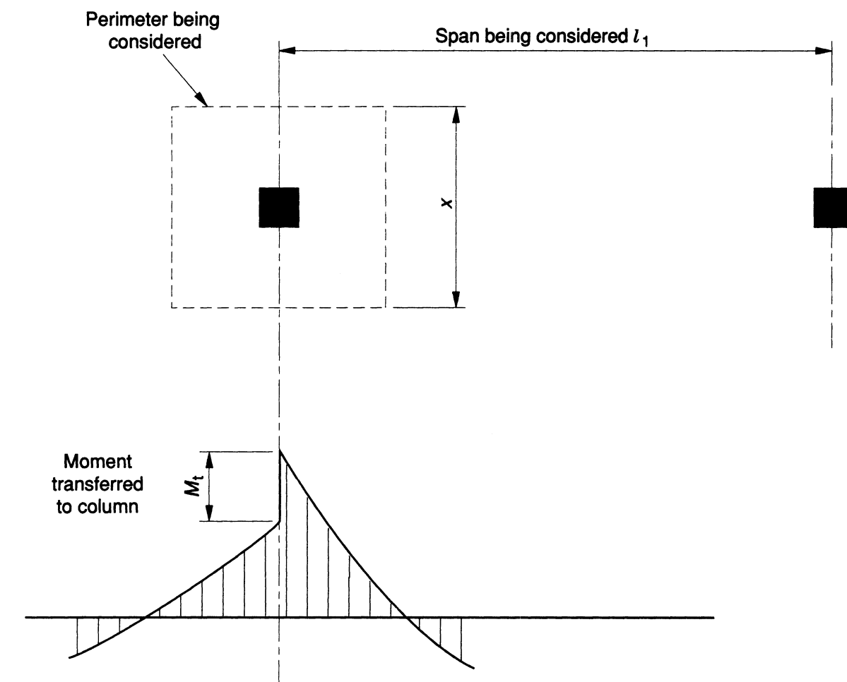
a) Bending moments diagram for load case being considered
