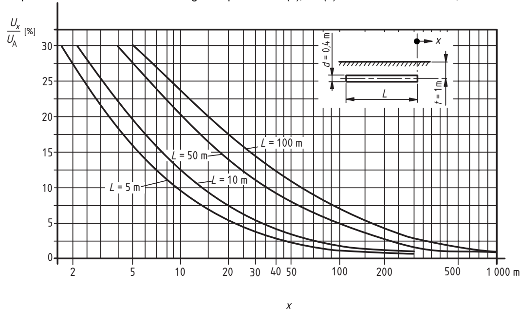
Figure D.1 — Voltage attenuation curve around an horizontal grounded measured in the direction of "X" (longitudinal axis of the grounded)
