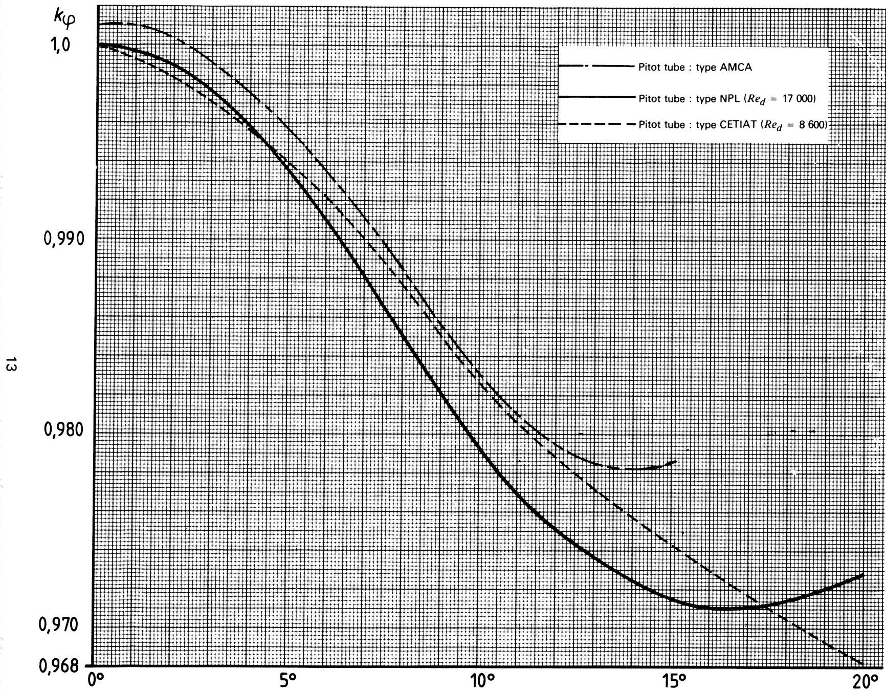
Figure 9 — k_\varphi versus \varphi for typical Pitot static tubes
