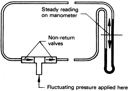
Figure 13 — Arrangement of non-return valves
