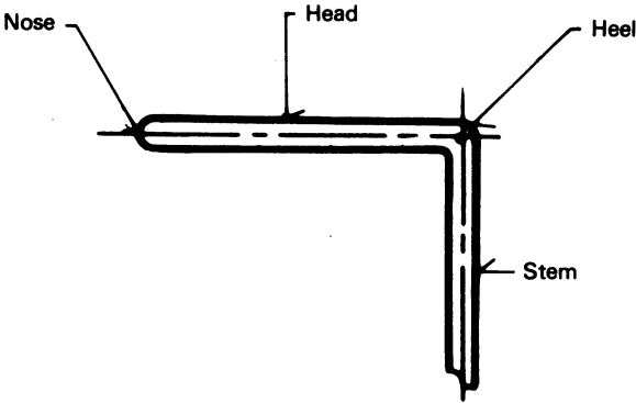
Figure 16 — Pitot static tube
