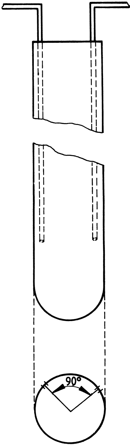
Figure 8 — Cylindrical yaw probe
