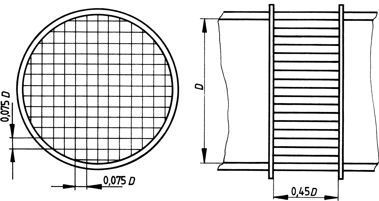
Figure 5 — Type D — AMCA straightener
