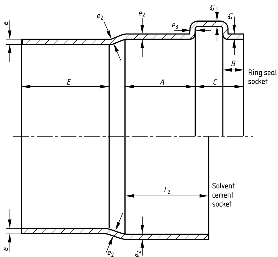
Figure 2 — Location of dimensions and spigots
