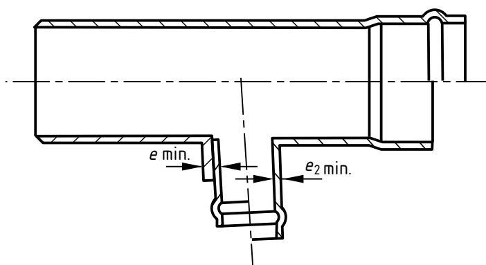
Figure 3 — Wall thickness of boss configurations
