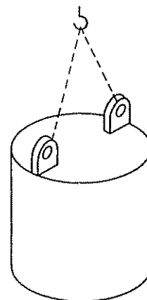
Figure 82. Lugs in a plane on a diameter
