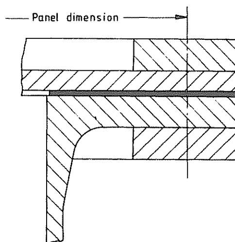
(b) Blanked full-face flange with backing rings
