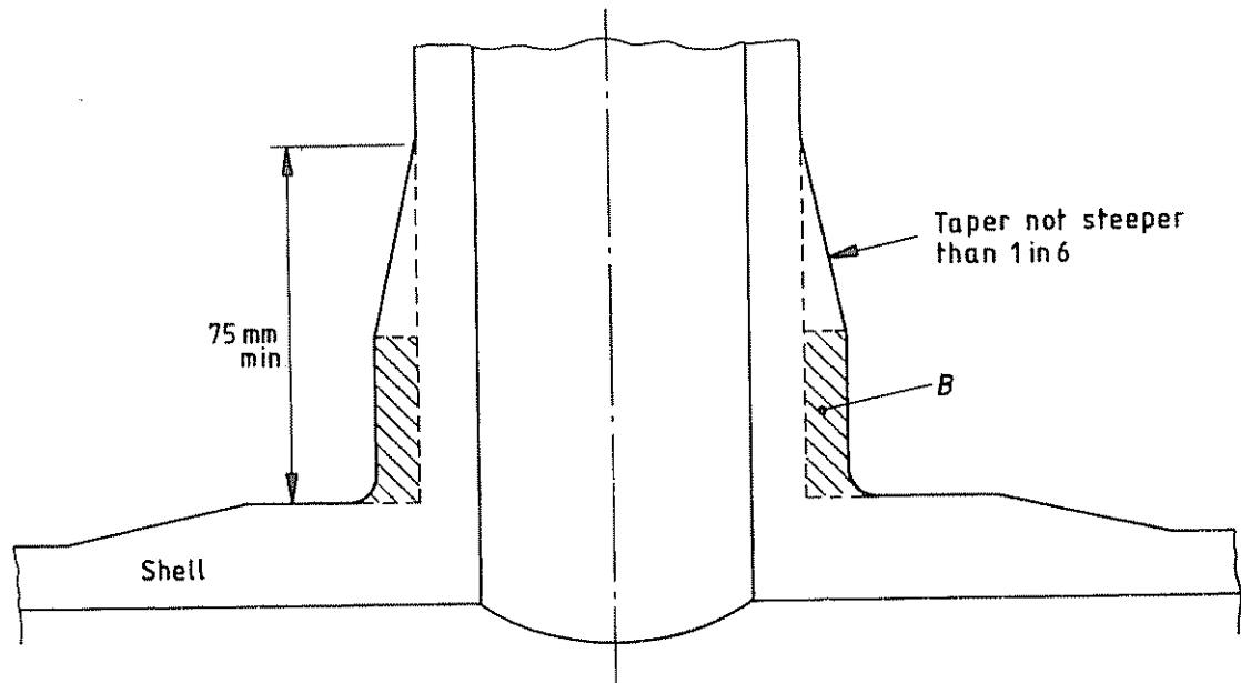
Figure 21. Arrangement of branch overlay for long branches (applicable to all types of branch construction in figure 20)
