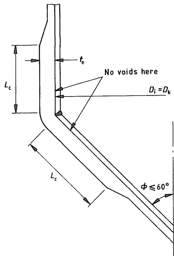
(b) Conical section without knuckle (only with fabric-backed thermoplastics lining (see 18.4.1))
