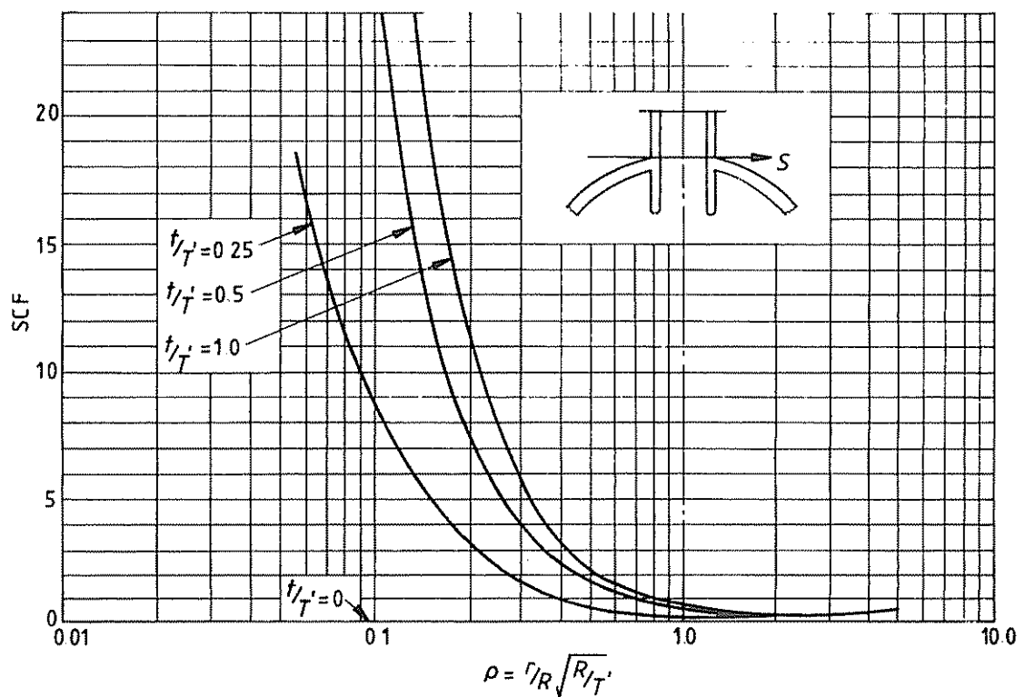
Figure 79. Maximum stress in sphere for shear loading (protruding nozzles)
