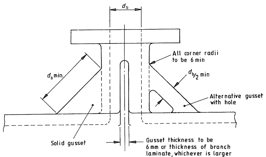
Figure 22. Gussets for branches
