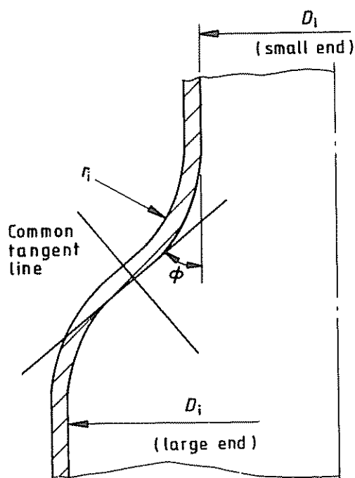
(c) Conical section with knuckles
