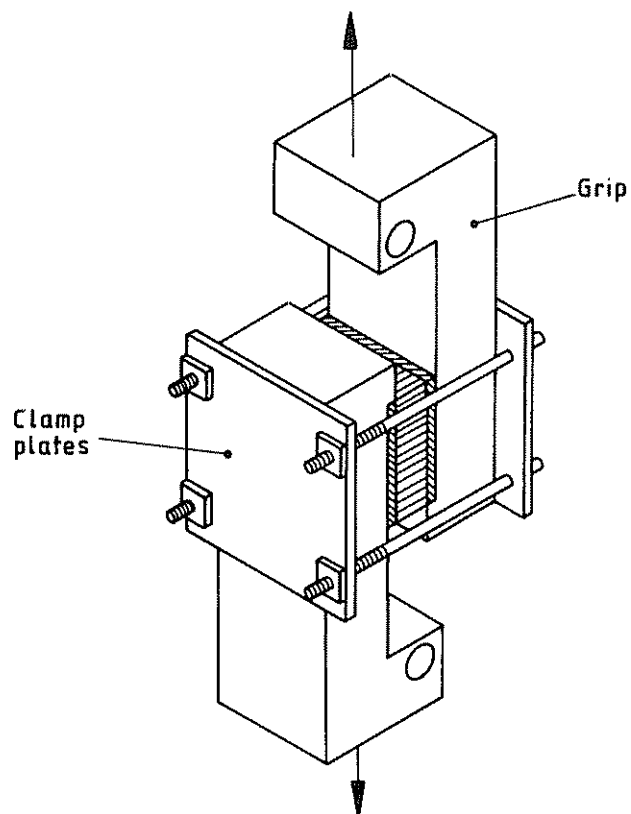
Figure 38. Assembly of test specimen and grips
