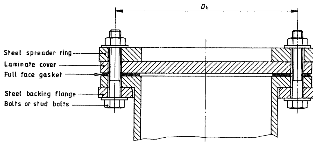
(b) Full-face gasket
