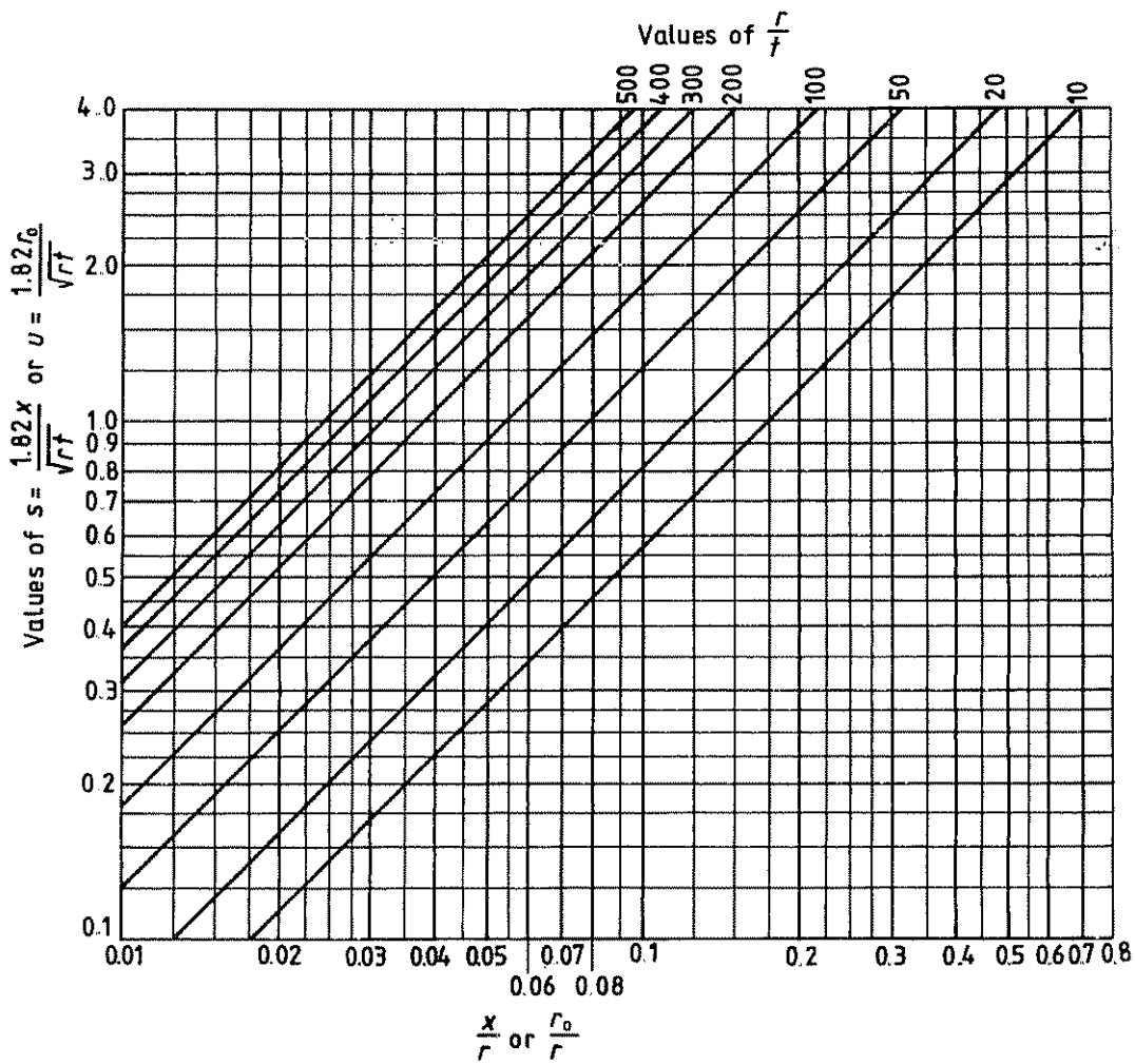
Figure 65. Chart for finding s and u
