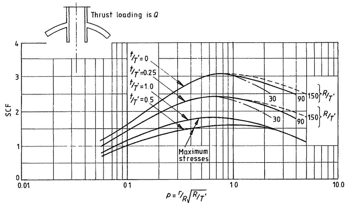
Figure 75. Maximum stress in sphere for thrust loading (protruding nozzles)
