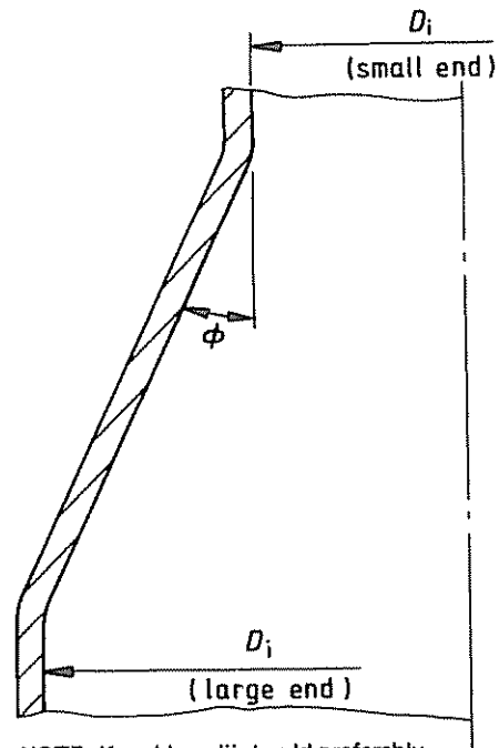
(c) Conical section with knuckles
