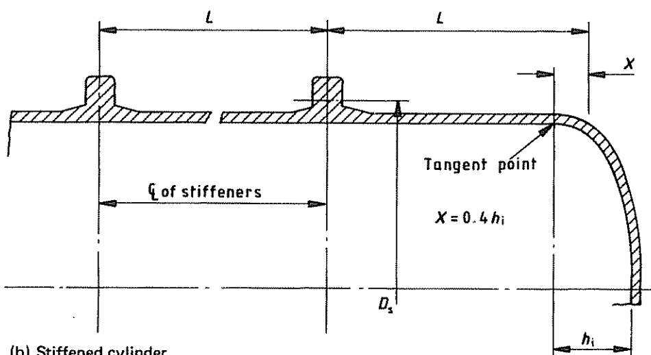
(b) Stiffened cylinder
