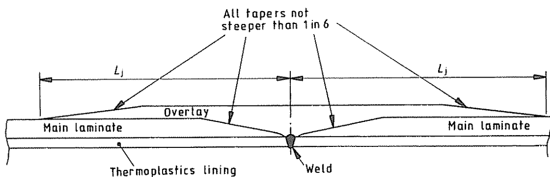
(a) Feathered joint
