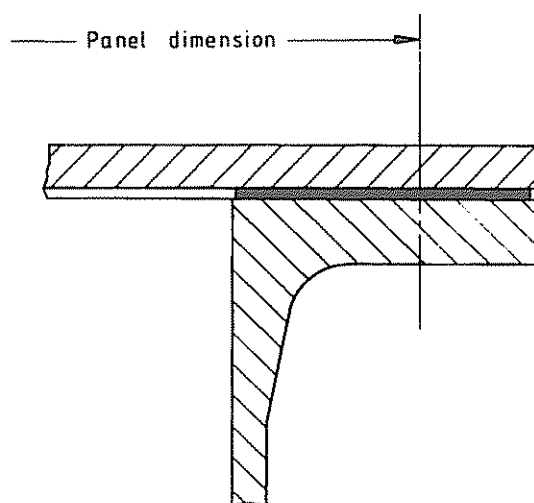
(a) Blanked full-face flange
