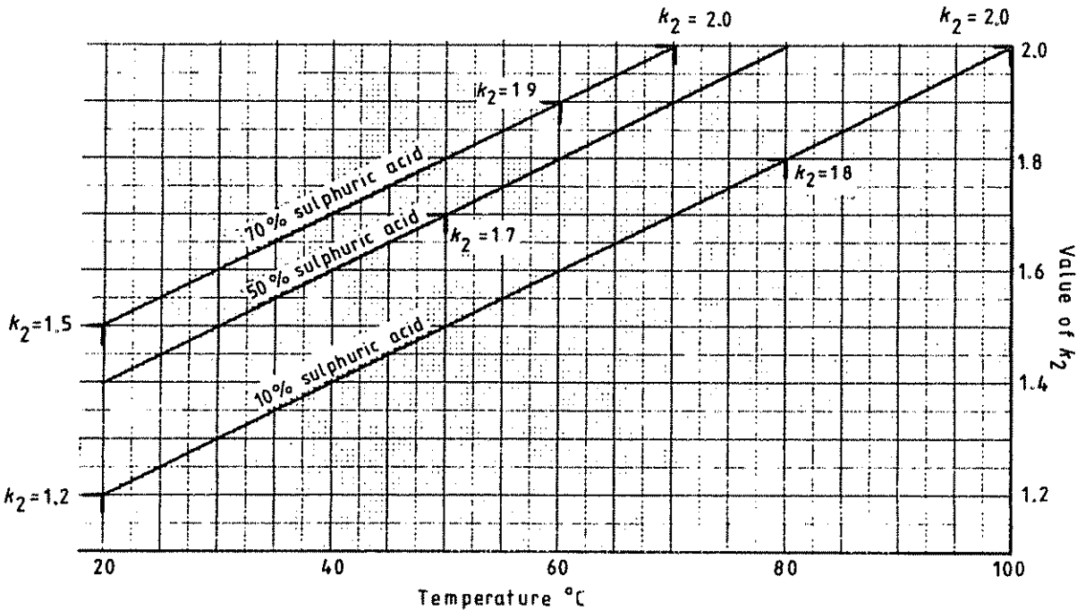
Figure 42. Graphical determination of k_2 : example E
