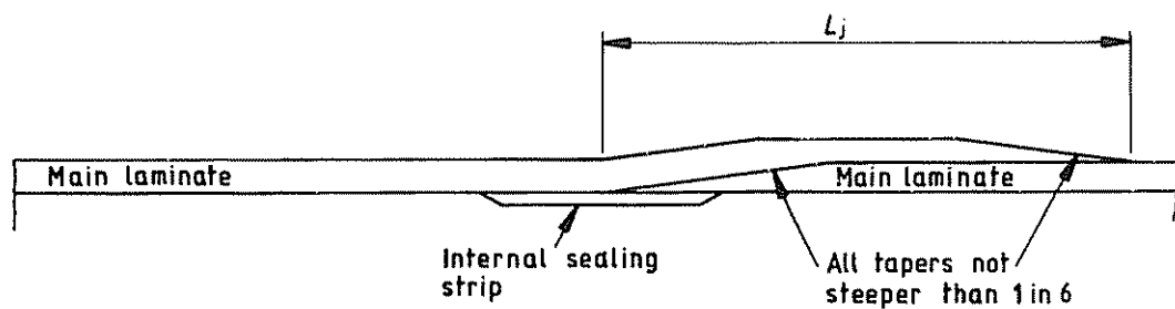
(e) Main laminate overlay joint
