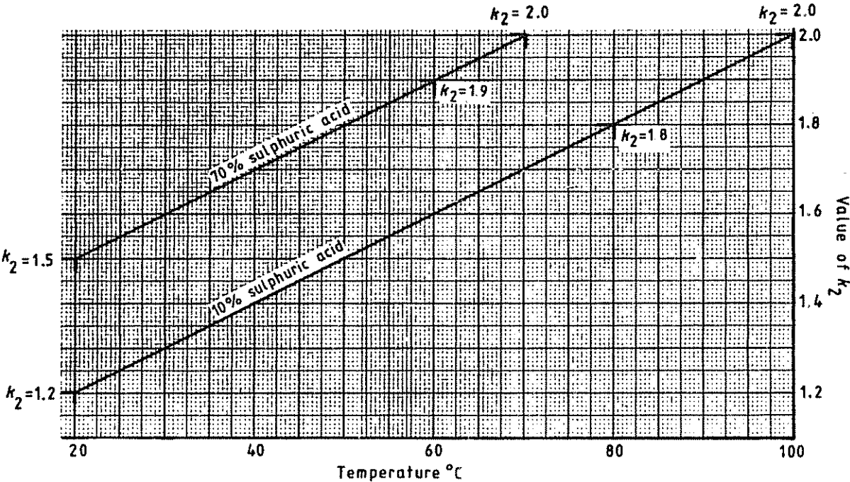
Figure 41. Graphical determination of k_2 : example D
