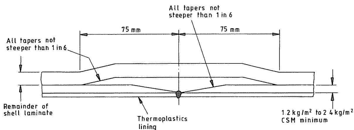
(b) Skin form main seam joint
