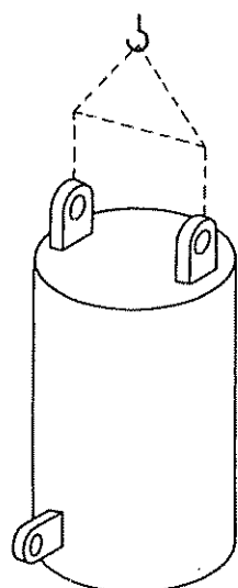
Figure 81. Parallel lugs
