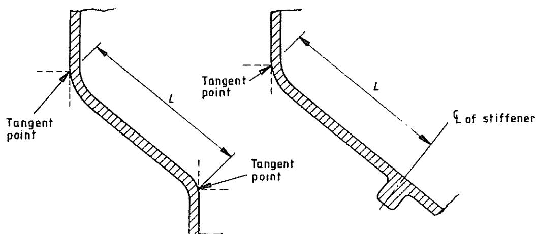
(c) Conical sections
