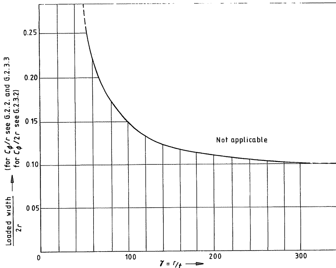
Figure 43. Restriction on vessel/attachment geometry (see G.2.2 and G.2.3)
