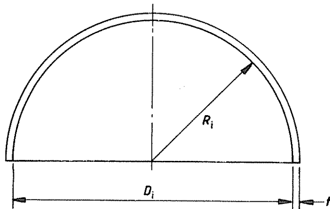
(a) Hemispherical
