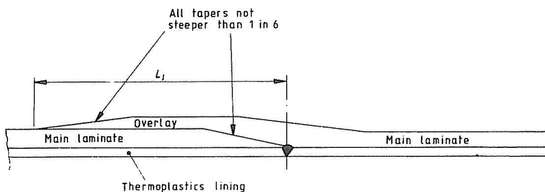
(c) Main laminate overlay joint
