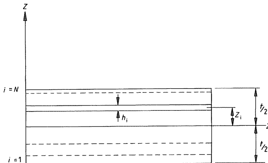
Figure 31. n ply laminated beam
