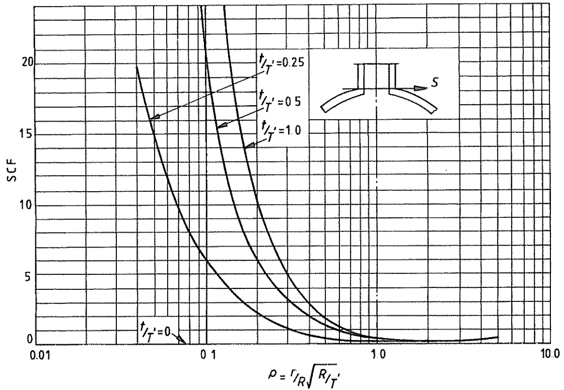
Figure 78. Maximum stress in sphere for shear loading (flush nozzles)
