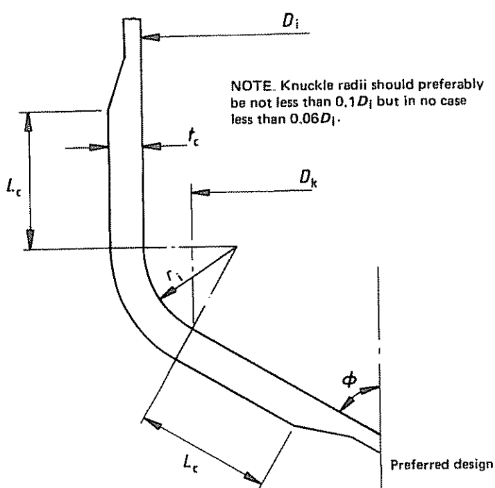
(a) Conical section with knuckle
