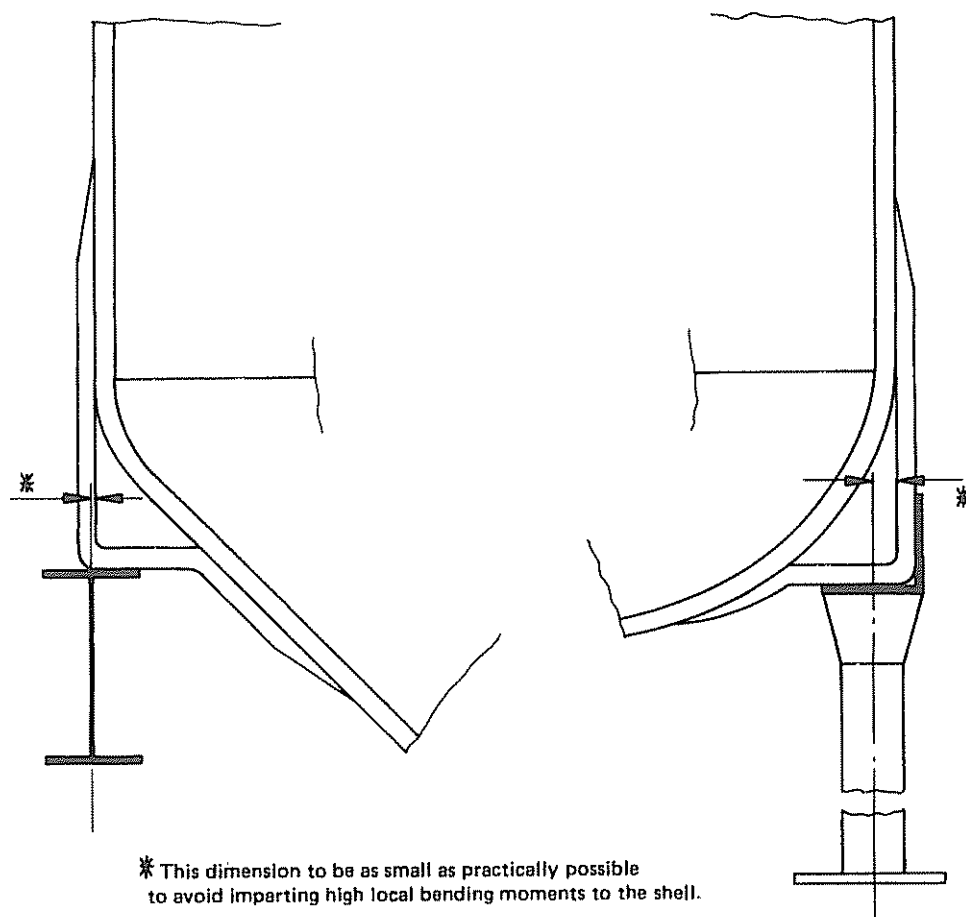
(a) Angle ring
