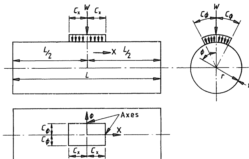
Figure 44. Vessel with central radial load
