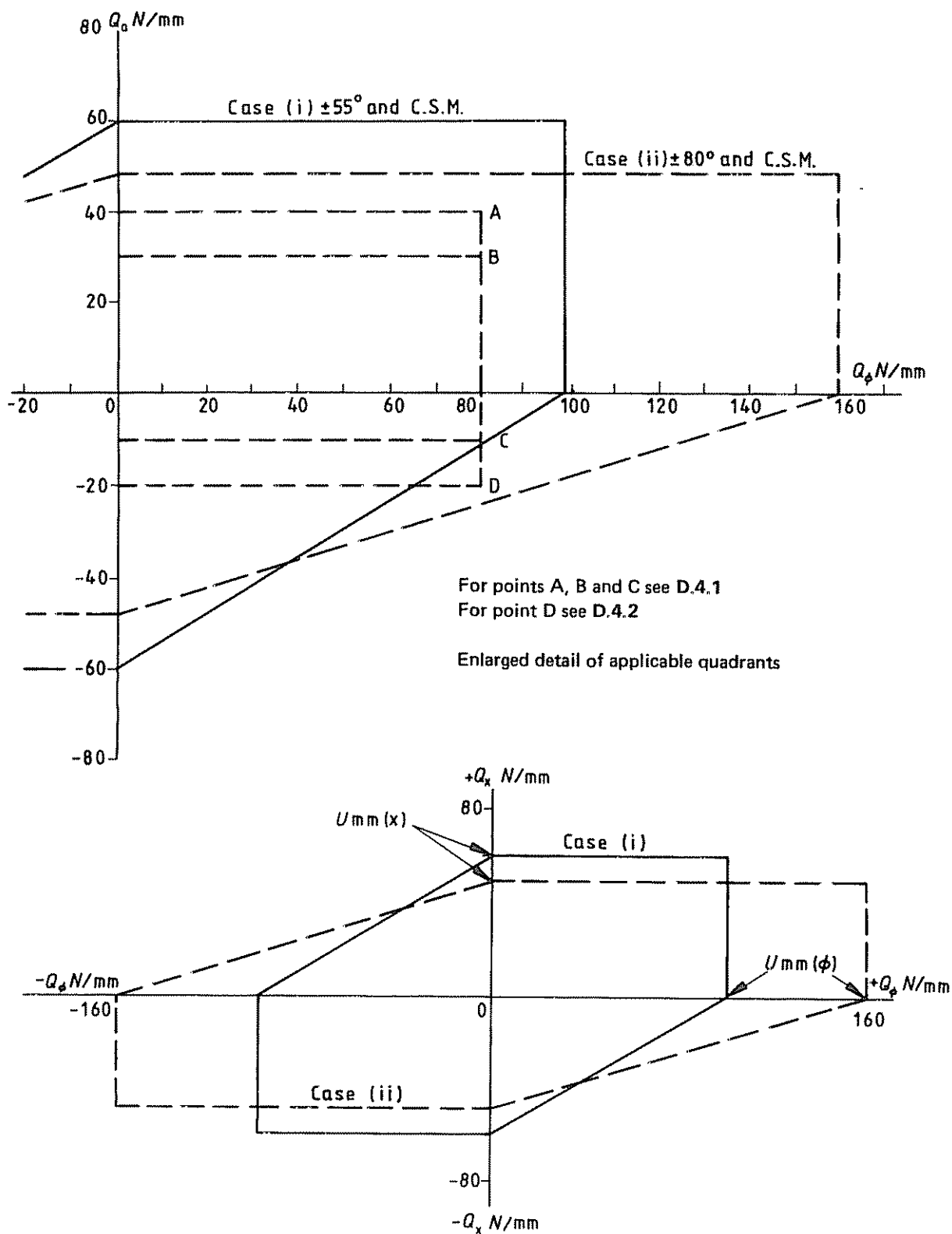
Figure 39. Biaxial design envelopes
