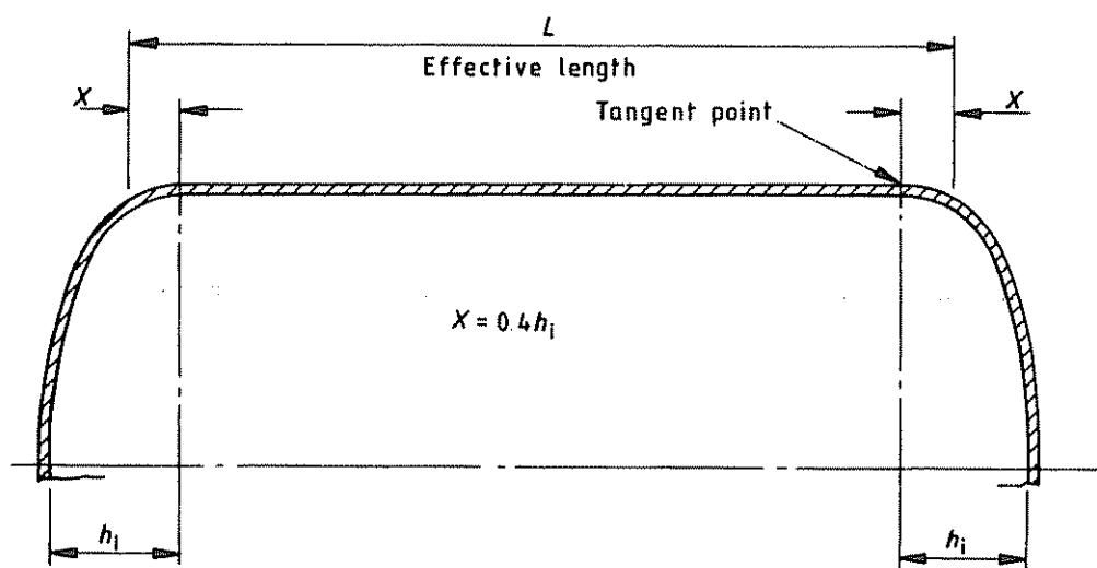
(a) Unstiffened cylinder
