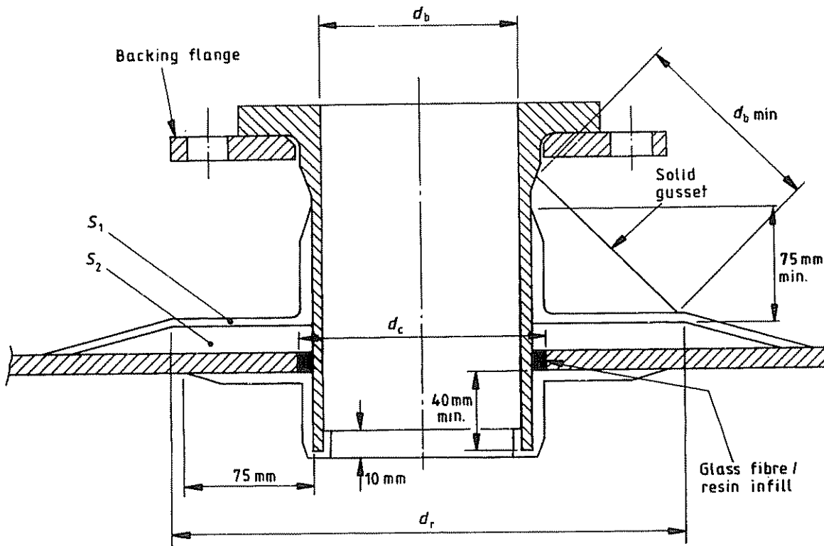
(b) Set through branch without thermoplastics lining (50 mm to 100 mm bore)
