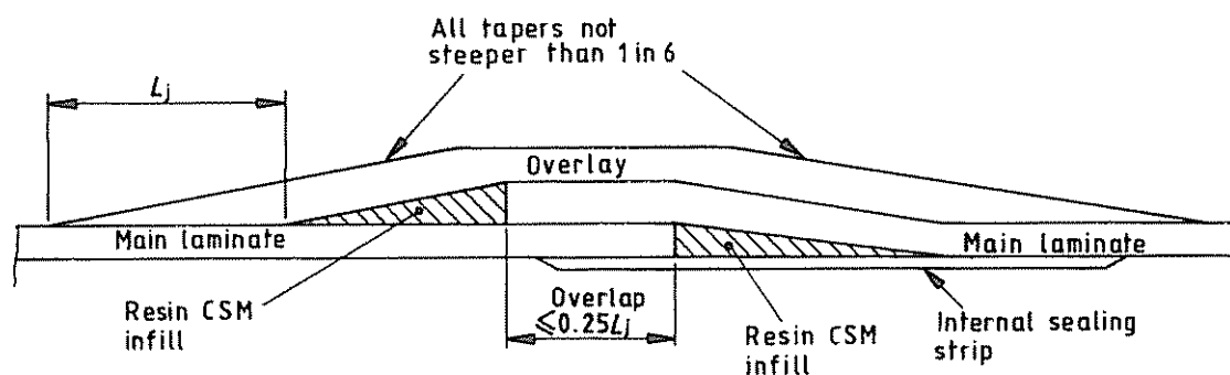
(b) Spigot and socket joint, limited to main laminate of 6 mm or less
