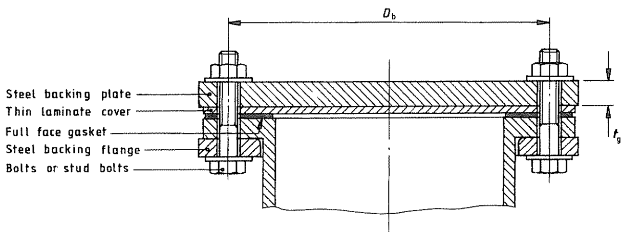
(b) Fully-supported
