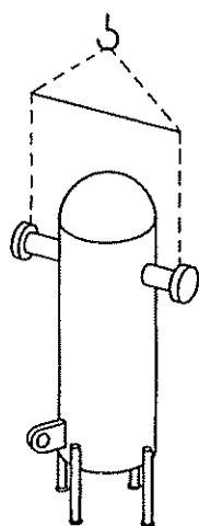
Figure 80. Trunnions
