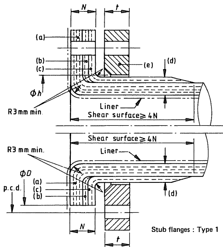
Figure 24. Flange construction
