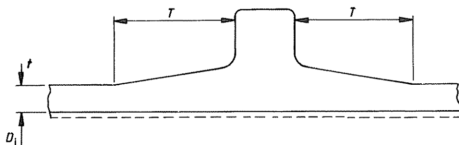
(c) Stiffeners
