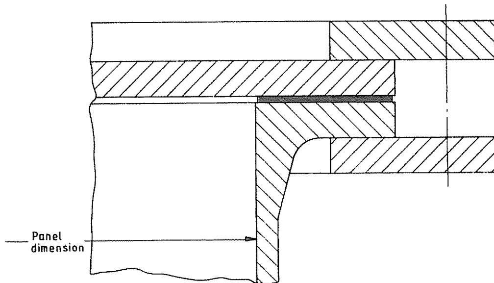
(a) Blanked stub flange with backing rings
