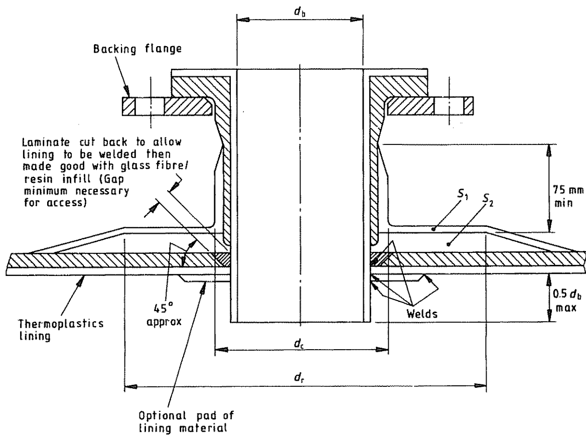
(f) Set through branch with thermoplastics lining
