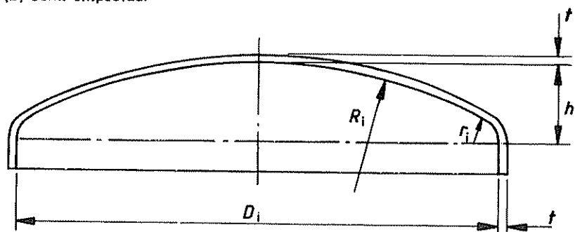
(c) Torispherical
