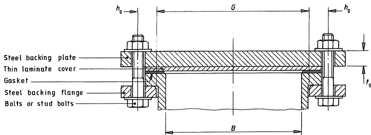
(a) Fully-supported
