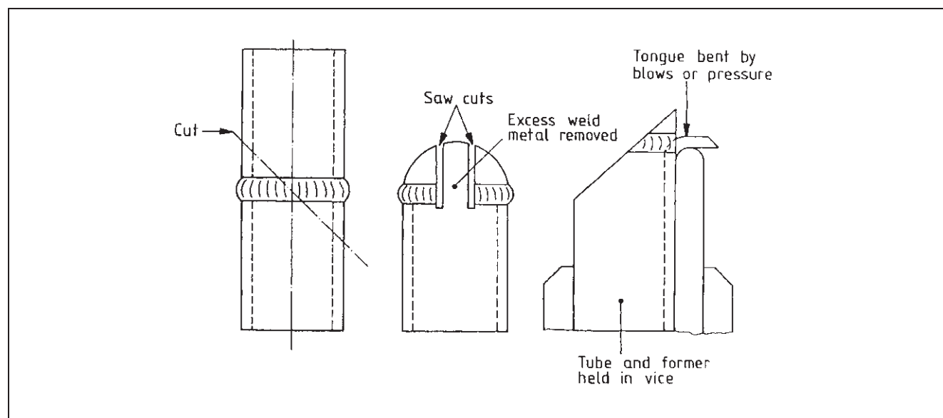
Figure 94 Tongue-bend test specimen
