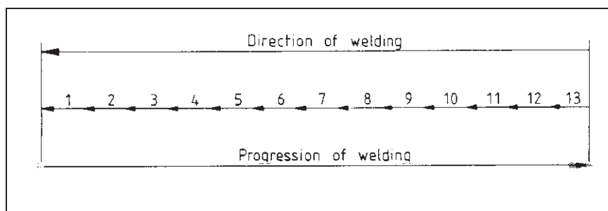
Figure 49 Example of back-step sequence
