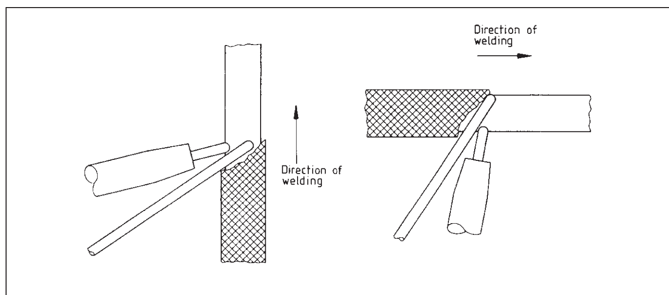
Figure 82 All-position rightward welding
