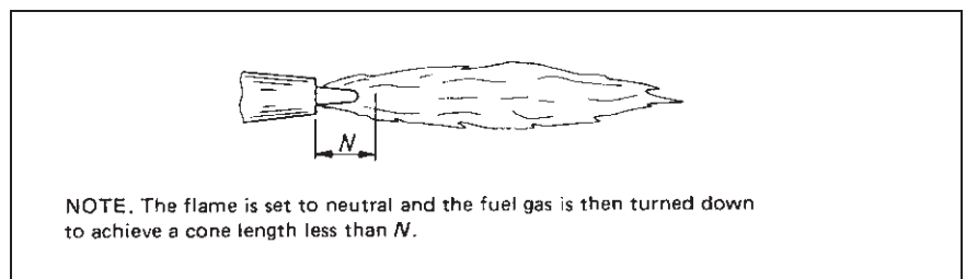
Figure 79 Oxidizing oxy-acetylene flame
