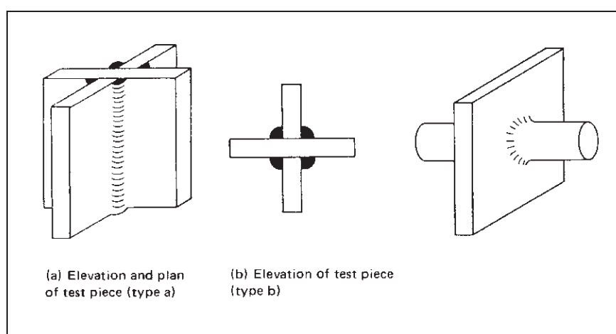
Figure 92 Cruciform test pieces
