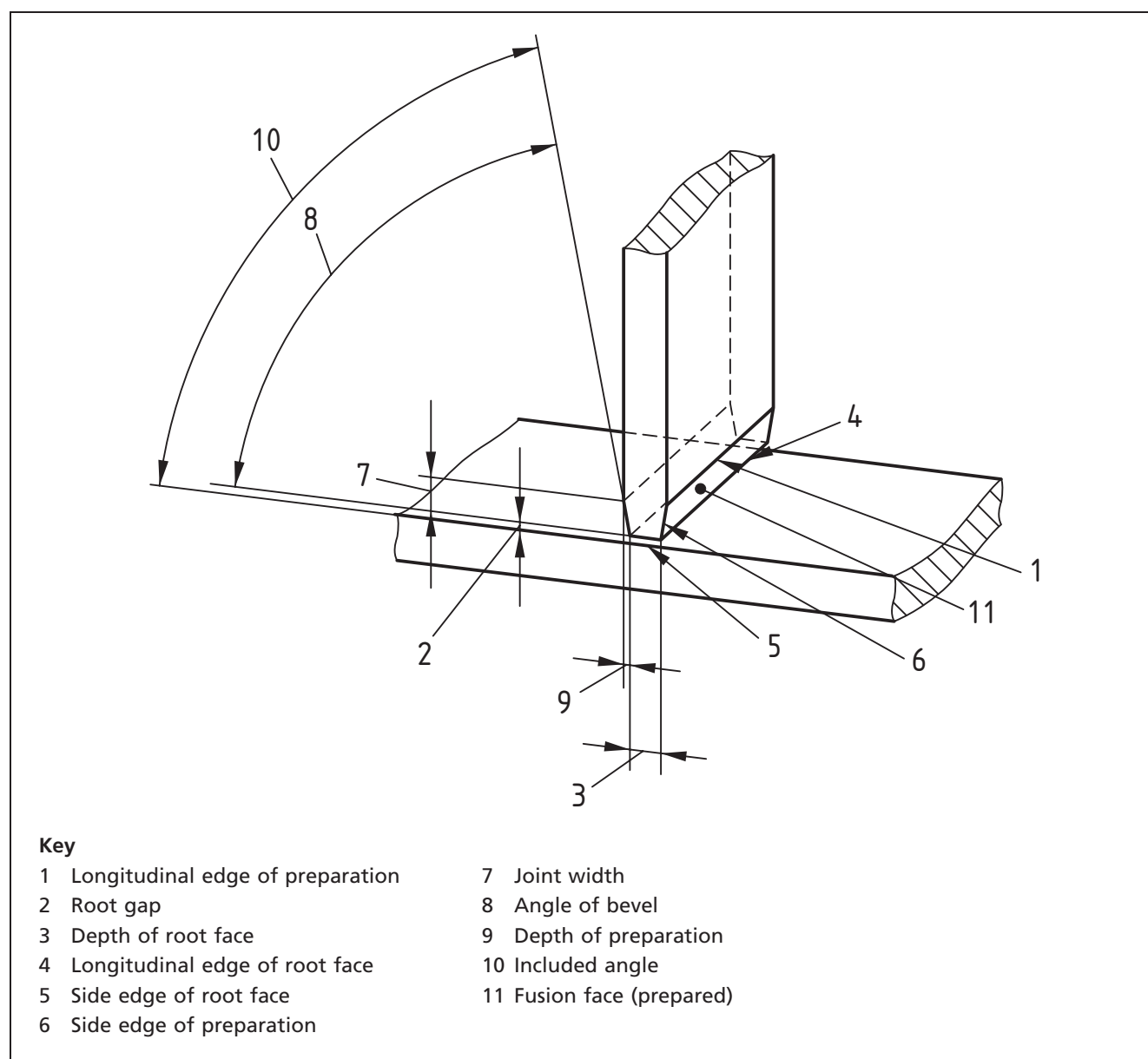
Figure 61 Preparation for double-bevel T-butt welds
