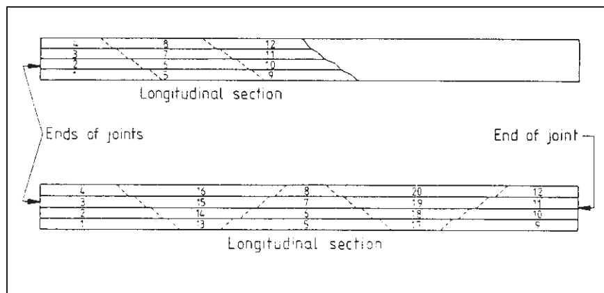
Figure 70 Examples of block sequences
