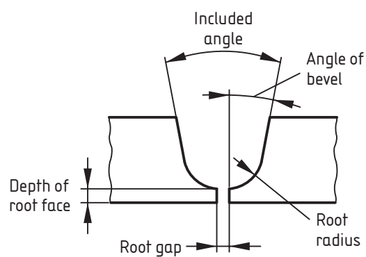
b) Single sided U-butt
