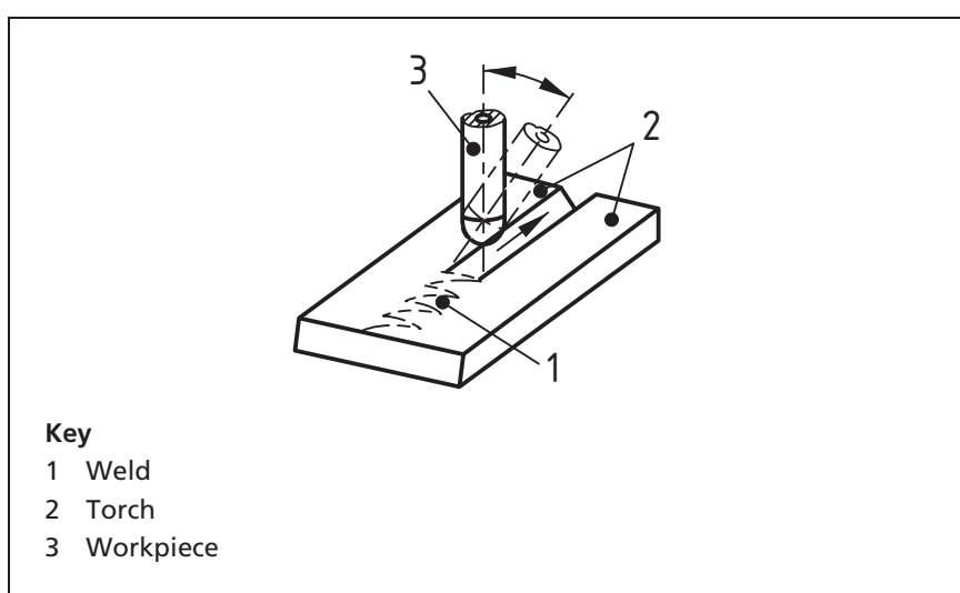
Figure 68 Weave technique
