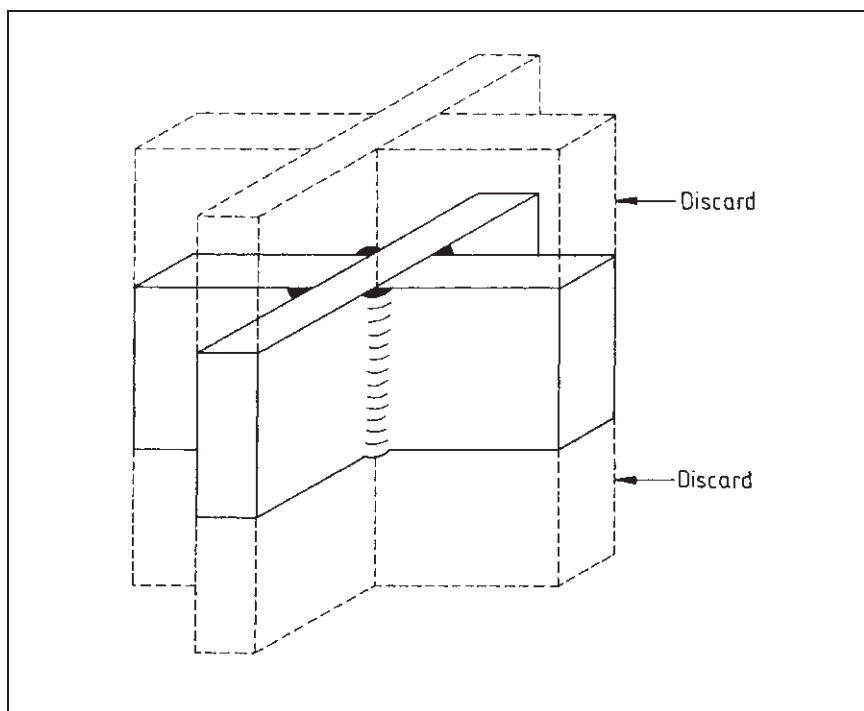
Figure 93 Method of obtaining cruciform test specimen
