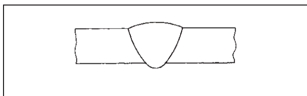
Figure 102 Excess penetration bead
