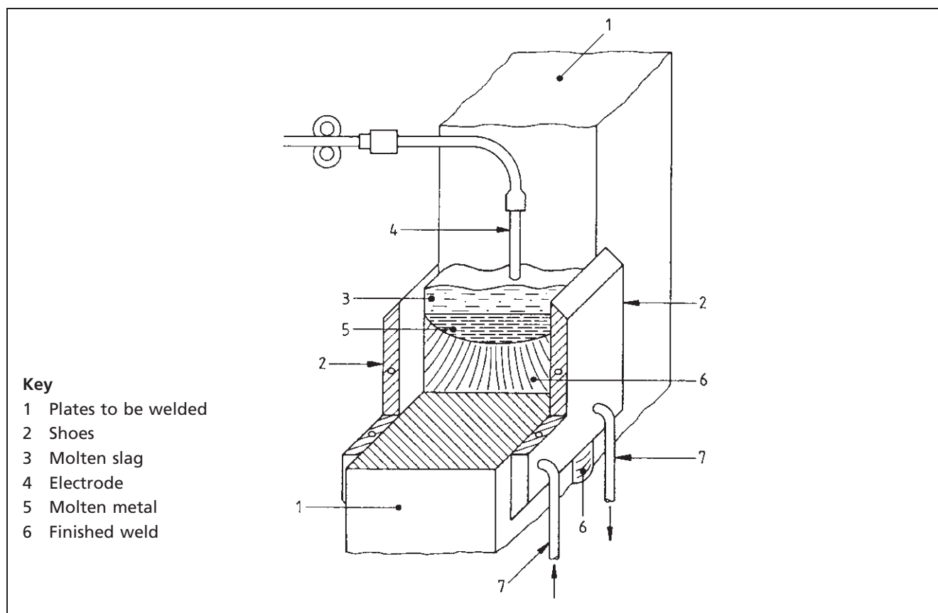
Figure 87 Electro-slag welding
