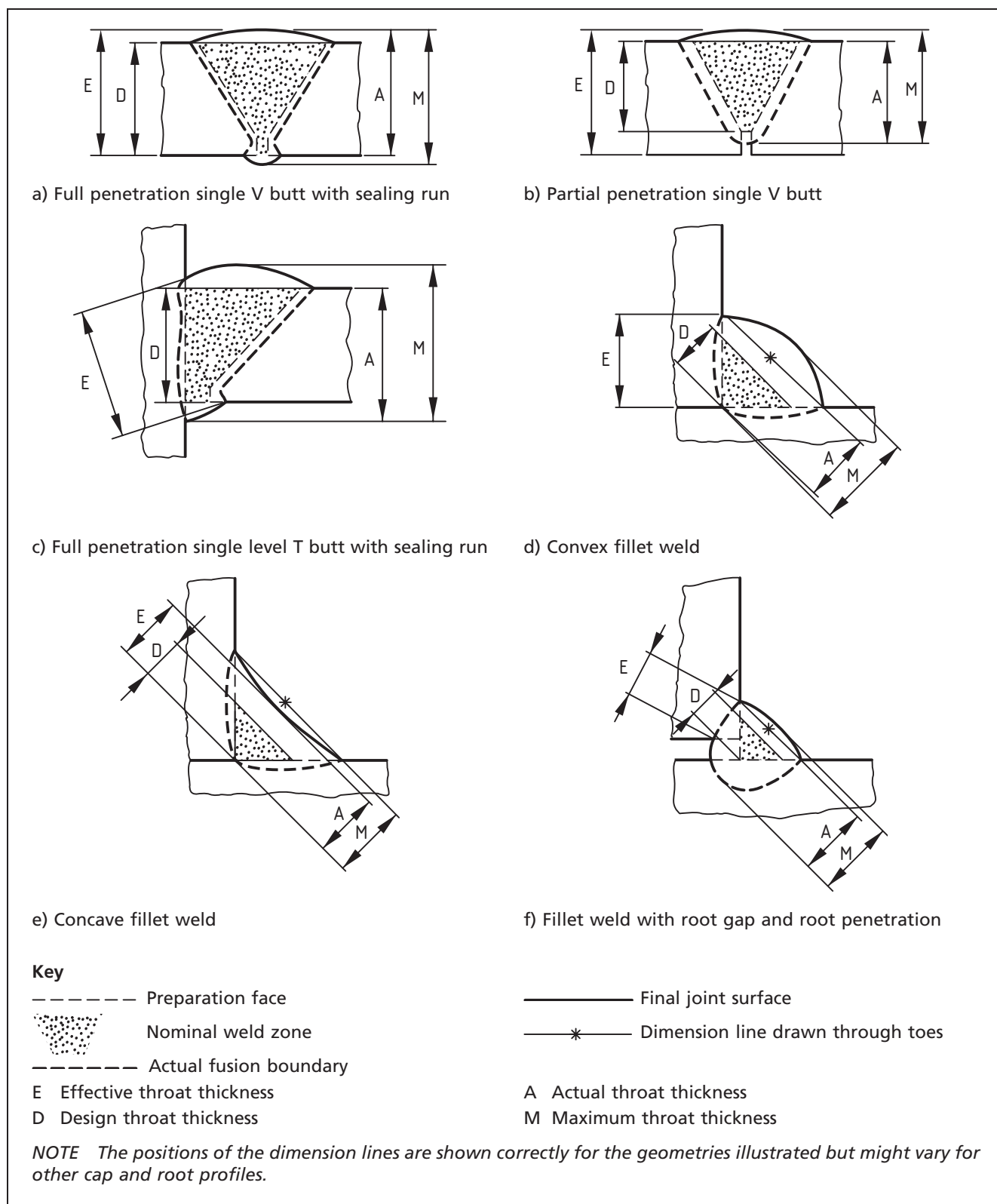
Figure 53 Examples of actual, effective, design and maximum throat thickness of typical welds
