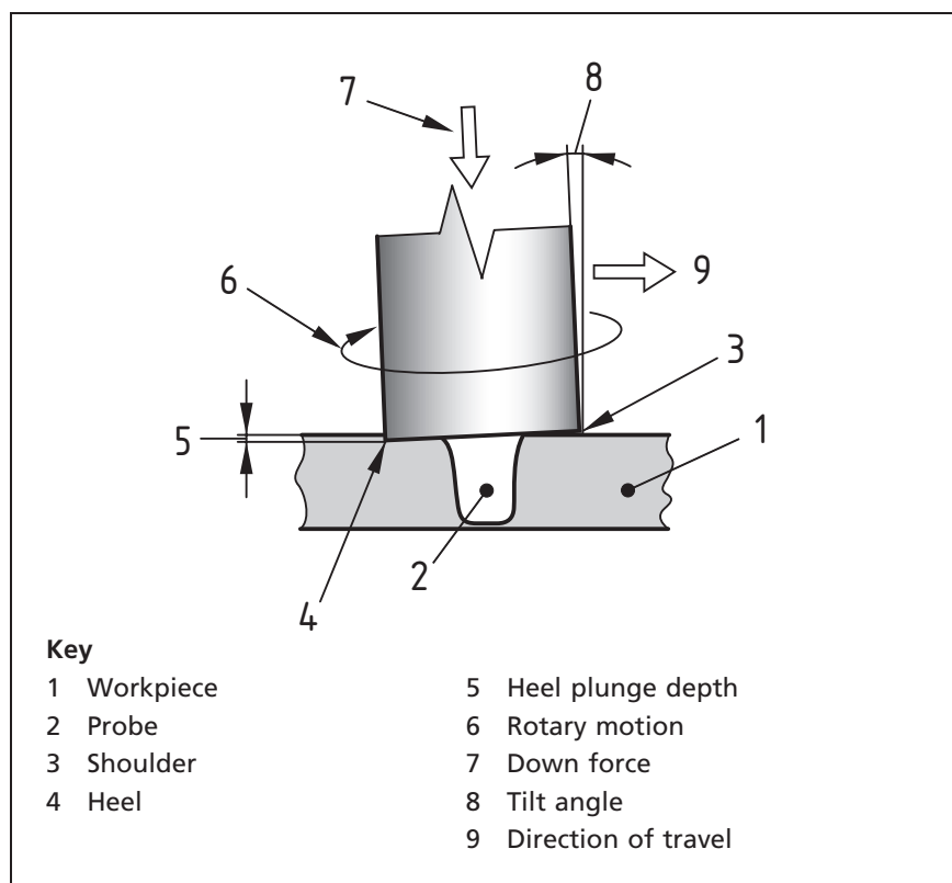
Figure 42 Heel and heel plunge depth
