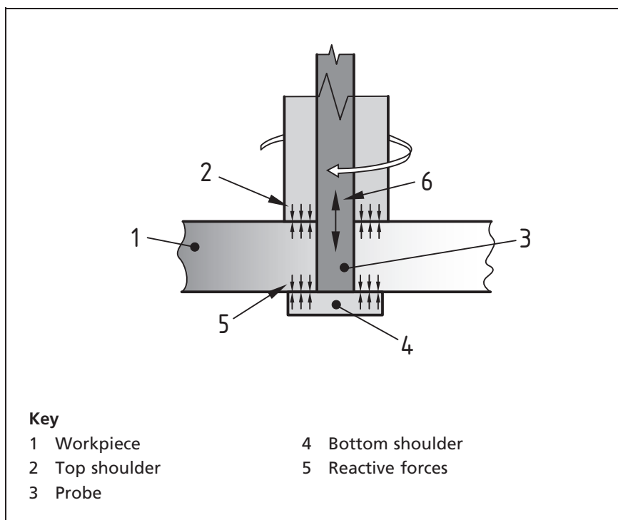
Figure 45 Self-reacting bobbin tool
