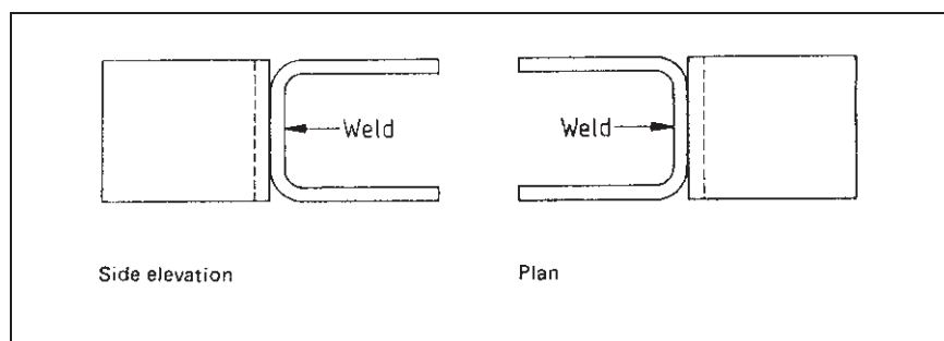
Figure 91 U-tensile test specimen
