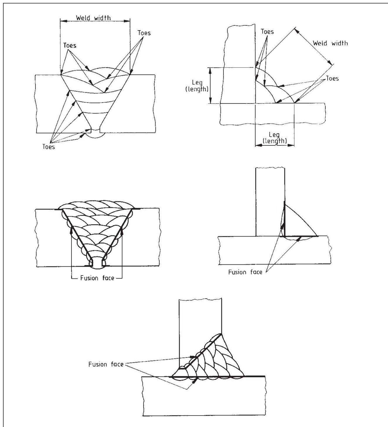
Figure 52 Examples of toes, legs, weld widths and fusion faces
