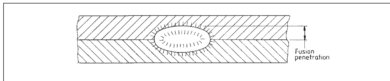
Figure 17 Weld nugget
