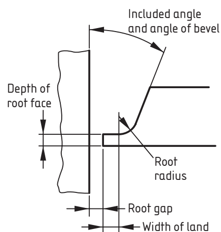
f) Single sided J T-butt
