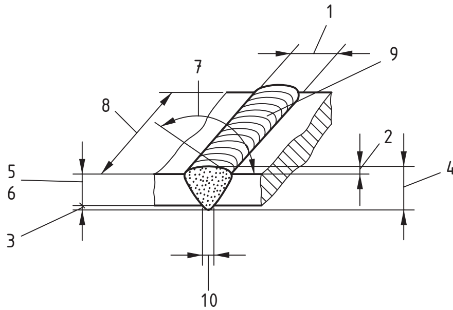
Figure 60 Typical example of butt weld – General view of butt weld
