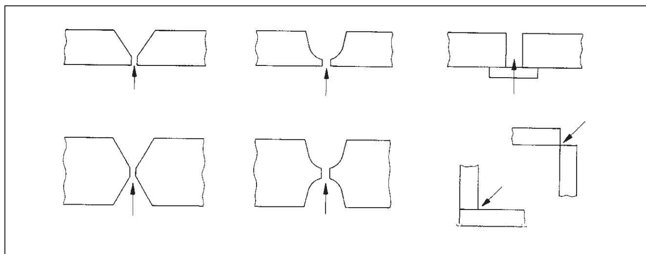
Figure 71 Roots of typical weld preparations
