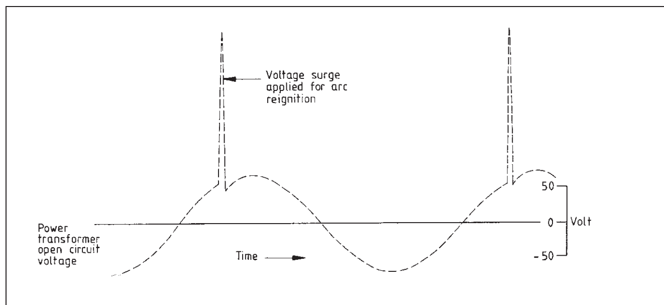
Figure 74 Surge reignition
