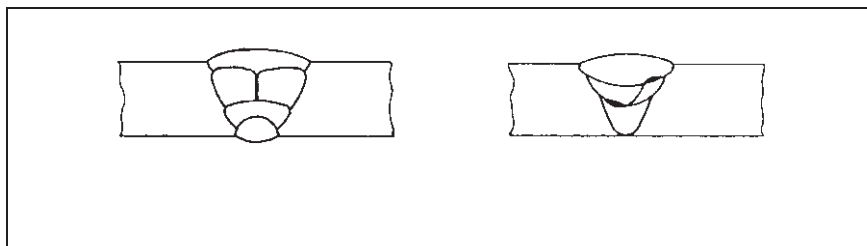
Figure 100 Lack of inter-run fusion
