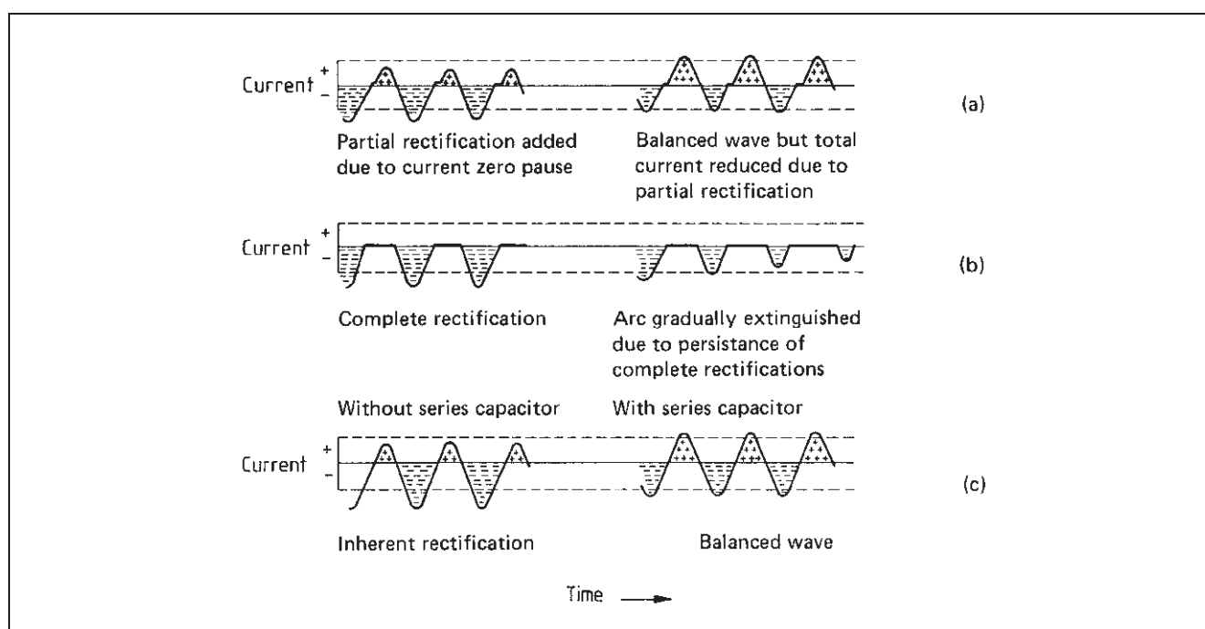
Figure 75 Types of rectification
