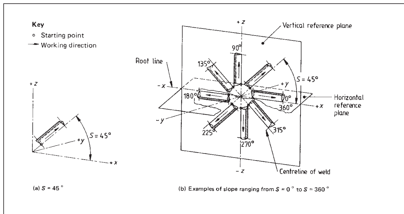
Figure 55 Welding positions: slope ( S )
