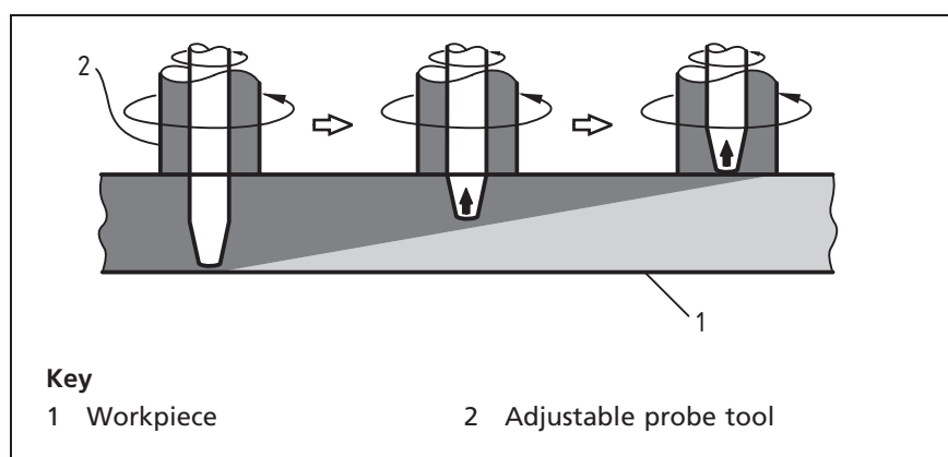
Figure 43 Adjustable probe tool
