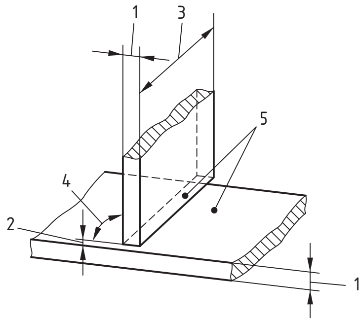
Figure 63 Preparation for fillet weld (T-joint)
