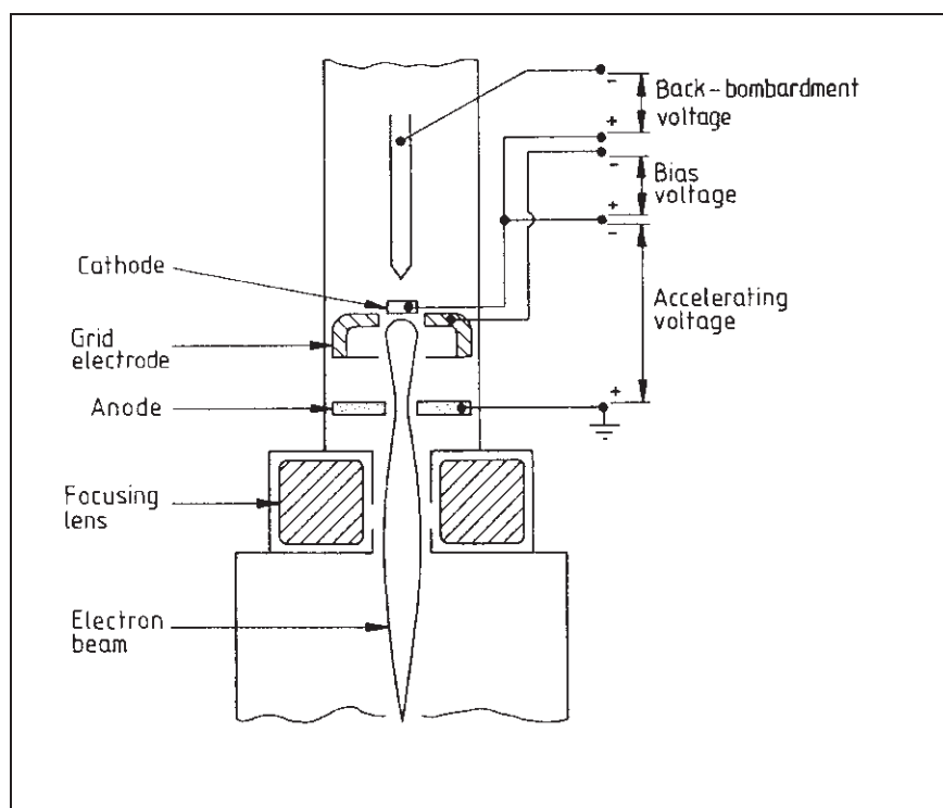
Figure 85 Diagrammatic representation of a back-bombarded gun
