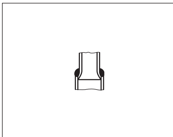
Figure 89 Diminishing bell butt joint
