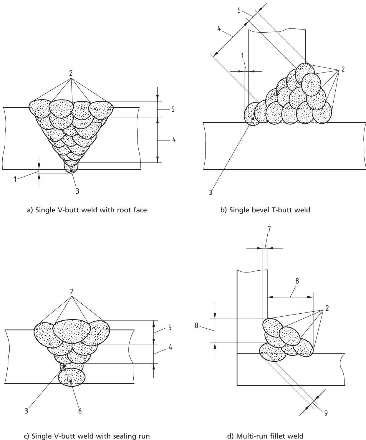
Figure 64 Typical examples of multi-run fusion welds
