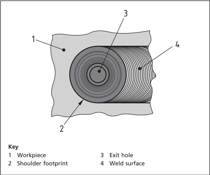
Figure 47 Tool shoulder footprint visible at the exit hole
