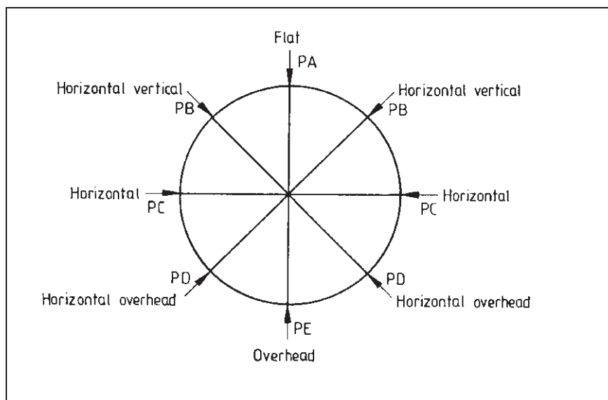
Figure 57 Simplified view of main welding positions
