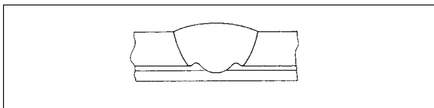
Figure 104 Shrinkage groove
