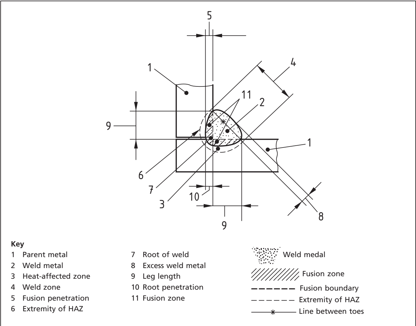
Figure 67 Typical example of fusion weld – Fillet weld
