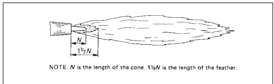
Figure 77 Carburizing oxy-acetylene flame
