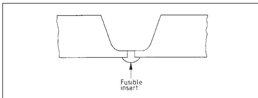
Figure 59 Weld preparation using a fusible insert
