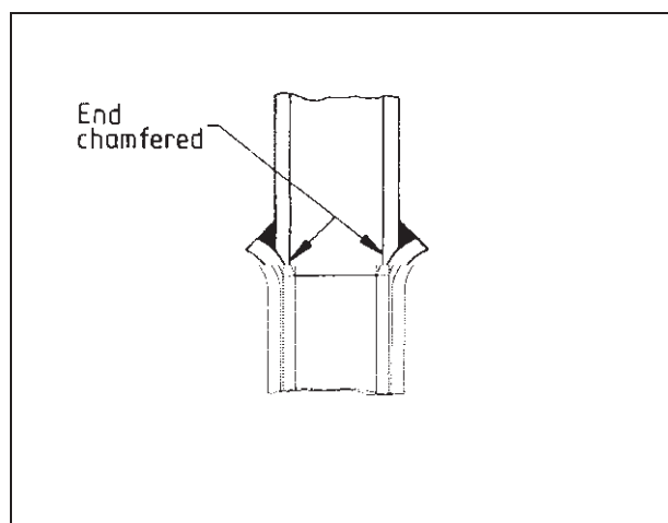
Figure 88 Bell butt joint
