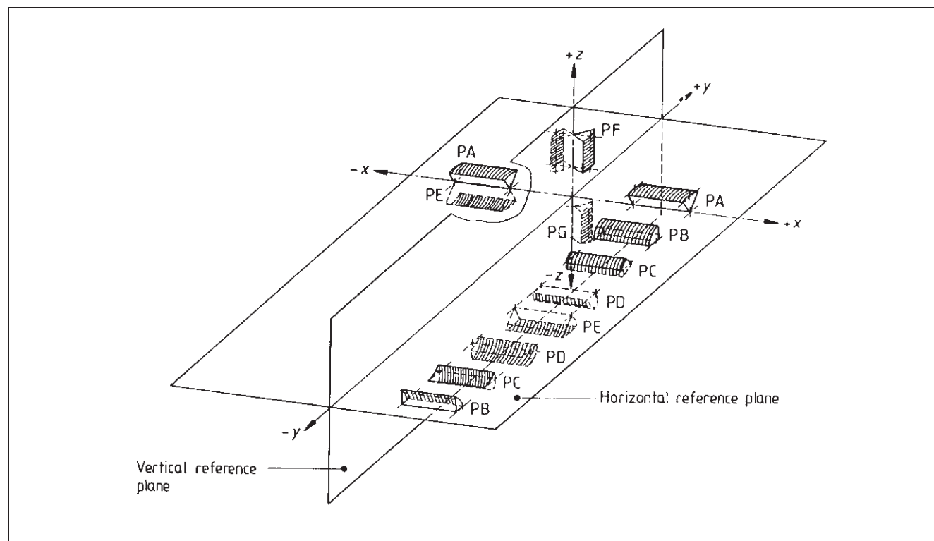
Figure 56 Schematic diagram of main welding positions
