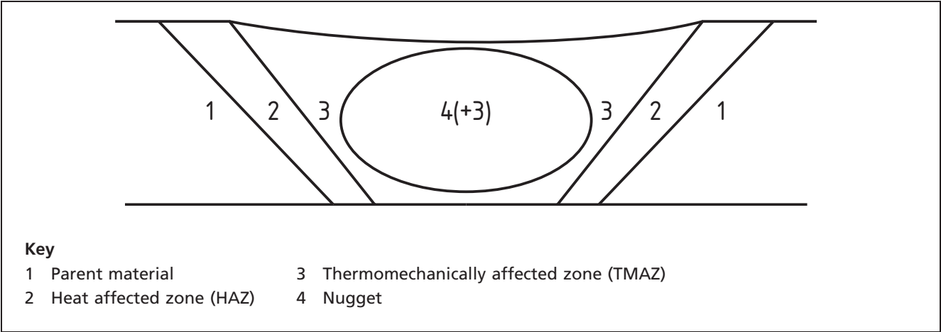
Figure 46 Cross-section of a friction stir weld
