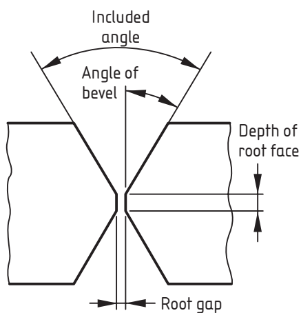
c) Double sided V-butt
