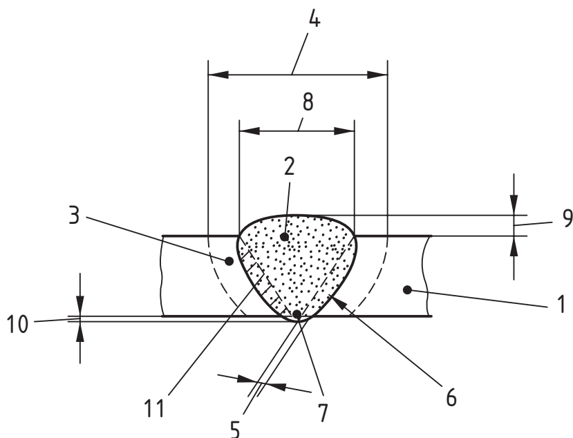
Figure 66 Typical example of fusion weld – Single V-butt weld
