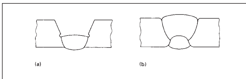
Figure 97 Undercut
