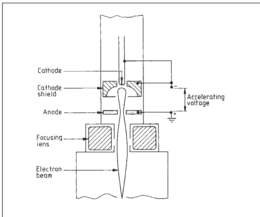
Figure 83 Diagrammatic representation of a diode gun
