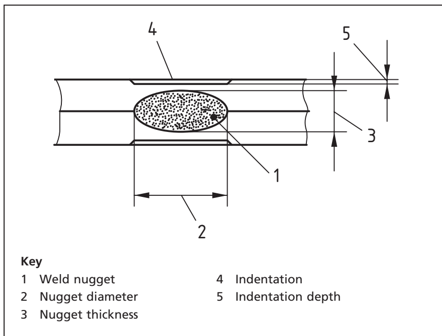
Figure 18 Typical example of weld made using pressure – Resistance spot welds
