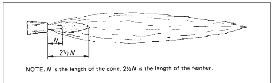
Figure 78 Carburizing oxy-acetylene flame for a hard surfacing application
