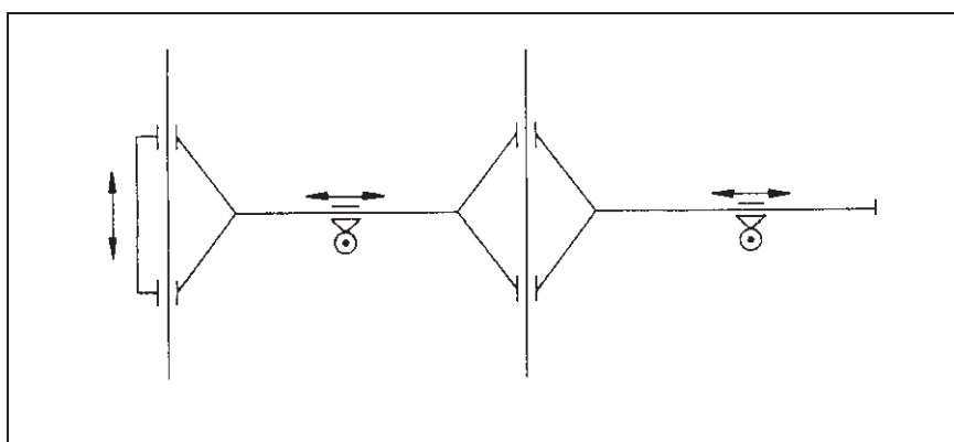
Figure 111 Portal-cantilever cutting machine
