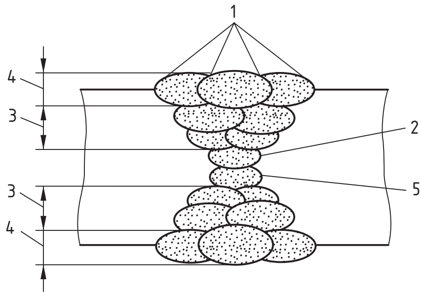
Figure 62 Typical example of multi-run fusion weld – Double V-butt weld
