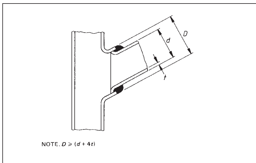
Figure 90 Short bell branch joint
