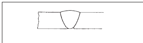
Figure 99 Lack of root fusion
