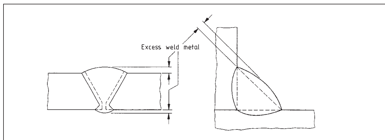
Figure 54 Examples of excess weld metal
