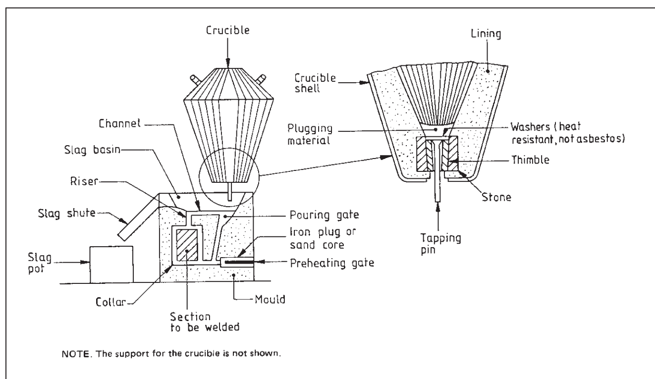
Figure 86 Basic equipment for aluminothermic welding
