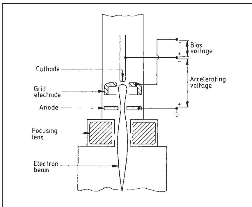
Figure 84 Diagrammatic representation of a triode gun
