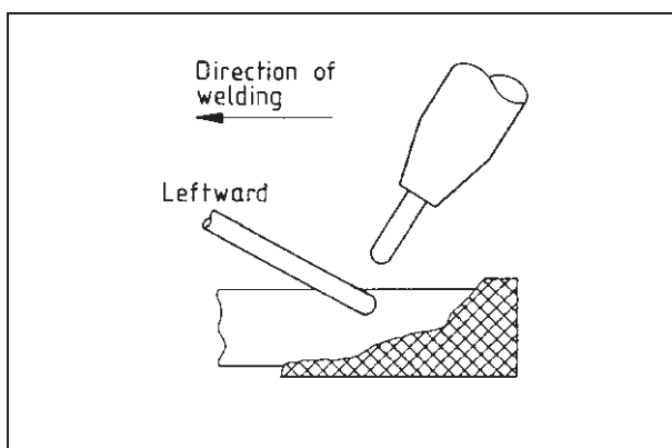
Figure 80 Leftward welding
