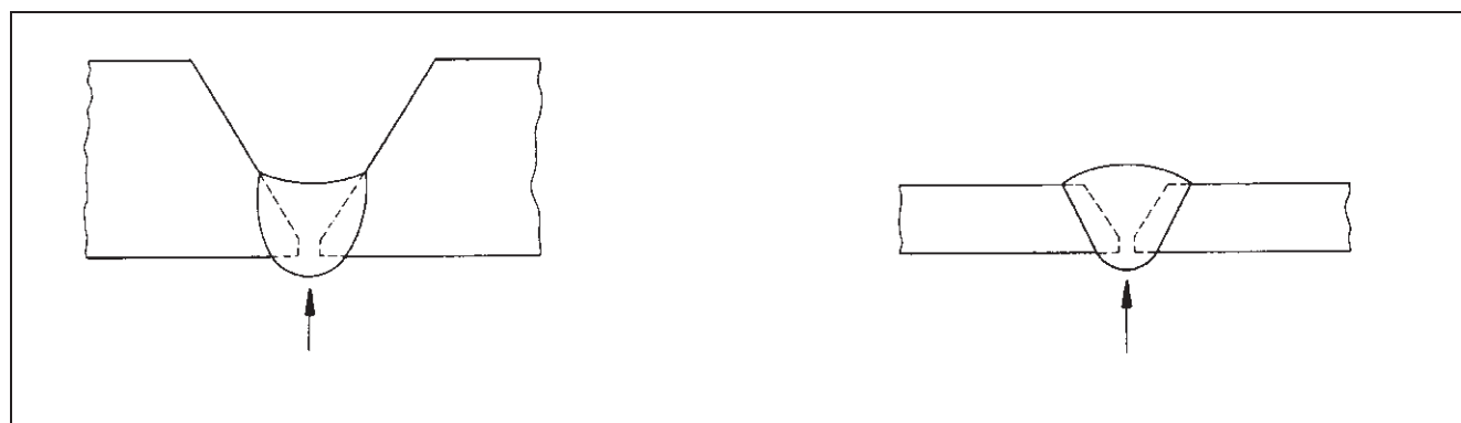
Figure 72 Penetration bead
