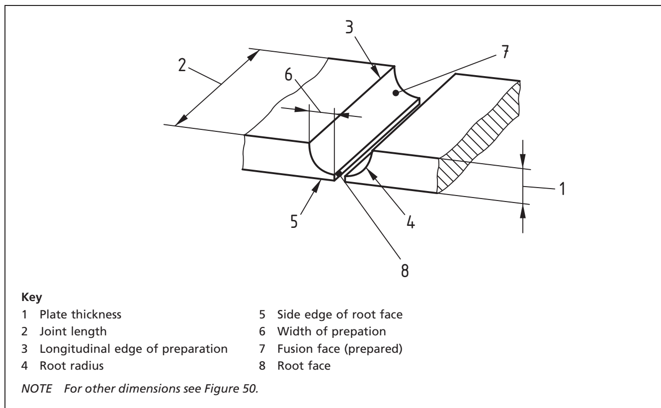
Figure 65 Preparation for single U-butt weld
