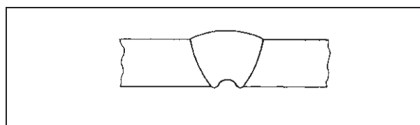
Figure 103 Root concavity
