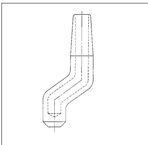
Figure 39 Swan-necked electrode
