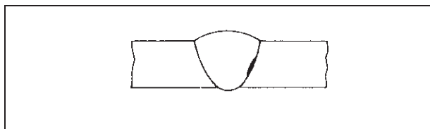
Figure 98 Lack of sidewall fusion
