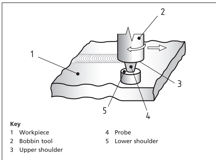
Figure 44 Fixed bobbin tool
