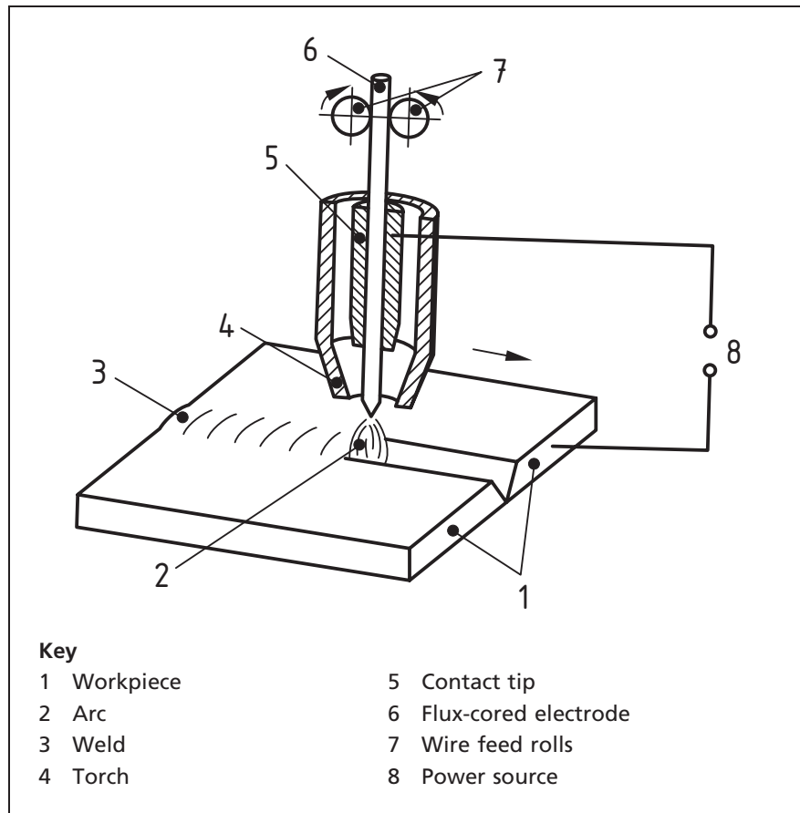
Figure 73 Self-shielded tubular-cored arc welding
