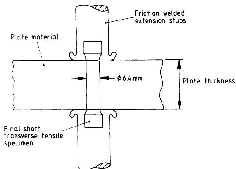
Figure 10 — Short transverse tensile test specimen with friction welded extensions
