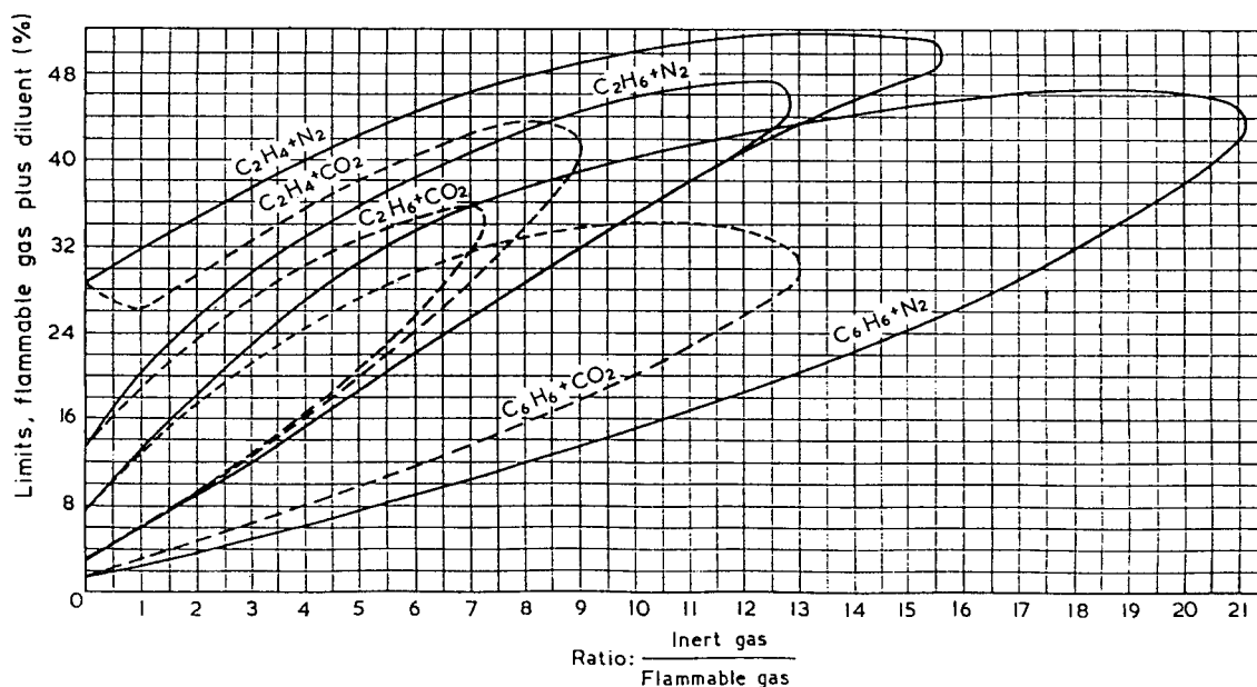
Figure 2 — Flammable limits of ethane, ethylene and benzene containing various amounts of carbon dioxide and nitrogen
