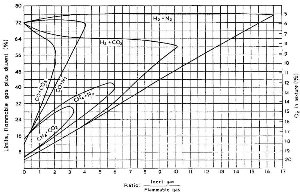
Figure 1 — Flammable limits of hydrogen, carbon monoxide and methane containing various amounts of carbon dioxide and nitrogen
