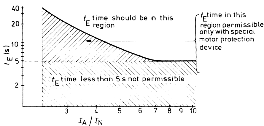
Figure 1 — Minimum t_E time for motors in relation to I_A/I_N
