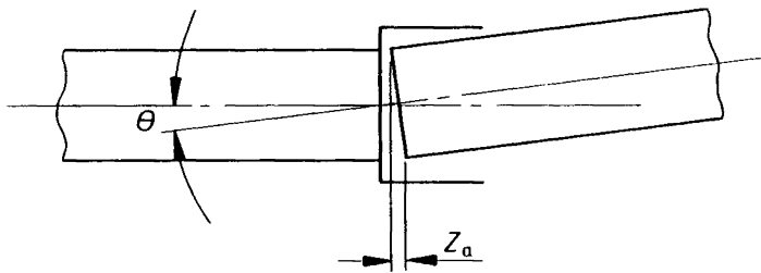
NOTE Angular deflection causes a longitudinal movement Z_a . Figure 7 — Angular deflection
