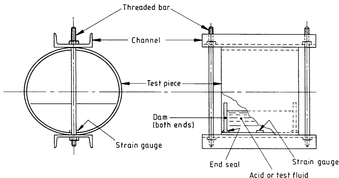
Figure 5 — Diagrammatic representation of apparatus for strain corrosion testing
