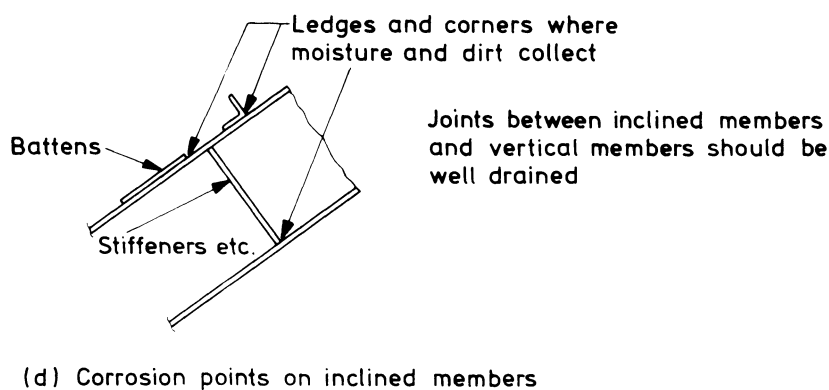
Figure 2 — Corrosion points
