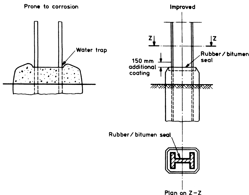
Figure 6 — Protection of a stanchion at ground level
