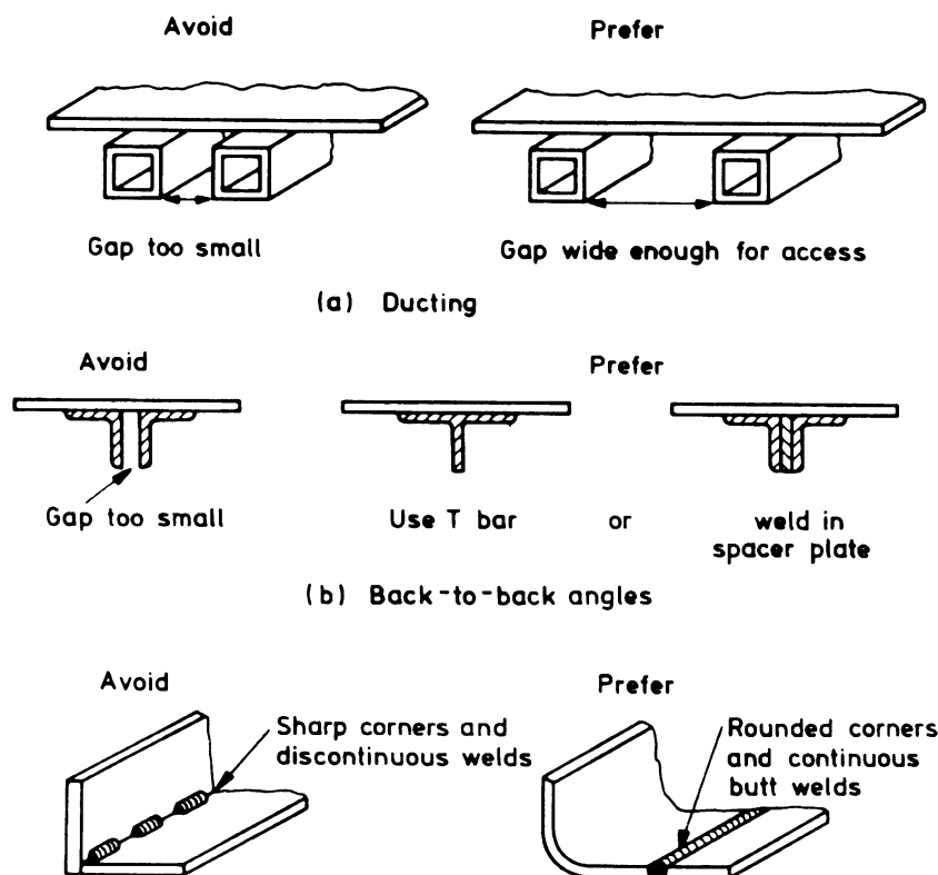
Figure 8 — Design for coating
