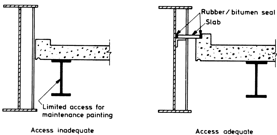
Figure 9 — Access for maintenance
