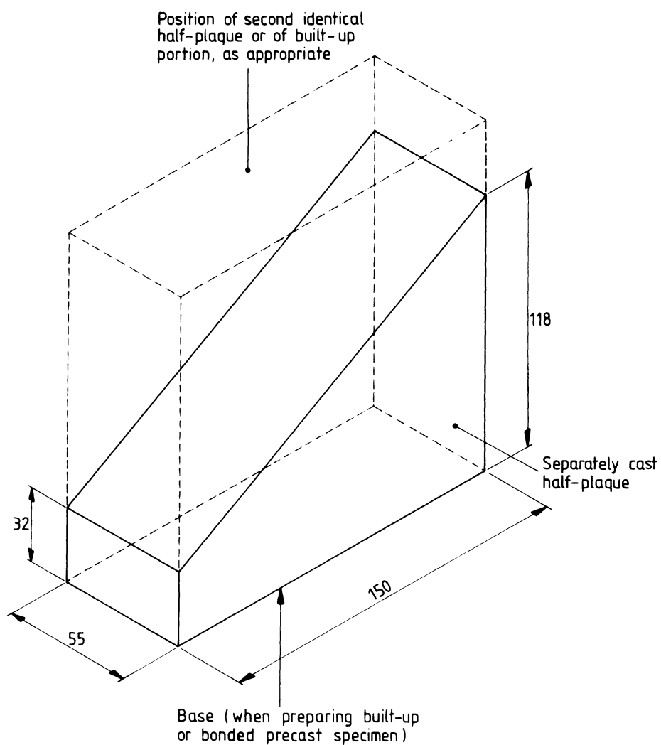
Figure 3 — Dimensions of cast half-plaques used for preparation of built-up or bonded test specimens
