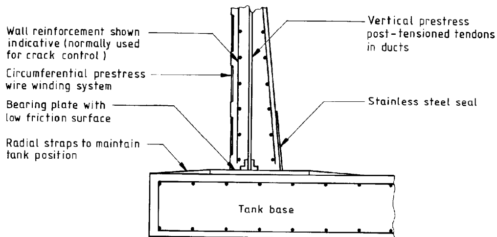
a) Sliding joint
