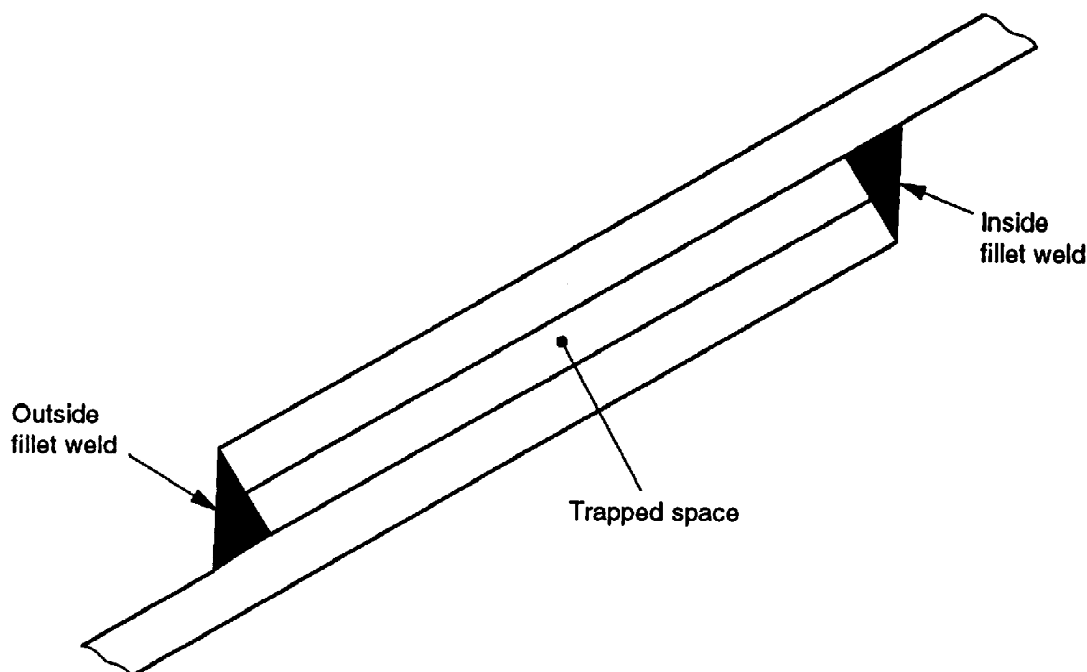
Figure 1. Detail of lap welded inner roof
