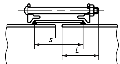
Figure C.4 — Slip-on type couplings
