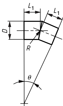
Figure 3 — Gusseted bend type 1, \theta \leq 30^\circ
