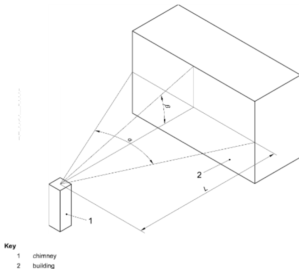
Figure C.1 — Chimney outlet position (see text)
