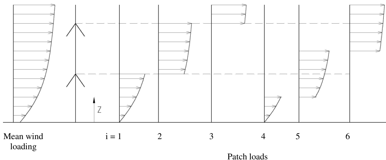
Figure B.4.1 Application of patch loads
