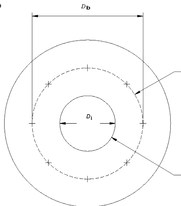
Figure 6.1 Bolted flanged connections
