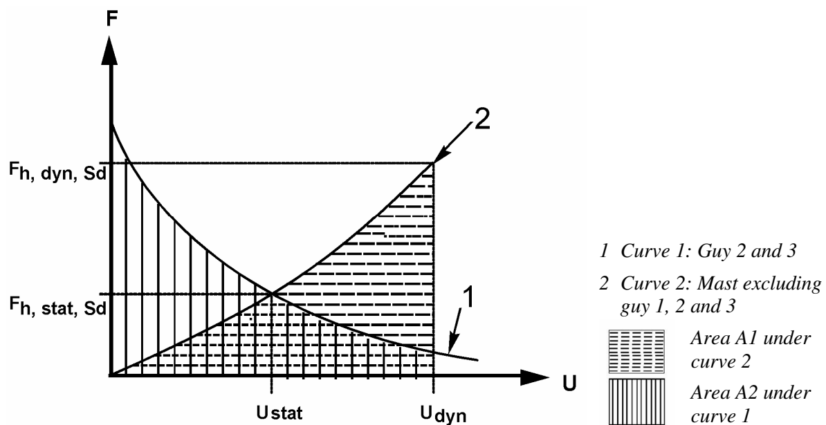
Figure E.2 Force-deflection diagram
