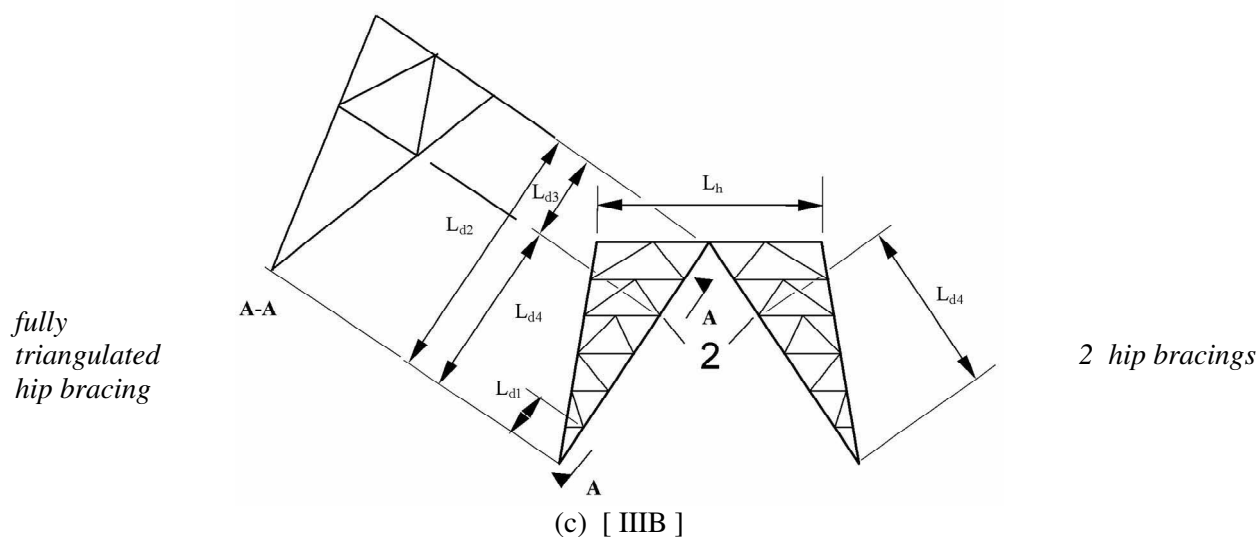
(c) [ IIIB ] Figure H.2 Use of secondary bracing systems
