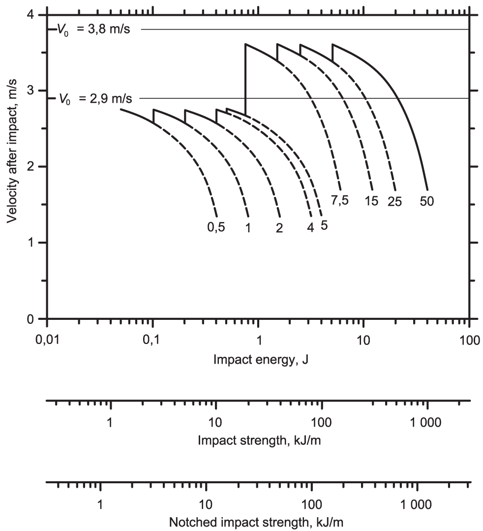
Figure E.1 — Pendulum velocity after impact as a function of impact energy, impact strength, and notched impact strength for Charpy impact testing
