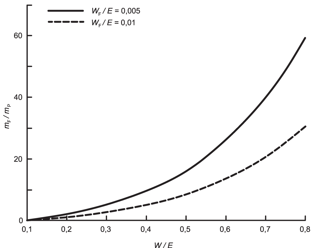
Figure D.1 — Ratio of mass of frame to mass of pendulum plotted against the relative energy uptake by the specimen W/E for two values of the relative energy uptake by the frame W_F/E
