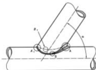
Figure 7 — Location of test specimens for a T-joint
