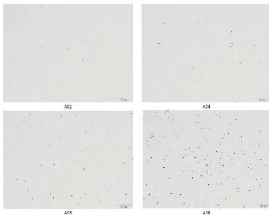
Figure 2 — A-type porosity classes at \times 200 magnification (optical)
