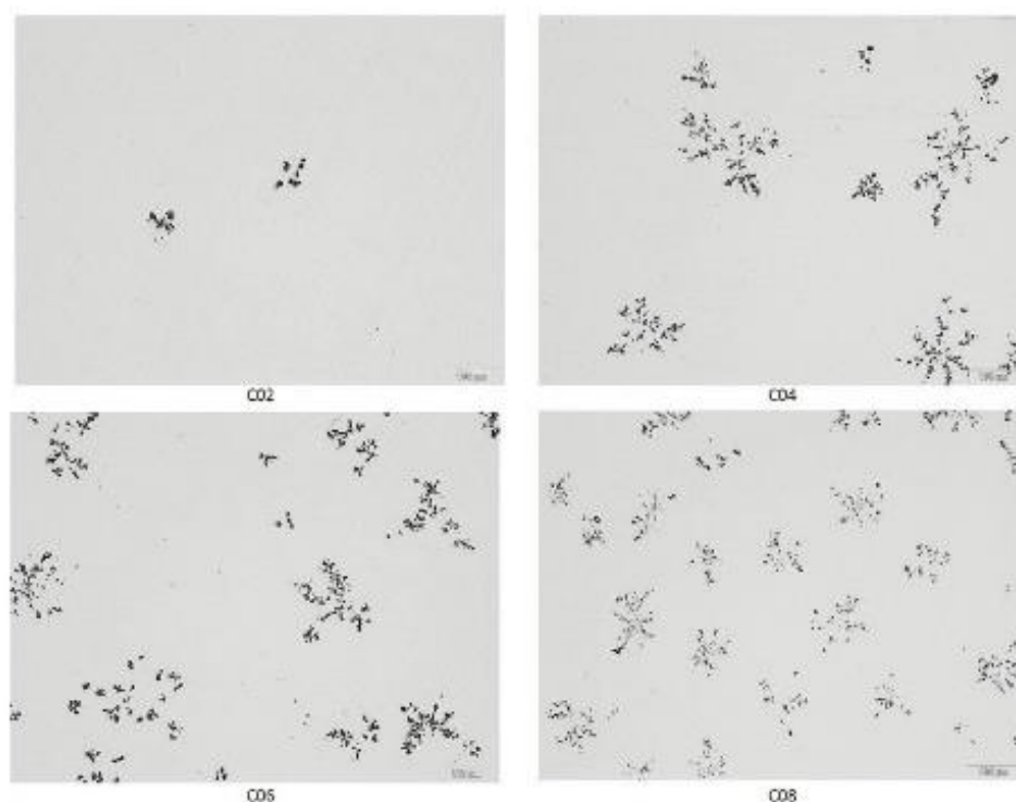
Figure 4 — Carbon porosity at \times 100 magnification (optical)
