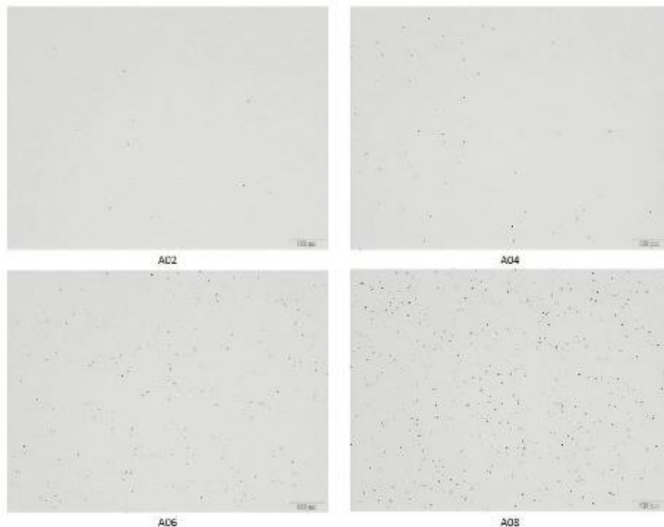
Figure 1 — A-type porosity classes at \times 100 magnification (optical)
