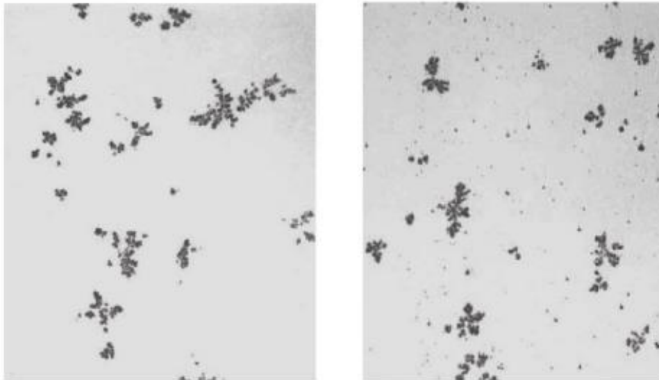
Figure 5 — Large eta-phase rosettes (about 100 \mu\text{m} in diameter)
