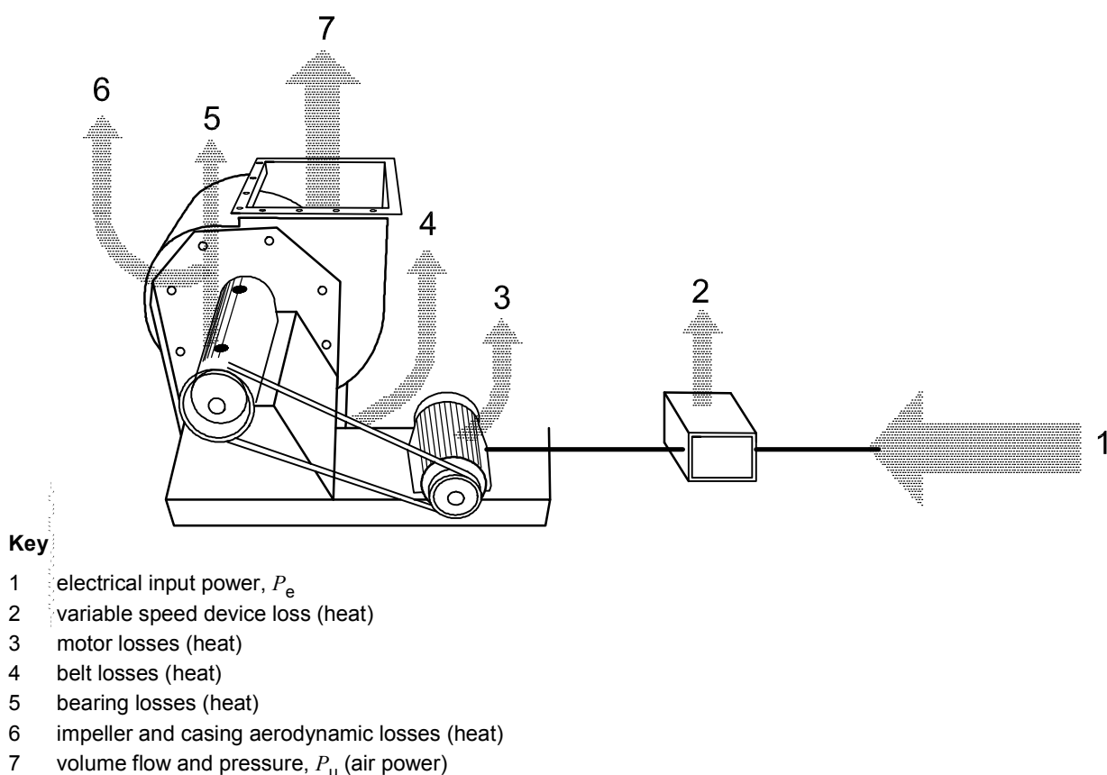
Figure E.1 — Typical belt-driven fan showing power losses
