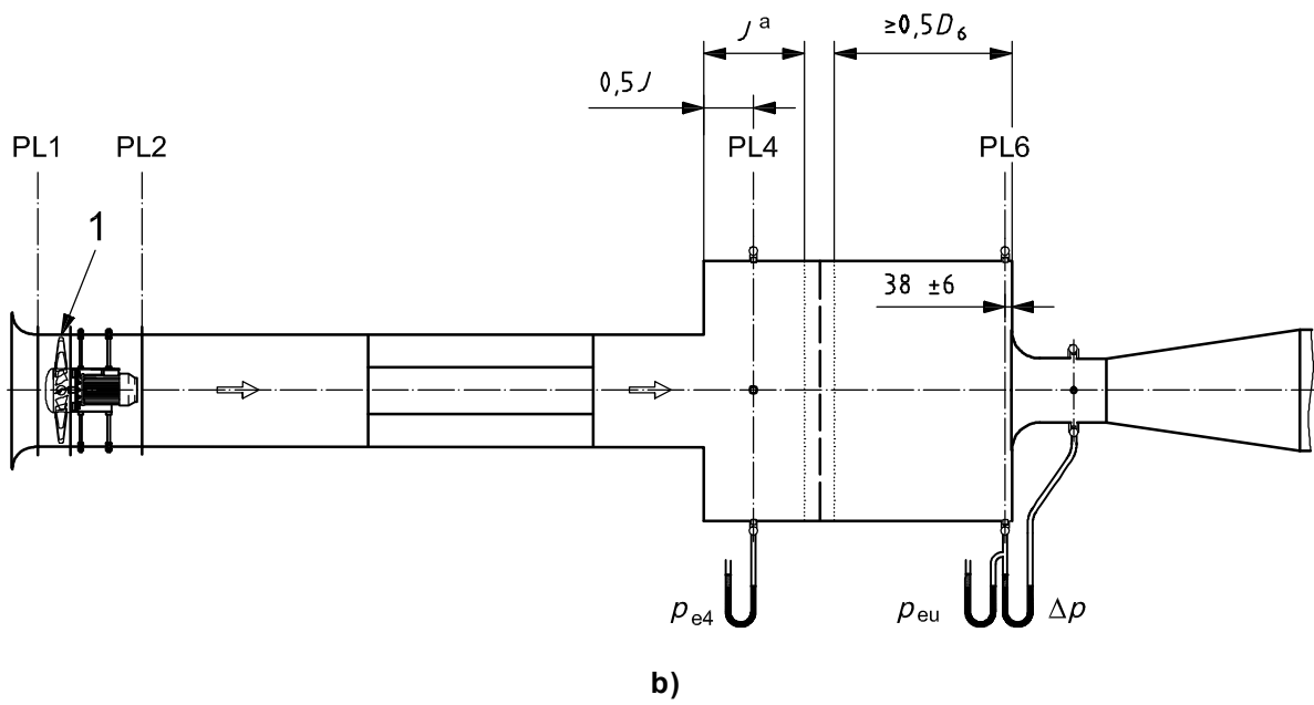
Figure 39 — Outlet-side test chambers
