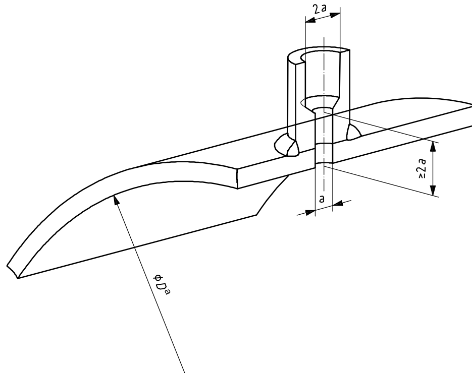
Figure 2 — Construction of wall pressure tapplings
