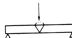
e) Fracture testing, root side
