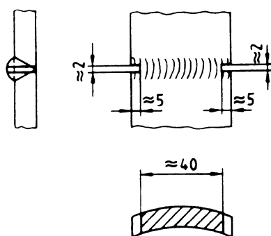
c) Inspection length of the test specimen
