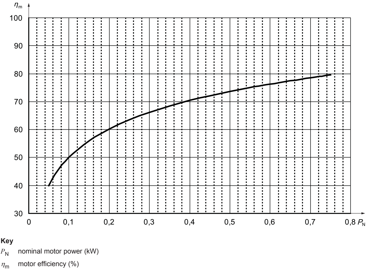
Figure B.1 — Default efficiency values for motors below 0,75 kW
