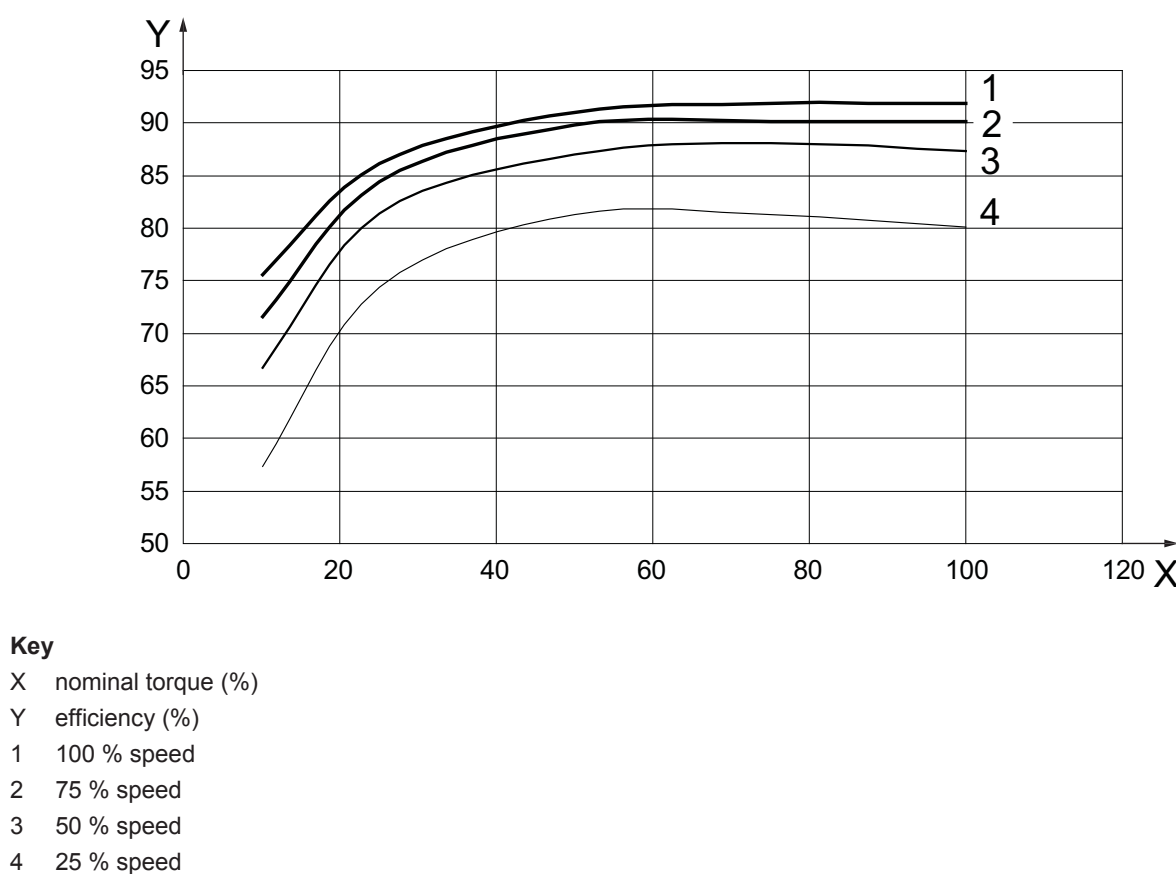
Figure D.3 — Efficiency of a typical motor at various loads
