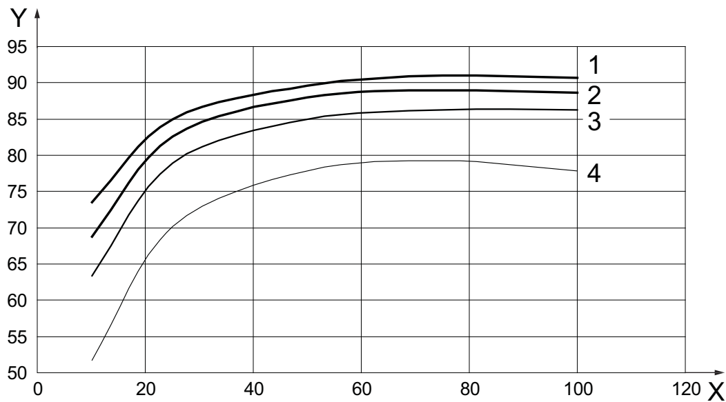
Key X nominal torque (%) Y efficiency (%) 1 100 % speed 2 75 % speed 3 50 % speed 4 25 % speed
