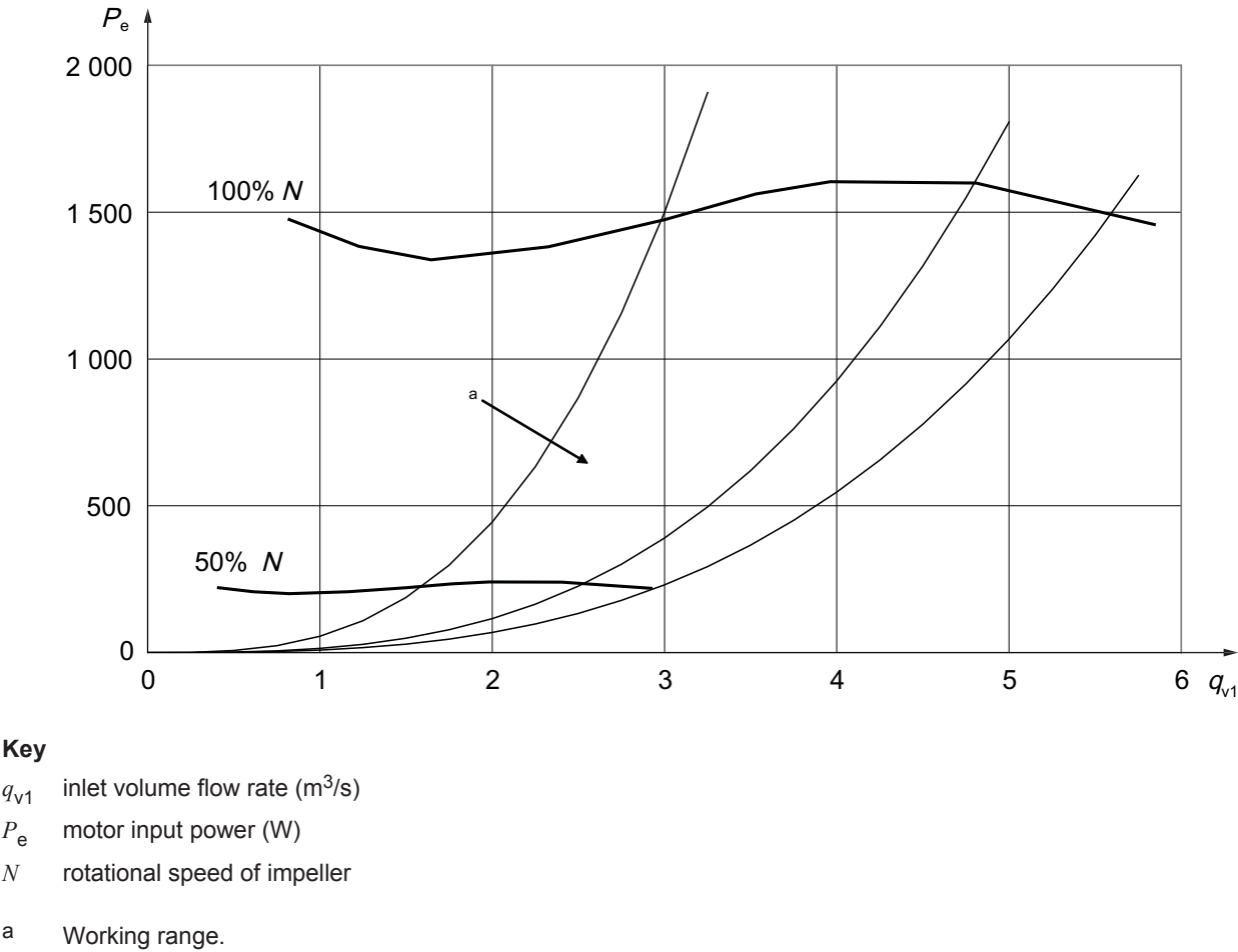
Figure E.2 — Fan input power characteristic
