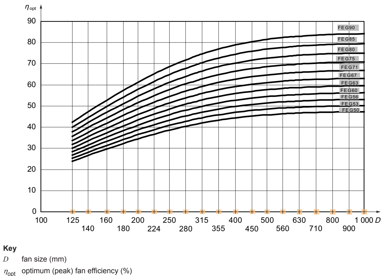
Figure 4 — FEG for bare shaft fans
