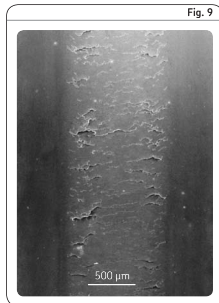
Initial spalling resulting from surface initiated fatigue on the inner ring raceway of a deep groove ball bearing
