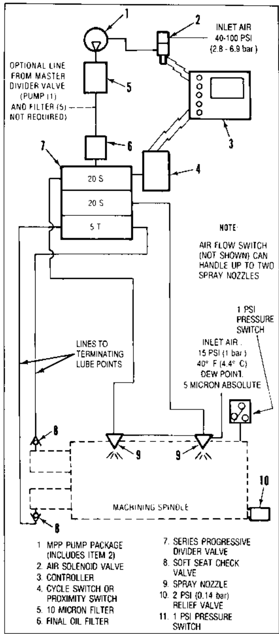
FIG. 13-23 Control of advanced oil mist system with flow dividers (reprinted with permission of Lubriquip).
