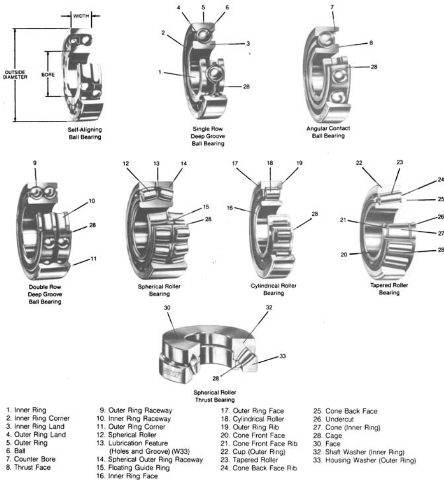
FIG. 12-1 Bearing types and terminology (with permission from SKF).
