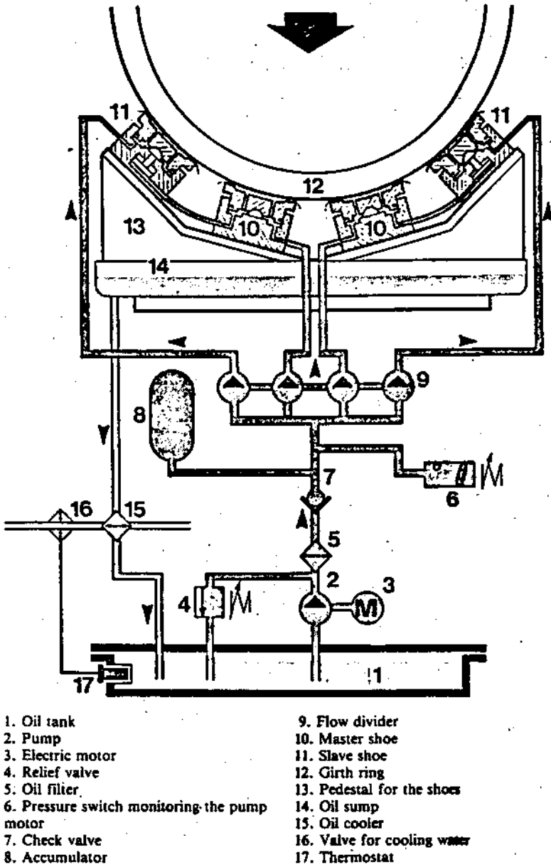
FIG. 10-15 Hydraulic system for hydrostatic pad shoes. (From Trygg and McIntyre (1982), reprinted with permission from CIM Bulletin.)
