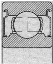
FIG. 13-29f Bearing with shields (from FAG, 1998, with permission).
