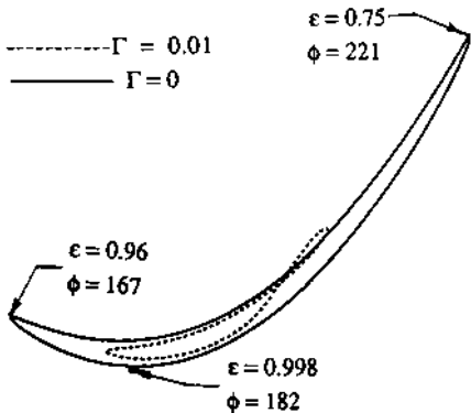
FIG. 15-2 Locus of the journal center for the load F_t = 800 + 800 \sin 2\omega t and journal mass \bar{m} = 100 .
