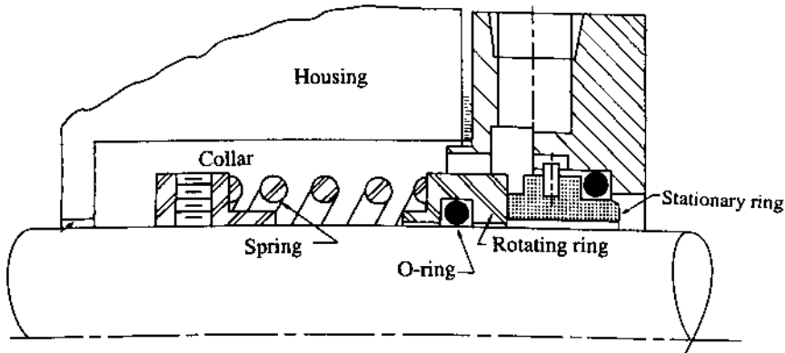
FIG. 13-30 Mechanical seal.
