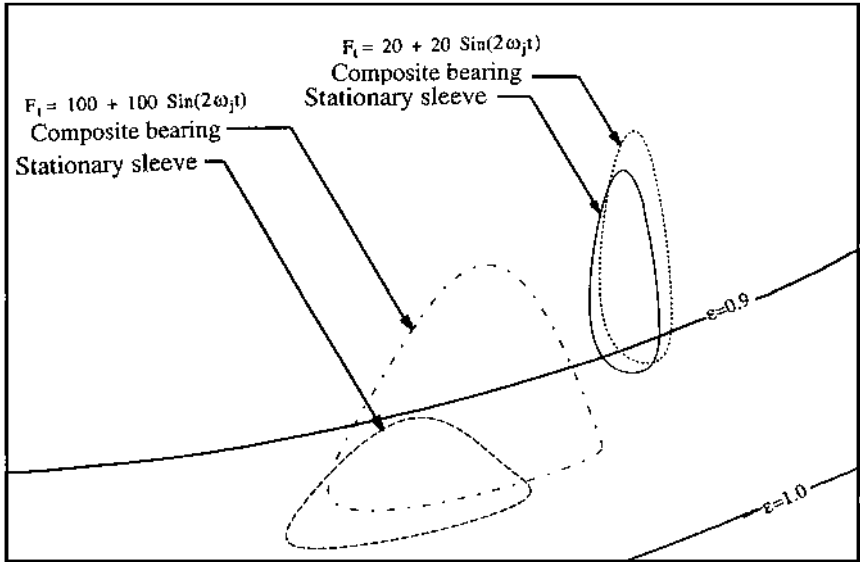
FIG. 18-9 Journal loci of a regular bearing and a composite bearing; F(t) = 100 + 100 \sin(2\omega_j t) and F(t) = 20 + 20 \sin(2\omega_j t) . The journal mass is m = 50 . The design parameters are H_1 = 0.1 and H_2 = 1.0 .
