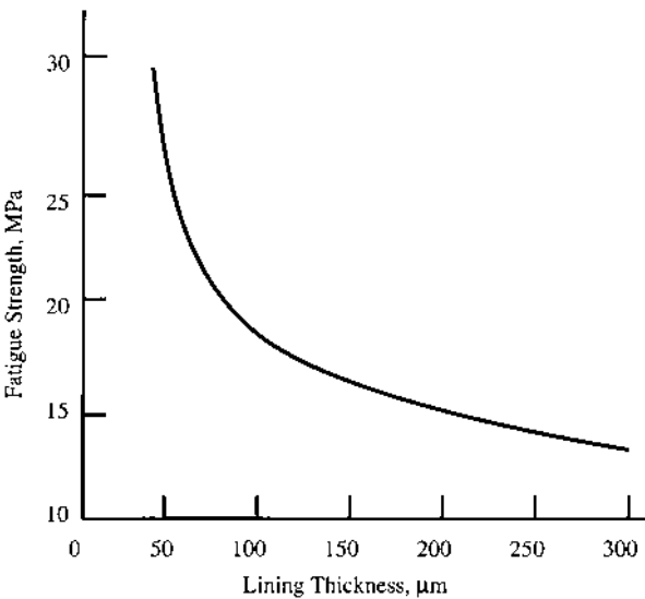
FIG. 11-1 Fatigue resistance as a function of white metal thickness.
