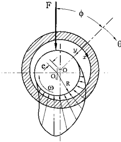
FIG. 6-1 Hydrodynamic journal bearing (clearance exaggerated).
