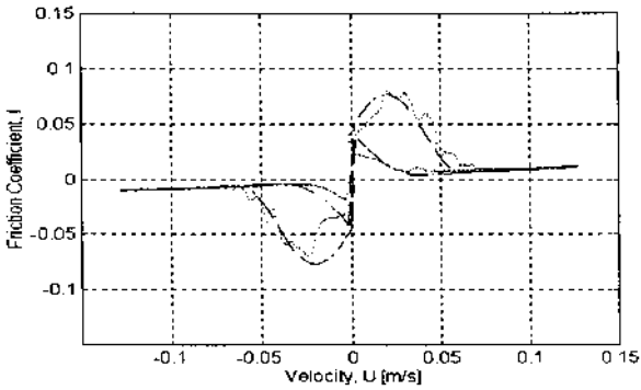
FIG. 17-5 Comparison of measured and theoretical f - U curves for sinusoidal sliding velocity: load = 84 N, U = 0.127 \sin(0.25t) m/s, oscillation frequency = 0.25 rad/s (measurement . . . , simulation —).
