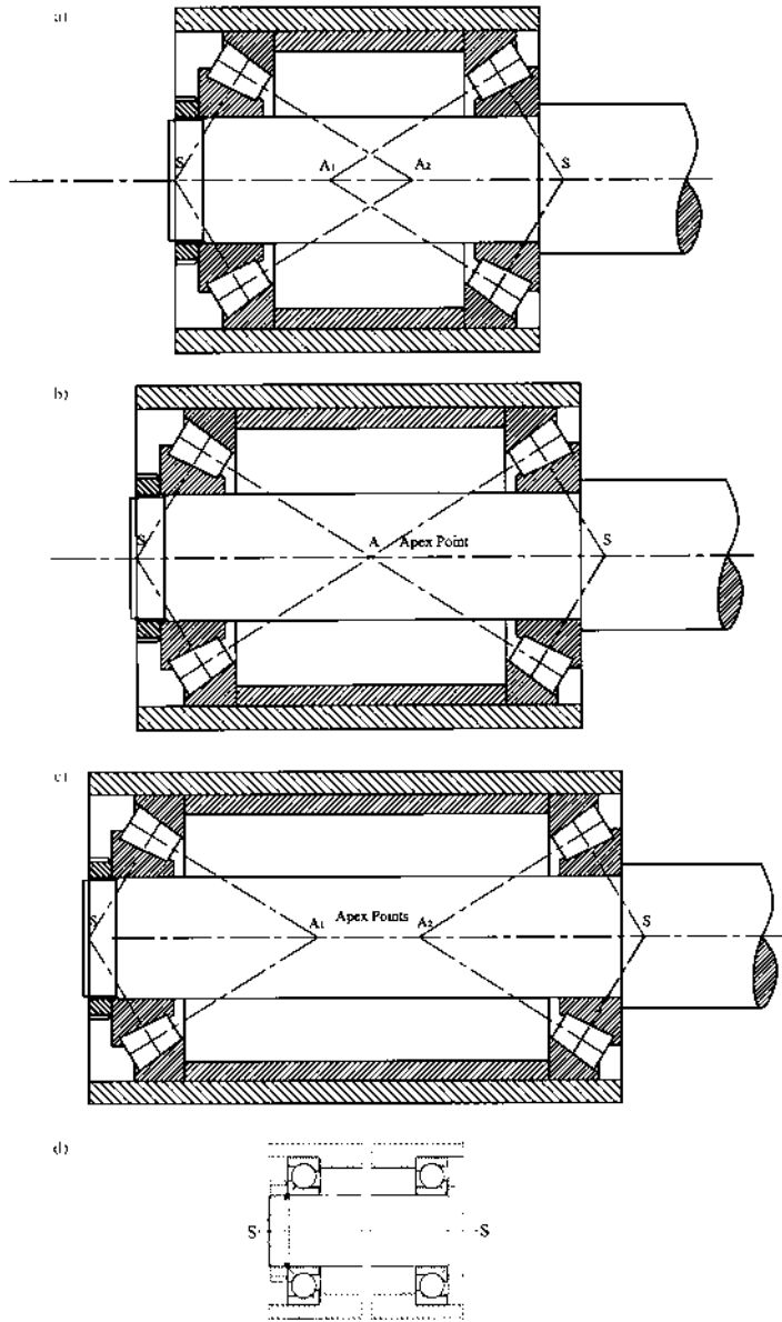
FIG. 13-9 (a) Adjustable arrangement, apex points between the bearings overlap. (b) Adjustable arrangement, apex points coincide between the two bearings. (c) Adjustable arrangement, apex points apart between the bearings. (d) Similar adjustable arrangements for angular contact bearings.
