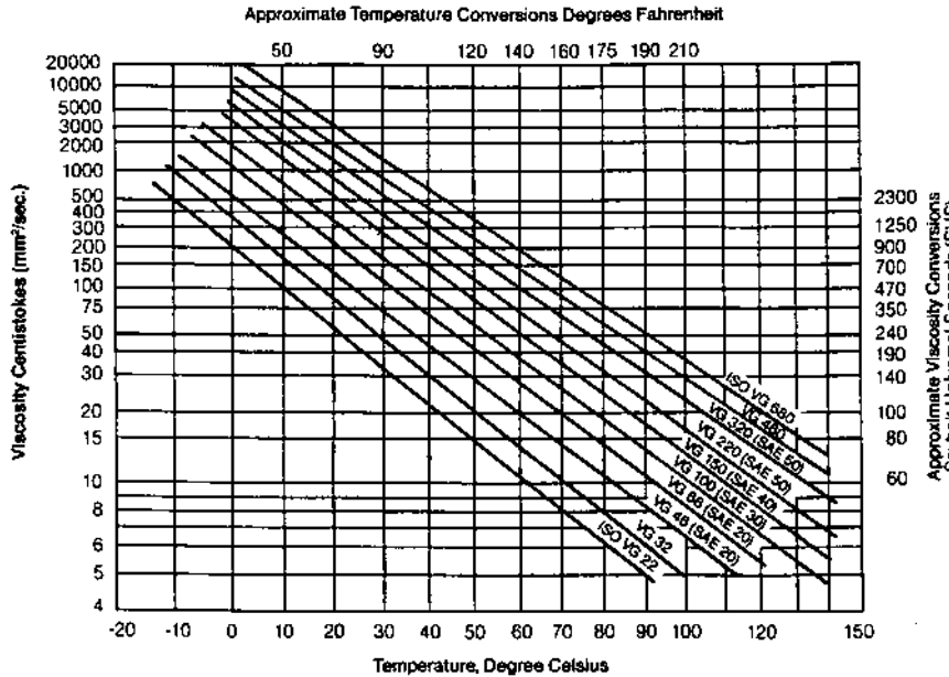
FIG. 13-2 Viscosity–temperature charts (from SKF, 1992, with permission).
