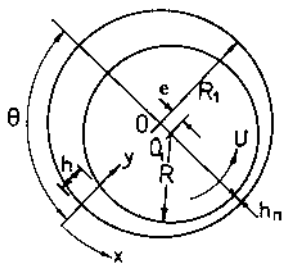
FIG. 4-1 Coordinates of a long journal bearing.
