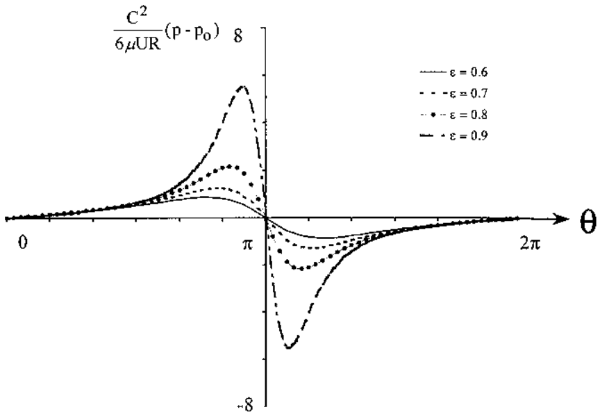
FIG. 6-4 Pressure waves in an infinitely long, full bearing according to the Sommerfeld solution.
