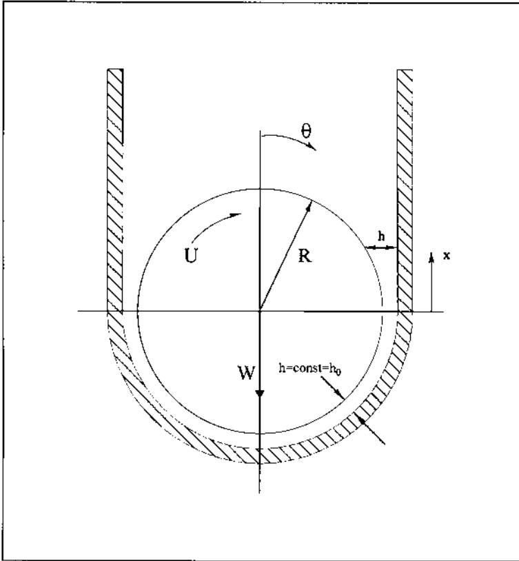
FIG. 9-5 Foil bearing.
