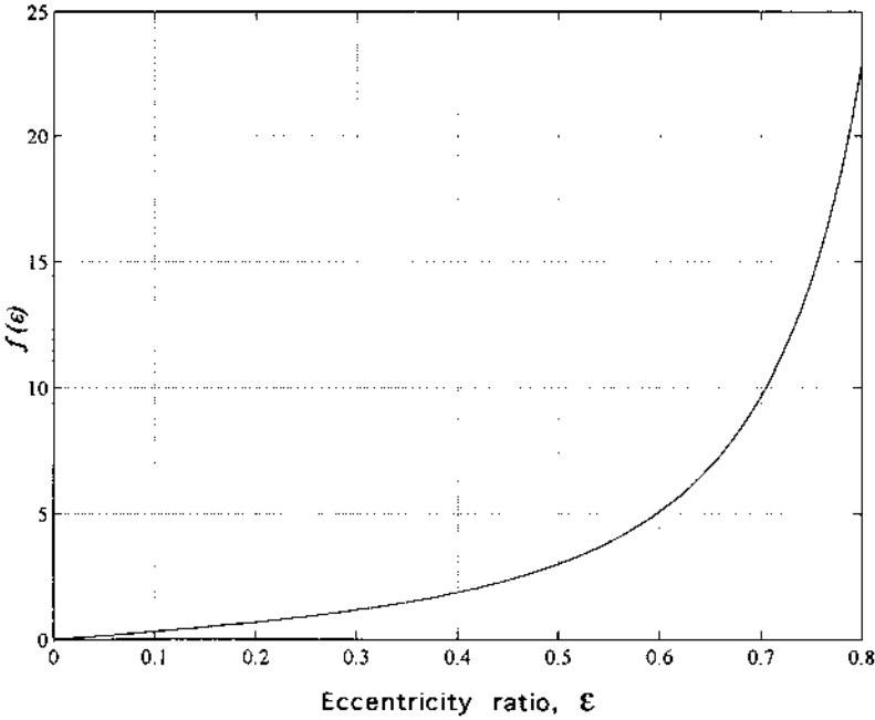
FIG. 7-3 Graph of f(\epsilon) vs. \epsilon , describing Eq. (7-33).
