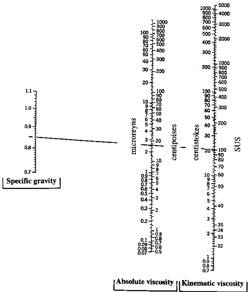
FIG. 2-2 Viscosity conversion chart from Saybolt universal seconds.
