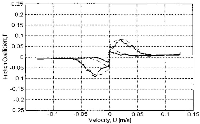
FIG. 17-2 Comparison of measured and theoretical f - U curves for sinusoidal sliding velocity: load = 104 N, U = 0.127 \sin(0.25t) m/s, oscillation frequency = 0.25 rad/s (measurement . . . , simulation —).
