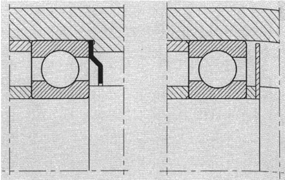
FIG. 13-29e Baffle plates seal (from FAG, 1998, with permission).
