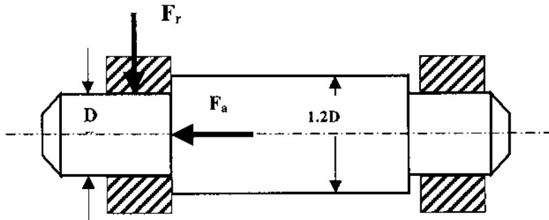
FIG. 1-6 Journal bearing under radial and thrust load.
