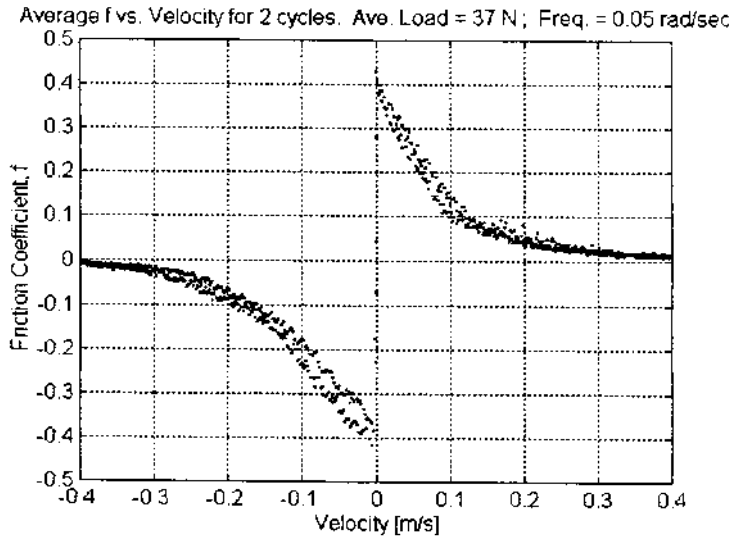
FIG. 16-2 f - U curve for sinusoidal velocity: oscillation frequency = 0.05 rad/s, load = 37 N, 25-mm journal, L/D = 0.75 , low-viscosity oil, \mu = 0.001 \text{ N}\cdot\text{s}/\text{m}^2 , no additives, steel on brass.
