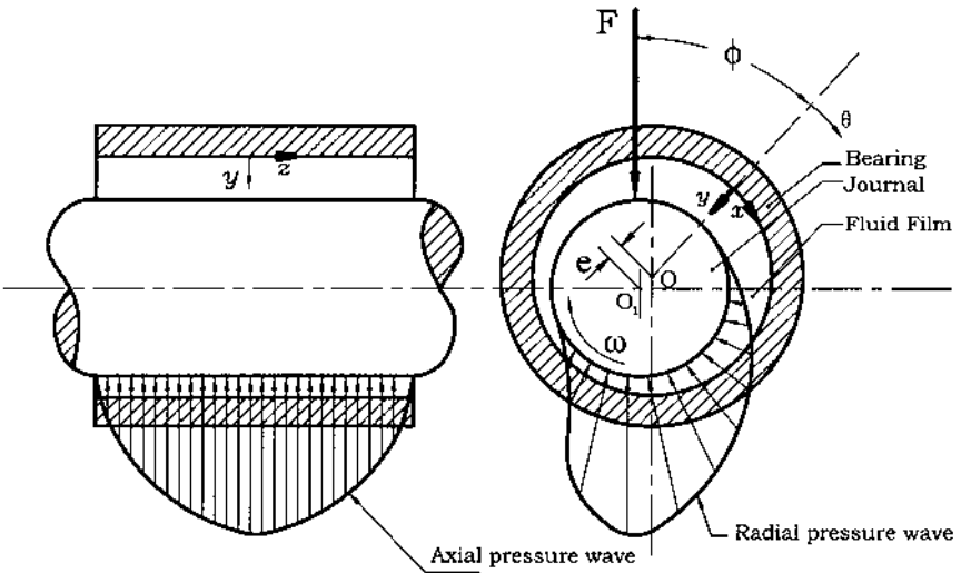
FIG. 1-3 Hydrodynamic journal bearing.
