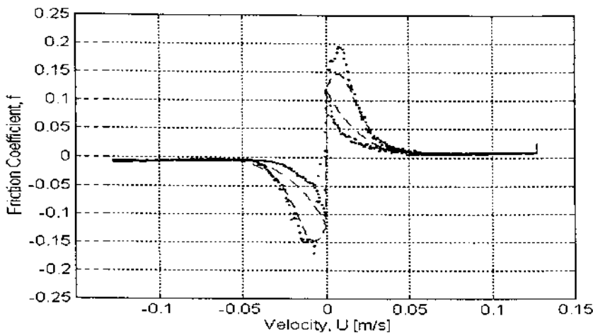
FIG. 17-1 Comparison of measured and theoretical f – U curves for sinusoidal sliding velocity: load = 104 N, U = 0.127 \sin(0.045t) m/s, oscillation frequency = 0.045 rad/s (measurement . . . , simulation —).
