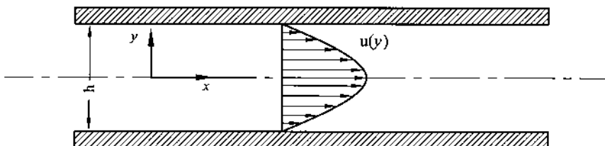
FIG. 4-6 Flow between two parallel plates.
