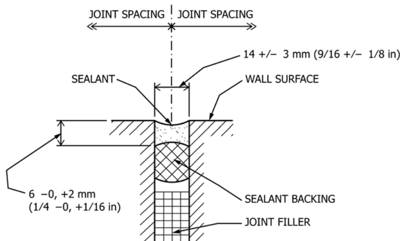
FIG. 9 Cross-Section of a Typical Butt Sealant Joint
