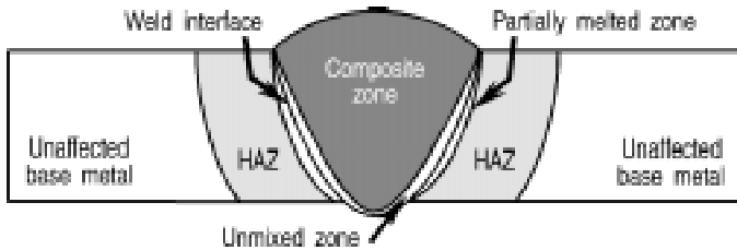
Figure 2.2 Metallurgical designations in weld zones
