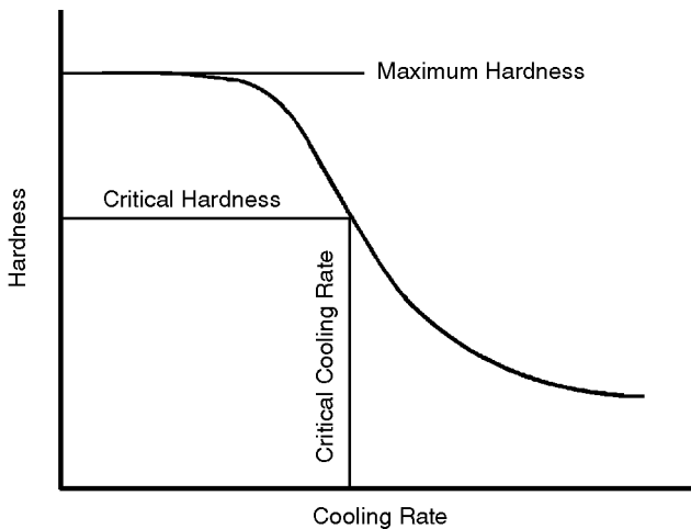
Figure 3.4 Hardness characterization curve for hardness control
