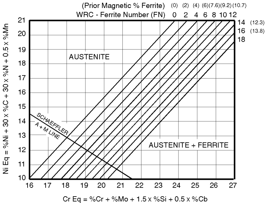
Figure 6.3 Delong diagram
