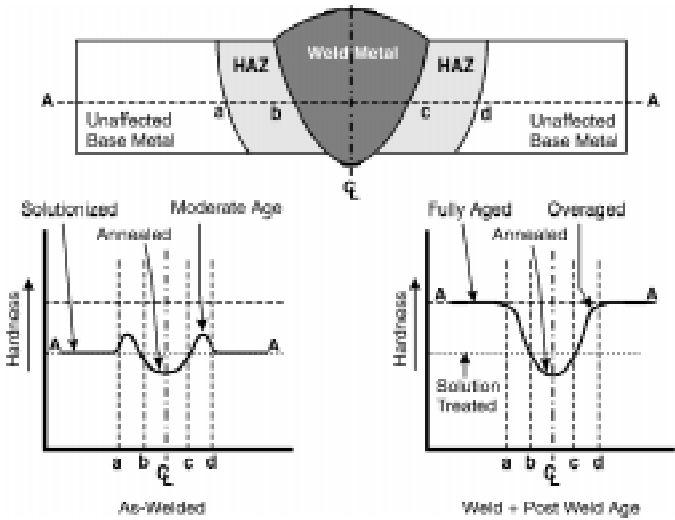
Figure 2.7(d) Hardness changes in solution treated alloys (high heat input weld)
