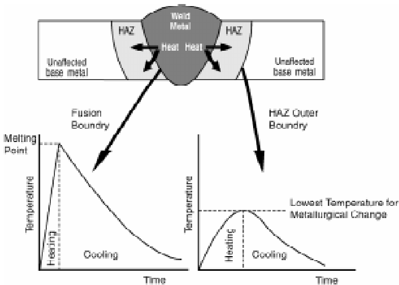
Figure 2.1 Thermal cycles in weld zones
