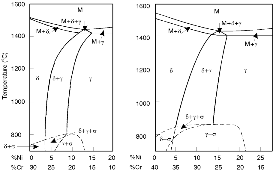
Figure 6.5 Pseudo binary phase diagrams for constant iron content
