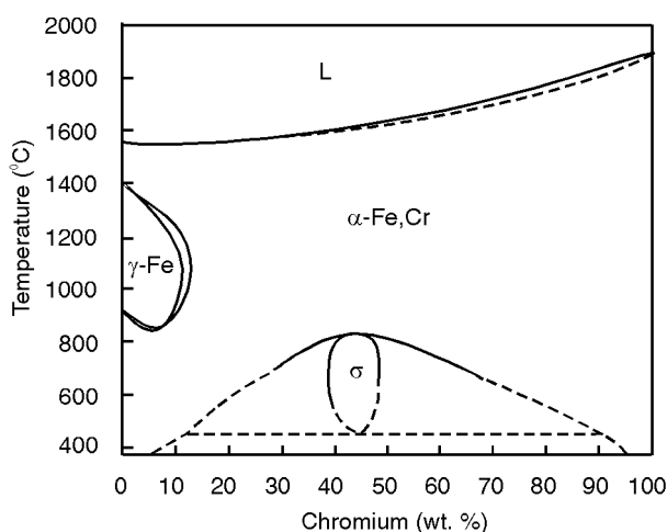
Figure 6.1 Fe-Cr phase diagram showing gamma ( \gamma ) loop
