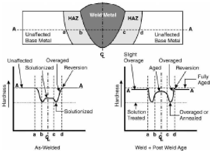
Figure 2.7(a) Hardness changes in fully age hardened alloys (low heat input weld)
