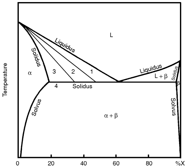
Figure 3.2 Solidification zones according to Borland
