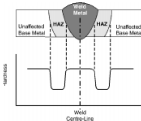
Figure 2.3 HAZ hardness in work hardened metals
