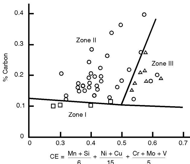
Figure 3.5 Classification zones of steels according to hardening characteristics
