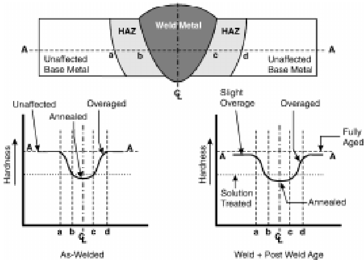
Figure 2.7(b) Hardness changes in fully age hardened alloys (high heat input weld )
