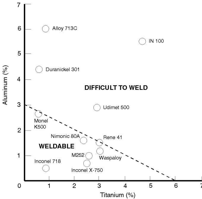
Figure 8.1 Weldability of age hardening nickel alloys
