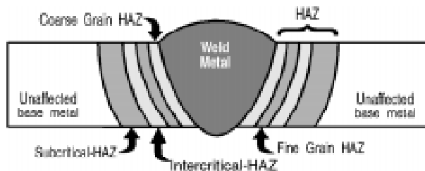
Figure 2.9 Metallurgical designations in heat affected zones
