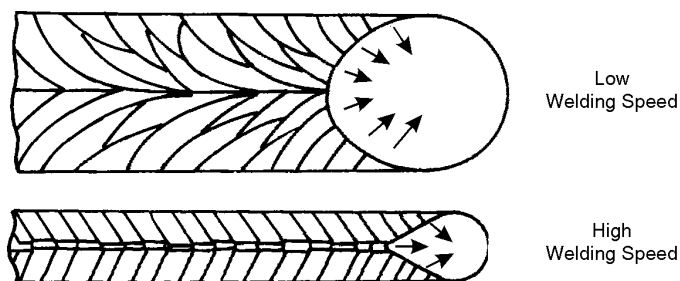
Figure 4.5 Weld metal solidification patterns at low and high welding speeds
