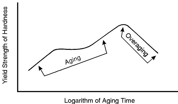
Figure 2.6 Typical strength changes during aging
