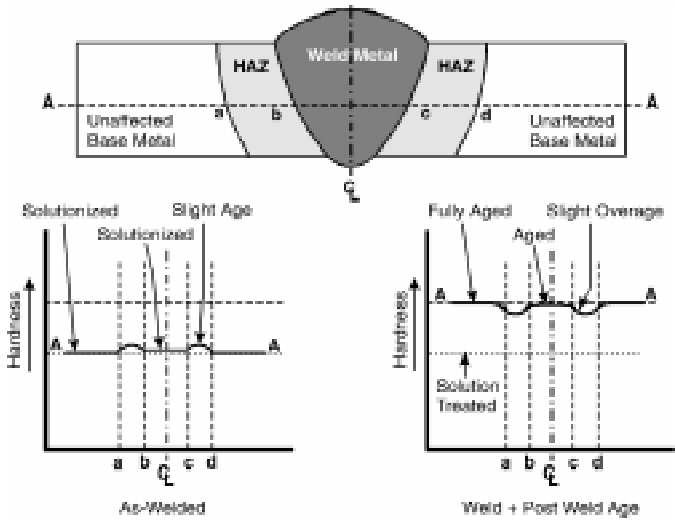
Figure 2.7(c) Hardness changes in solution treated alloys (low heat input weld)
