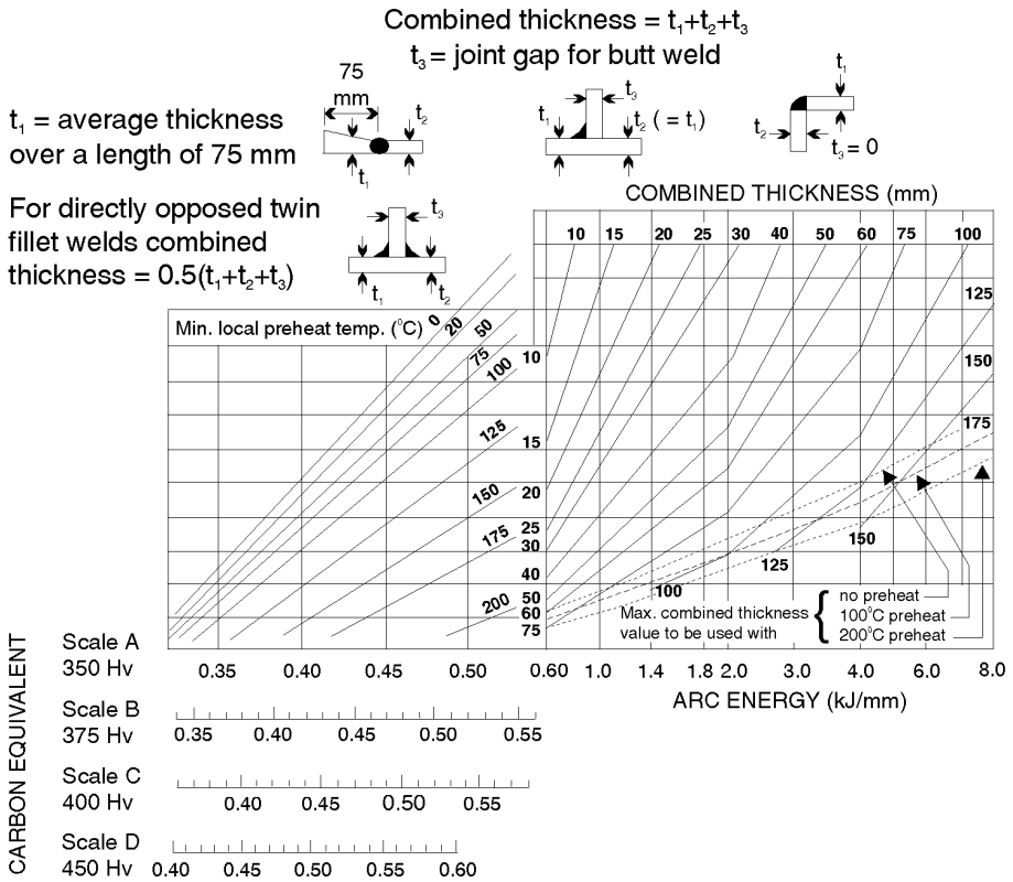
Figure 4.4 Nomogram for procedure control
