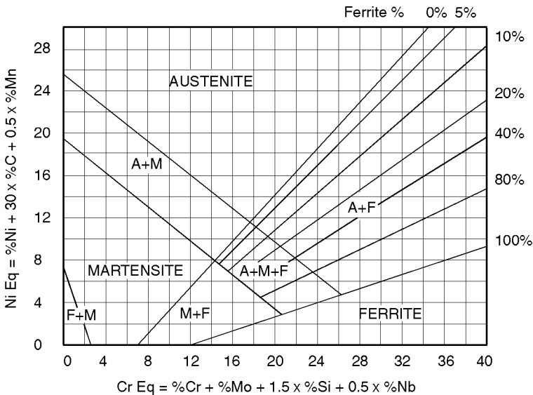
Figure 6.2 Schaeffler diagram
