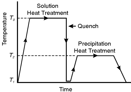
Figure 2.5 Typical age hardening heat treatment
