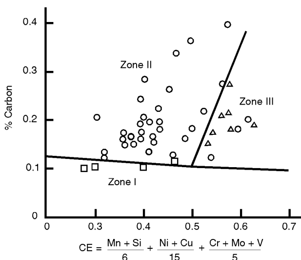
Figure 4.3 Classification zones of steels according to hardenability characteristics
