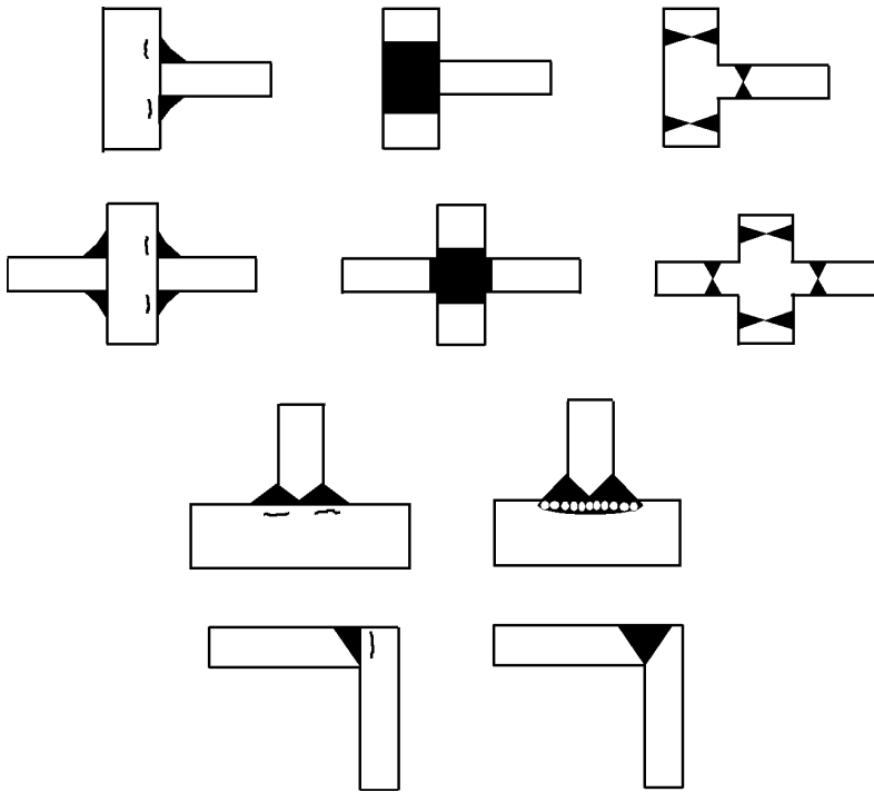
Figure 4.1 Location of lamellar tears and joint redesign for avoidance
