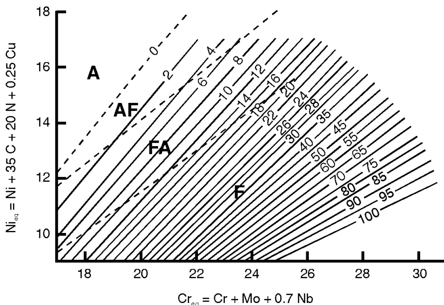
Figure 6.4 WRC - 1992 Constitution diagram for stainless steel weld metal
