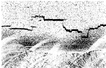
Figure 3.7 Lamellar tears
