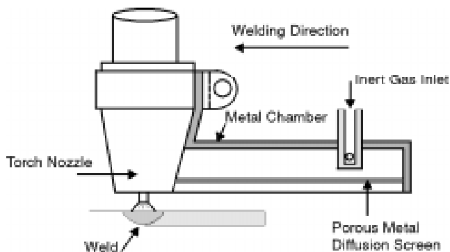
Figure 9.1 Trailing gas shielding system for welding reactive alloys
