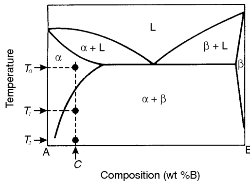
Figure 2.4 Binary phase diagram
