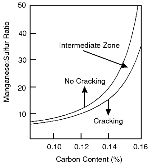
Figure 4.6 The effects of Mn/S ratio and carbon content on weld metal hot cracking in C-Mn steels
