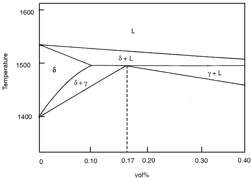
Figure 4.7 Peritectic reaction involving ferrite and austenite
