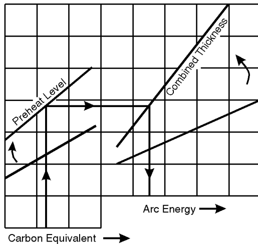
Figure 3.6 Generic nomogram for procedure control of HAZ hardness
