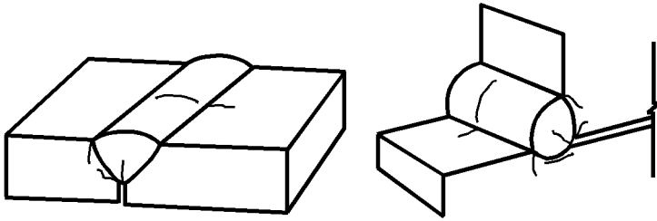
Figure 4.2 Location of hydrogen assisted cracks in weld zones
