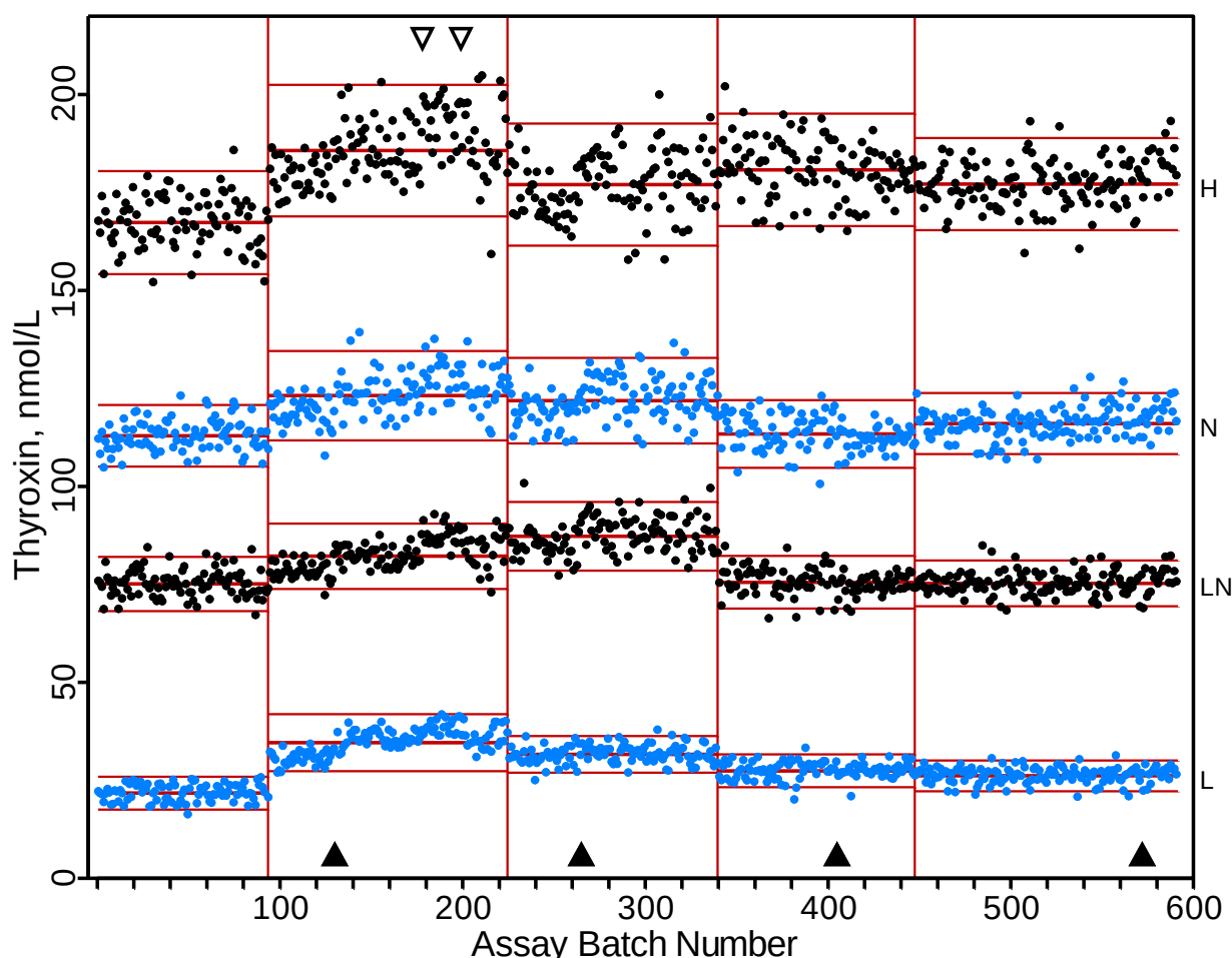
Figure A3. Levey-Jennings Plot Example 3, Thyroxine (T4). Modified from Figure 1 in William A. Sadler, Murray H. Smith, Lynda M. Murray, and John G. Turner. A pragmatic approach to estimating total analytical error of immunoassays. Clinical Chemistry 1997; v. 43, p.608-614 (with permission from the American Association for Clinical Chemistry). 7
