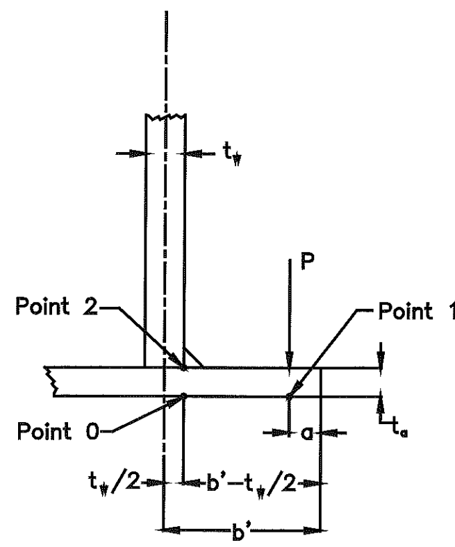
Lower Chord of a Box Girder Figure 3.3.2.6-4
