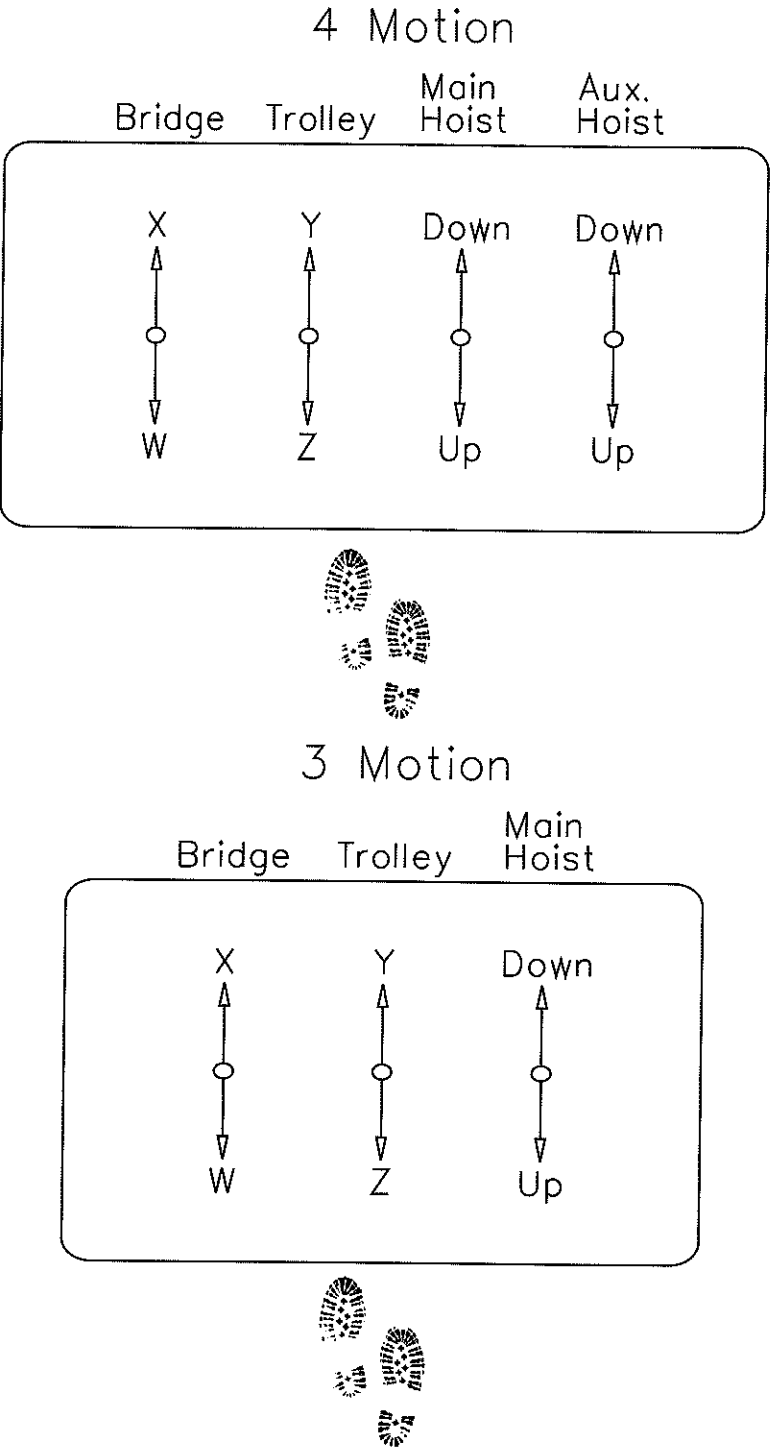
FIGURE 5.15.6 RADIO CONTROL TRANSMITTER LEVER ARRANGEMENT
