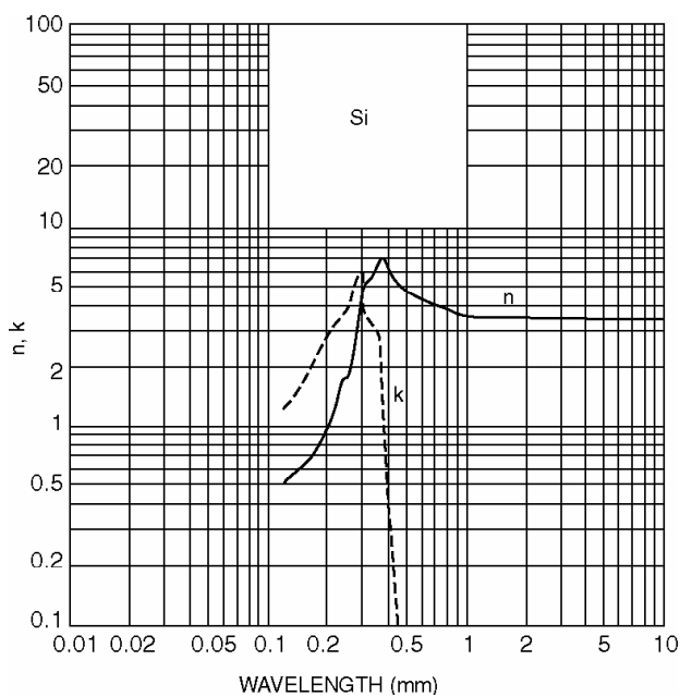
Figure 4.2.19 Real (n) and imaginary (k) part of the index of refraction for silicon.
