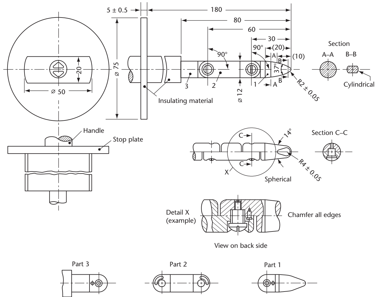
Figure 1 Articulated probe (See Clauses 7.1 and 7.2 .)
