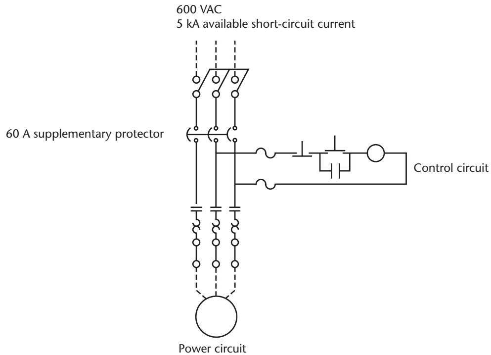
Figure A.4 Motor branch circuit — Supplementary protector misapplication
