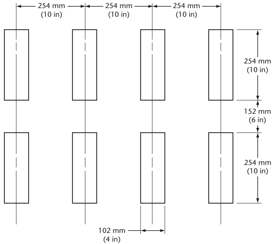
Figure 2 Location of applicators for crushing resistance test (See Clause 19.11.1. )
