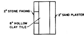
FIG. 27-OUTDOOR WALL
