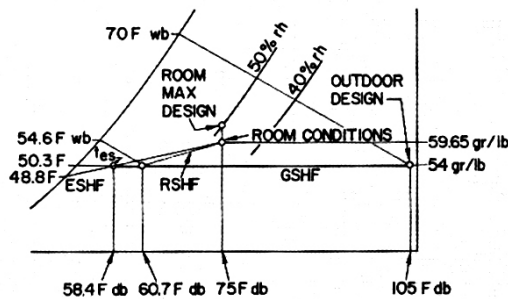
FIG. 53- SENSIBLE COOLING
