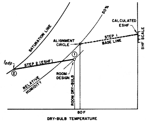
PSYCHROMETRIC CHART
