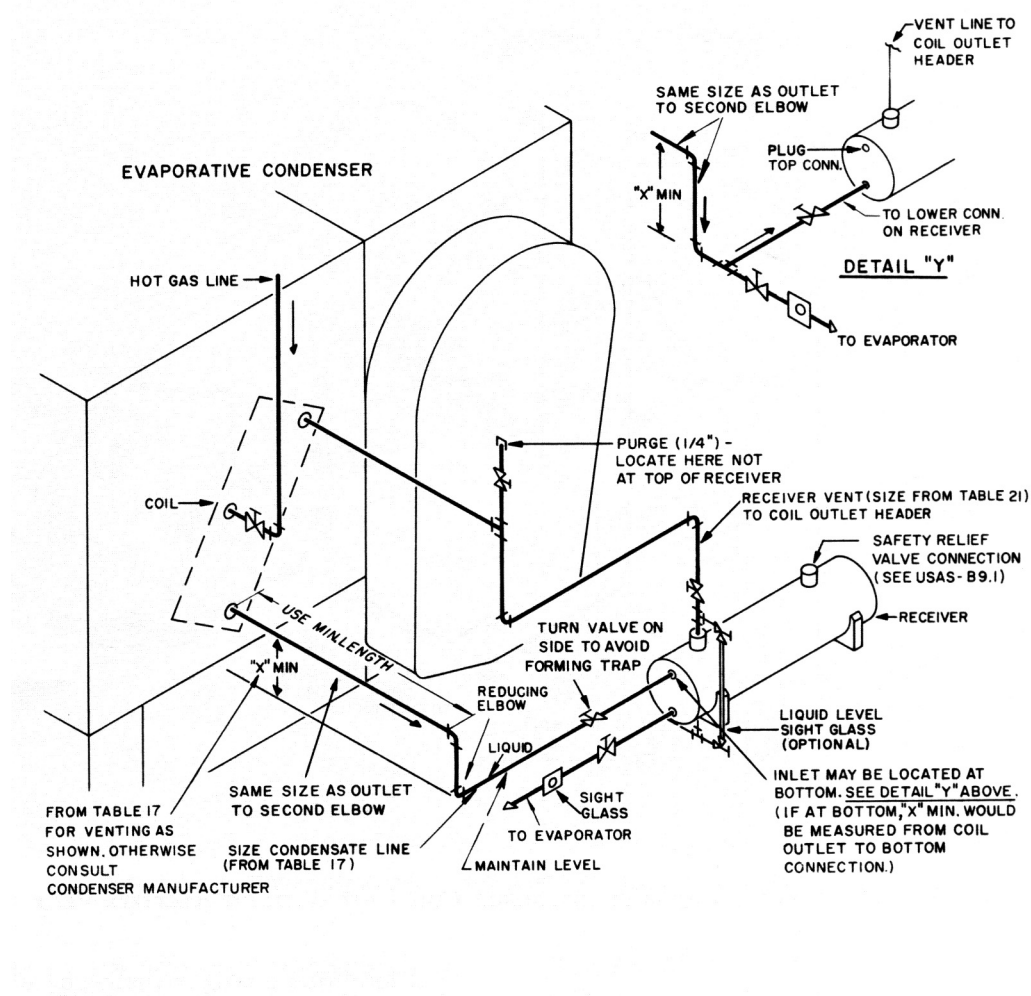
FIG. 71 — HOT GAS AND LIQUID PIPING, SINGLE COIL UNIT WITH RECEIVER VENT
