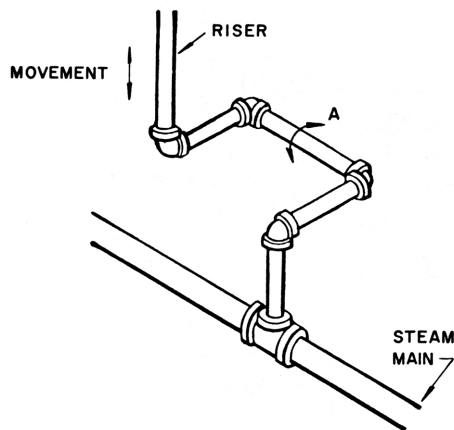
FIG. 114 — RISER CONNECTED TO ALLOW FOR EXPANSION
