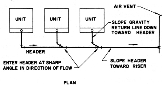
FIG.49 -AIR WASHER RTURN CONNECTIONS AT THE SAME LEVEL
