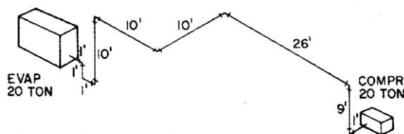
FIG. 58A – SUCTION LINE LAYOUT
