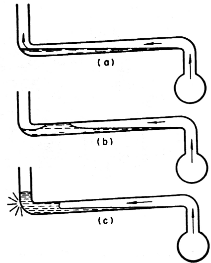
FIG. 112 — WATER HAMMER
