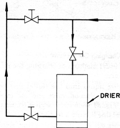
FIG. 81 — THREE-VALVE BYPASS FOR REFRIGERANT DRIER
