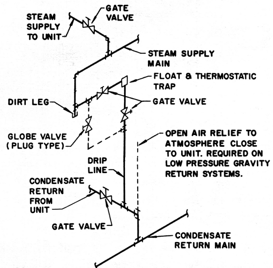
FIG. 124 — VACUUM SYSTEM STEAM COIL PIPING
