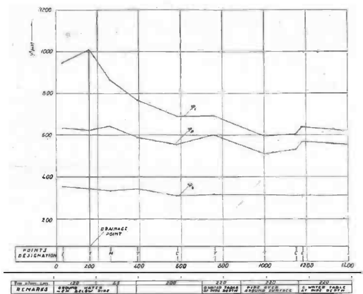
Figure 6.6 On ( \phi_i ), off ( \phi_o ) and natural ( \phi_n ) potential profiles and soil resistivity along the line. (Unz, M., Corrosion , 16, 289–297, 1960.)
