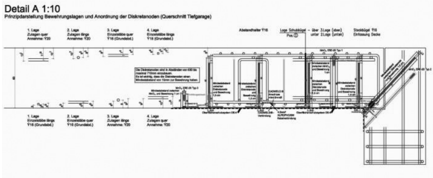
Figure 12.7 Installation of discrete anodes in hammer-drilled holes in the ceiling and adjacent bored pile walls.
