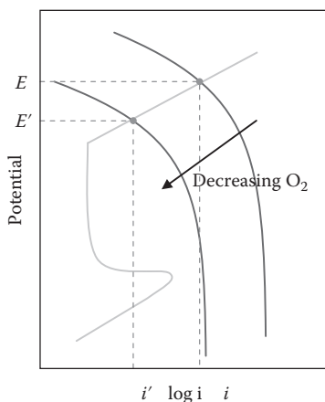
Figure 6.2 Carbonation schematic Evans diagram.
