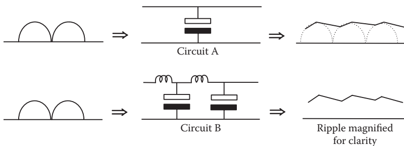
Figure 10.2 Smoothing circuits with results.
