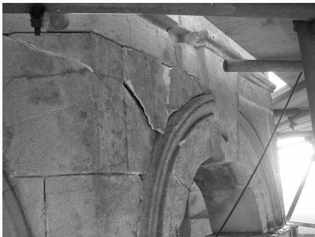
Figure 2.4 Damage to stonework at Great Witley church, Worcester, due to corroding cramps.
