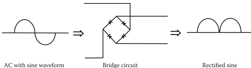
Figure 10.1 Full-wave rectification using a bridge circuit.
