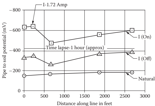
Figure 6.8 Potential profile. (Deskins, R. L., Mater. Protect. , 5, 35, 1966.)
