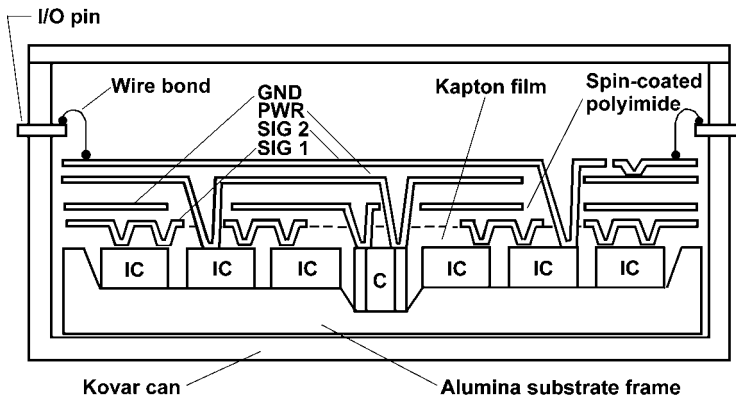
Figure 4.15. Cross-section of a chips first HDI assembly using polyimide dielectric.
