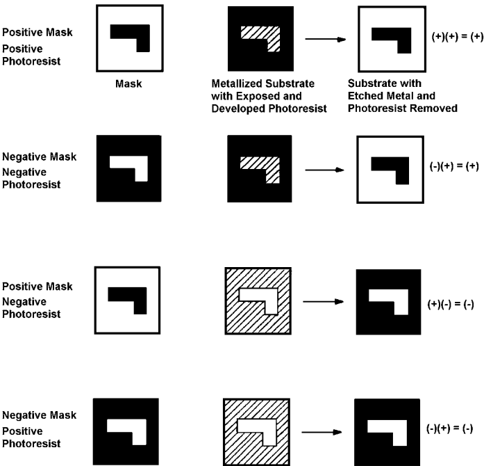
Figure 4.44. Mask/photoresist combinations.
