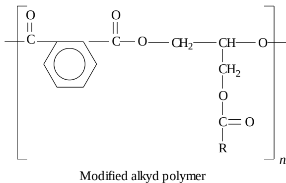
Figure 2.4. Steps in the formation of a modified alkyd polymer.
