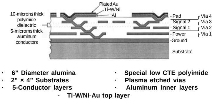
Figure 4.13. Cross-section of MCM-D interconnect substrate (chips last) showing polyimide interlayer dielectric.
